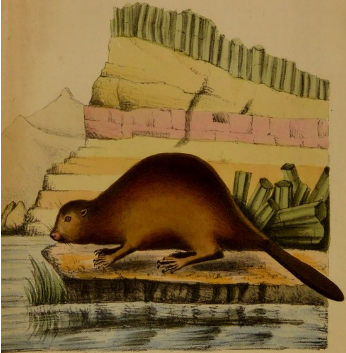
Castor fiber.
