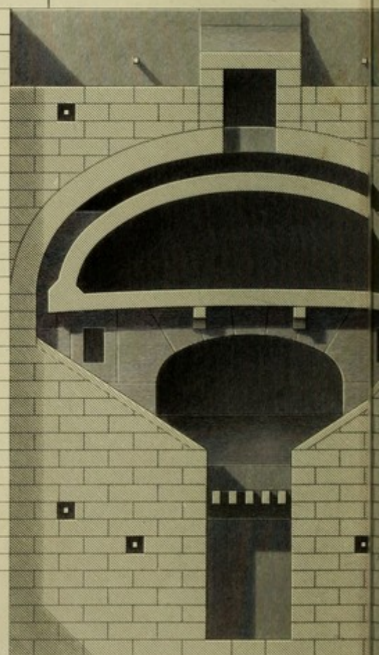
Transverse Section through B.
