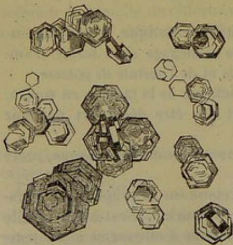
Fig. 84. — Cystine.
