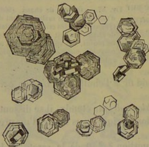
Fig. 88. — Cystine.
