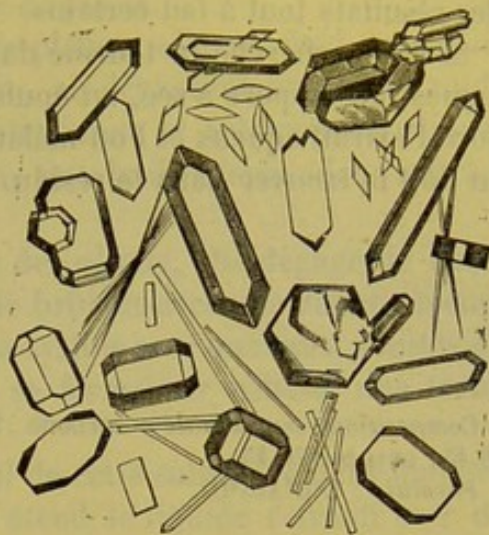
Fig. 85. — Taurine.
