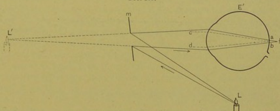
Employment of plane mirror in emmetropia.
