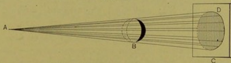
Shadow of sphere on a plane surface.
