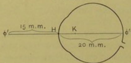
Reduced eye.
