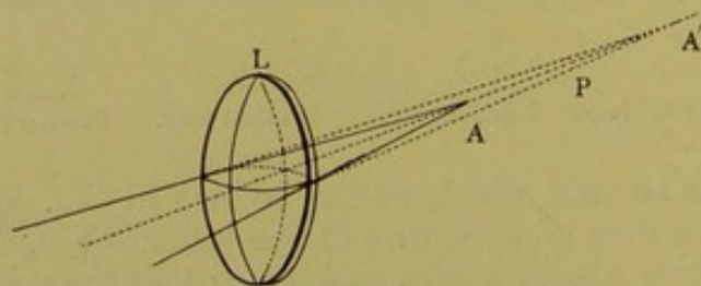
Negative focus from a bi-convex spherical lens.
