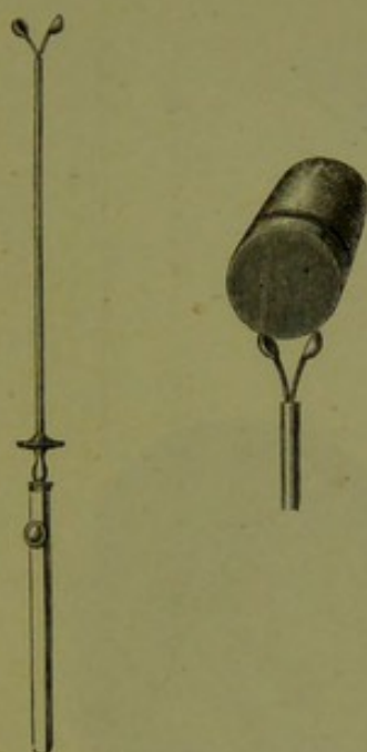
LECOMTE-LÜER'S bullet detector.
