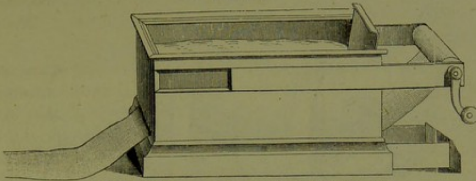
WYWODZOFF'S machine for plaster of Paris bandages.
