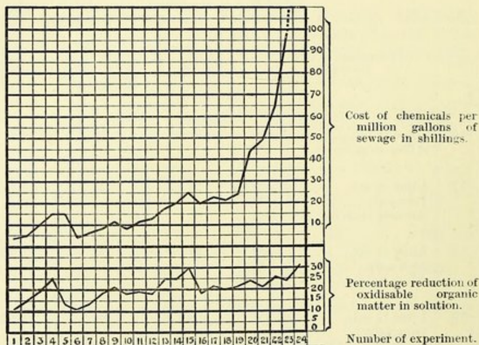
Fig. 7.—Dibdin's experiments on London sewage.
