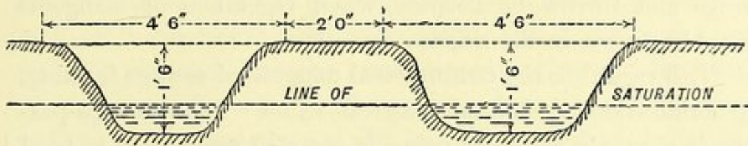
Fig. 13.—Ridge and furrow filtration areas.
