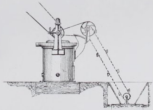
SIDE ELEVATION SHOWING ELEVATOR.
