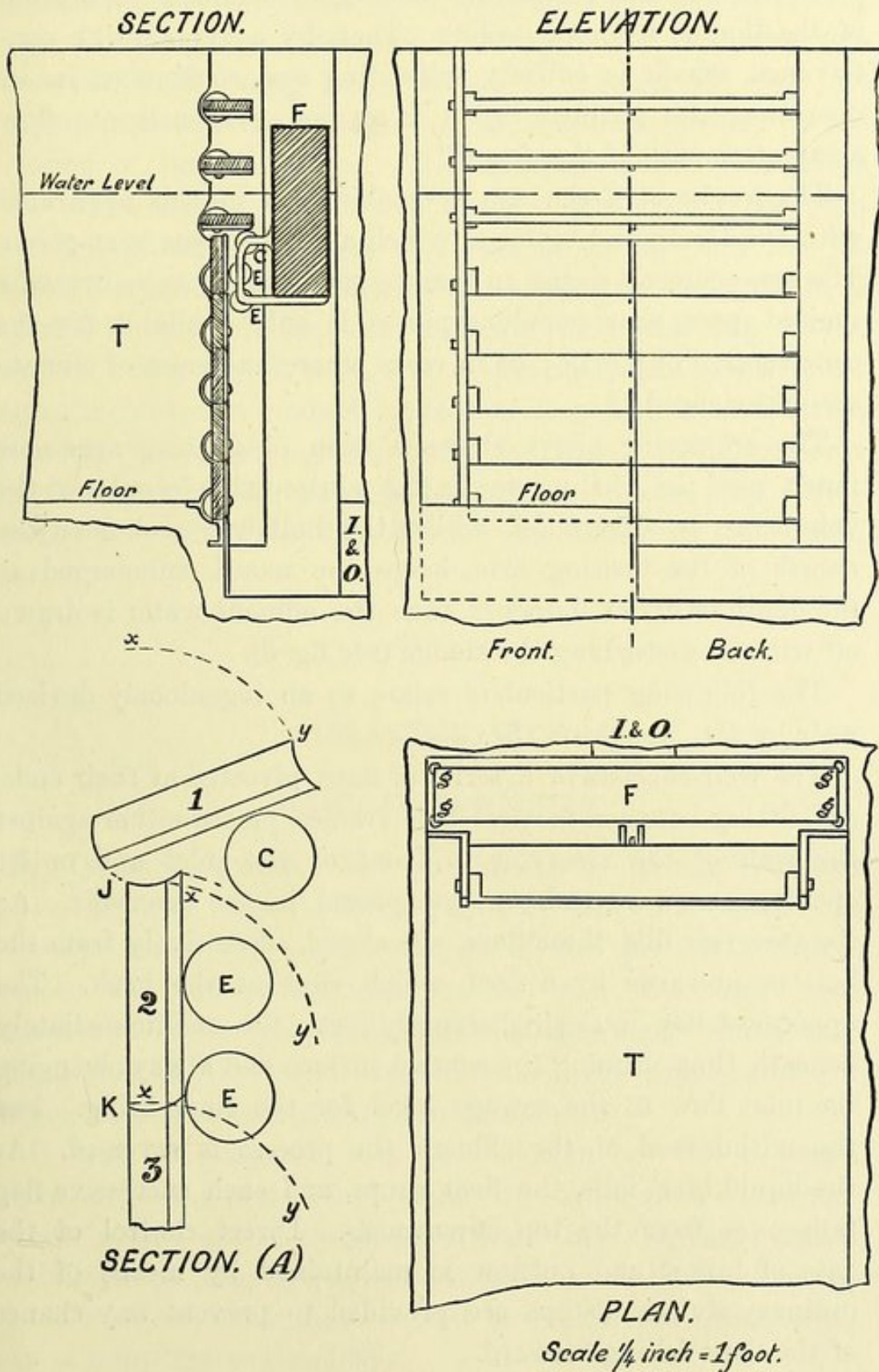
Fig. 4.—Weir designed by Mr. Houghton.
