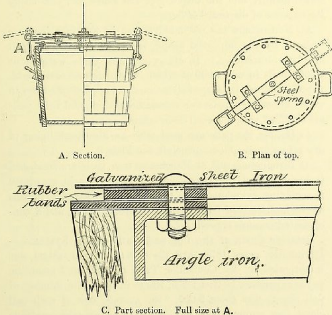
Fig. 1.—The Rochdale excreta pail—Scale \frac{1}{8} th full size.
