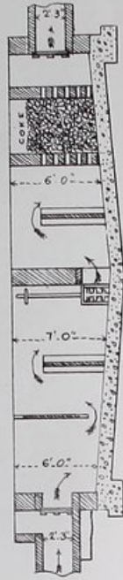
SECTION OF STRAINING TANK
