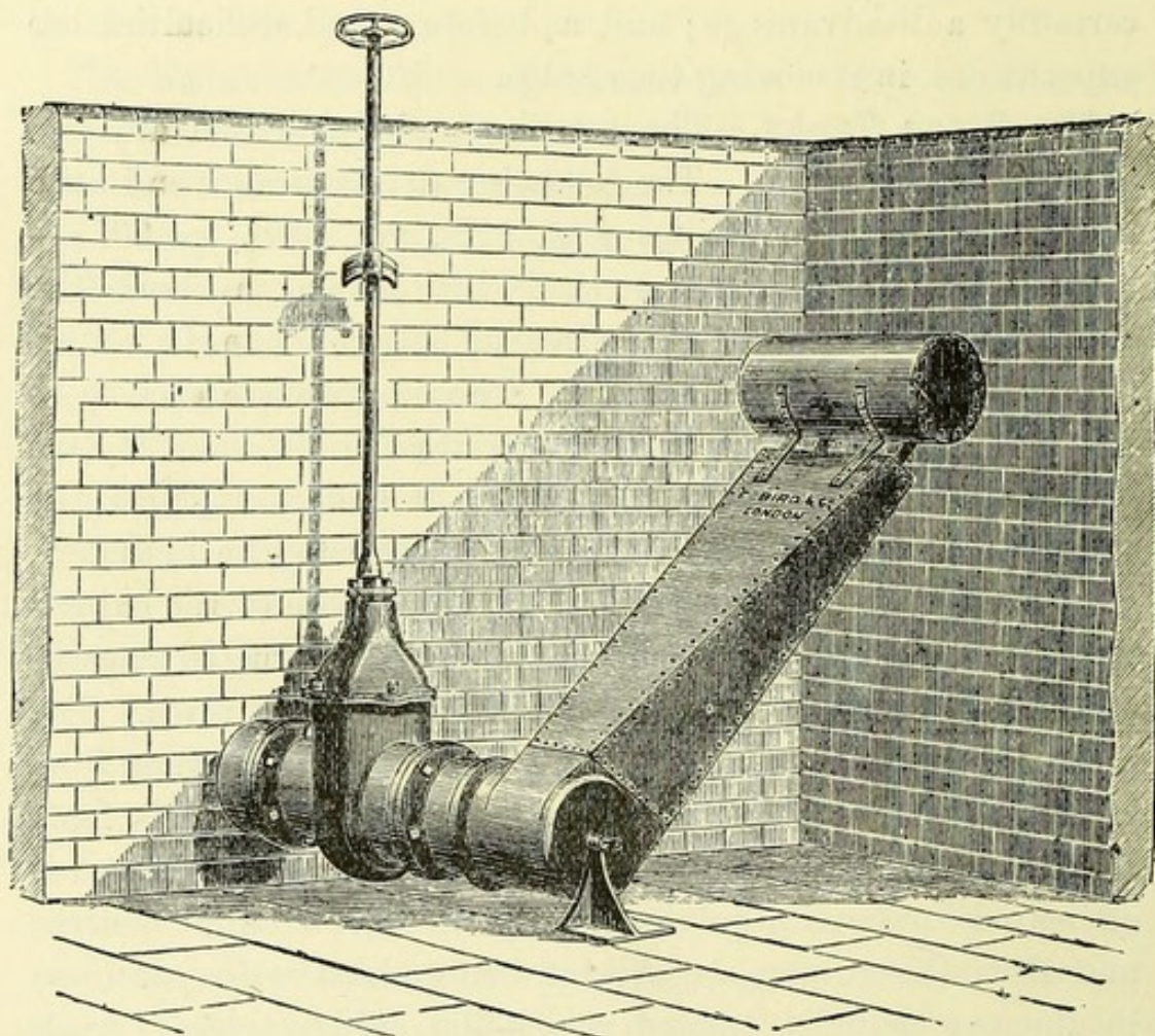
Fig. 3.—Floating arm used in settling tanks.
