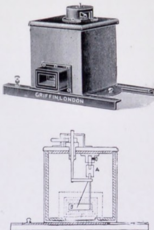
FIG. 9.—GAMMA-RAY ELECTROSCOPE.
