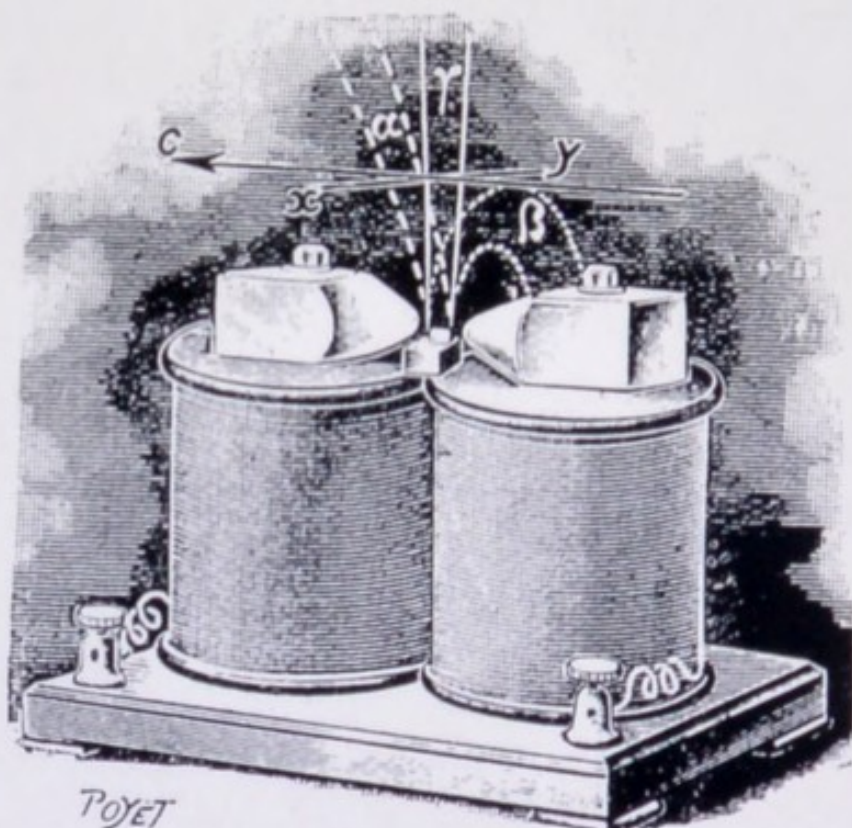
FIG. 5.—MAGNETIC DEFLECTION.
