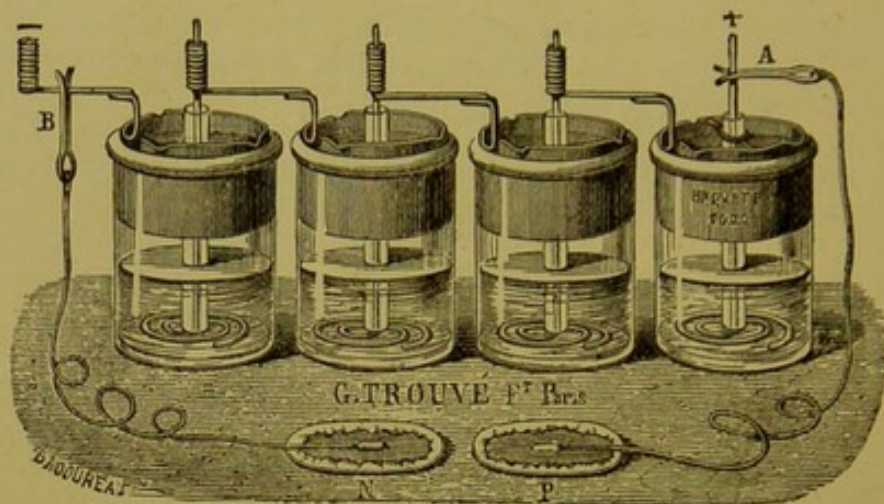
Four Callaud-Trouvé gravitation elements arranged in series.
