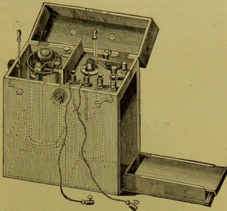
Stöhrer's single celled induction apparatus. Size: 10\frac{1}{2} inches long, 5 wide, 10\frac{1}{2} deep.
