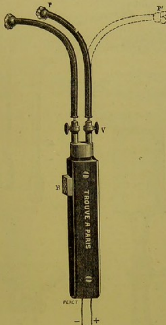
Trouvé's bipolar electrode.
