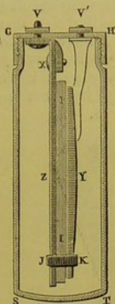
GAIFFE'S CHLORIDE OF SILVER ELEMENT.
