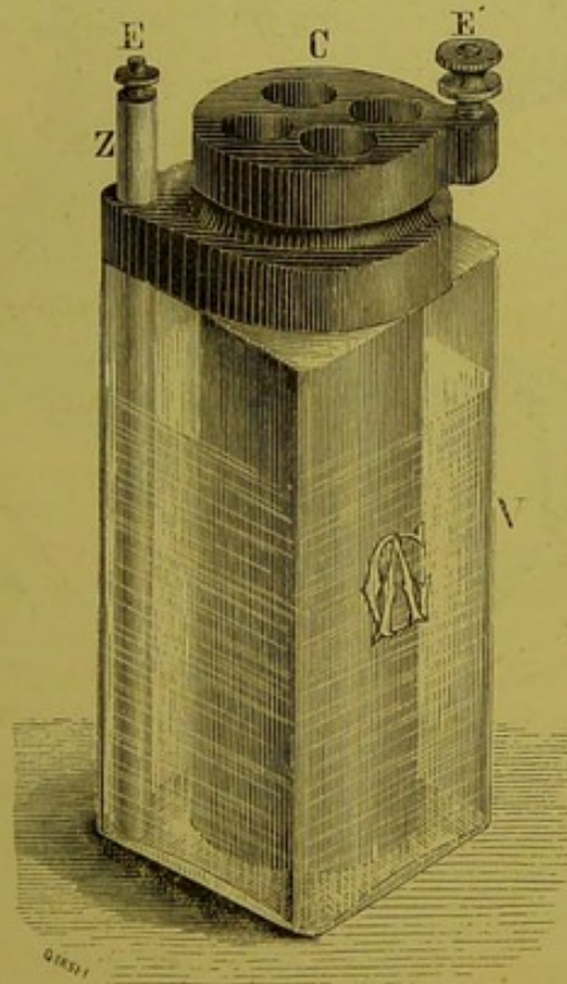
Gaiffe's peroxide of manganese element, see page 142.
