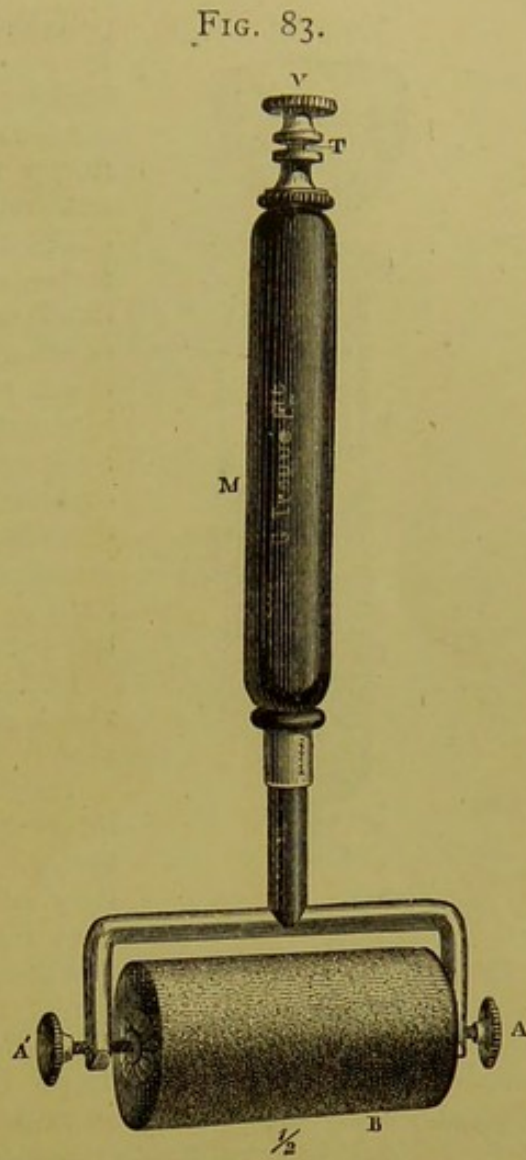
Trouvé's roller electrode.
