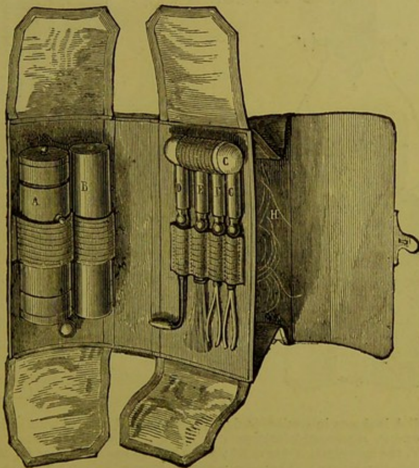
Trouvé's pocket faradic apparatus.
