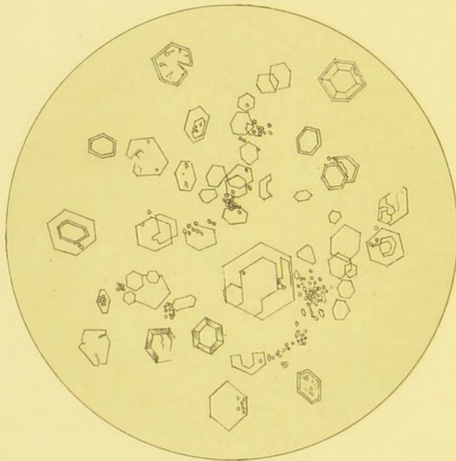
FIG. 84.—Cystin.
