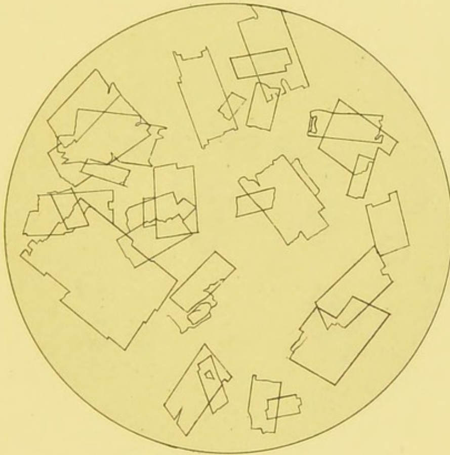
FIG. 85.—Cholesterin.
