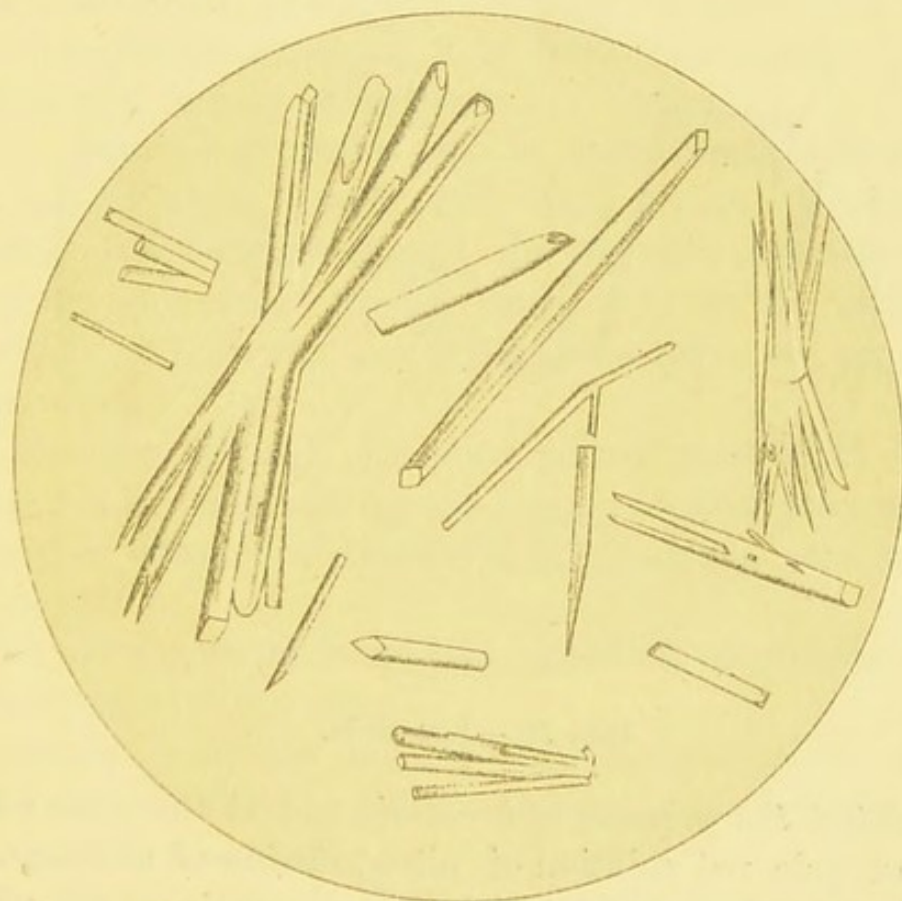
FIG. 77.—Hippuric acid.
