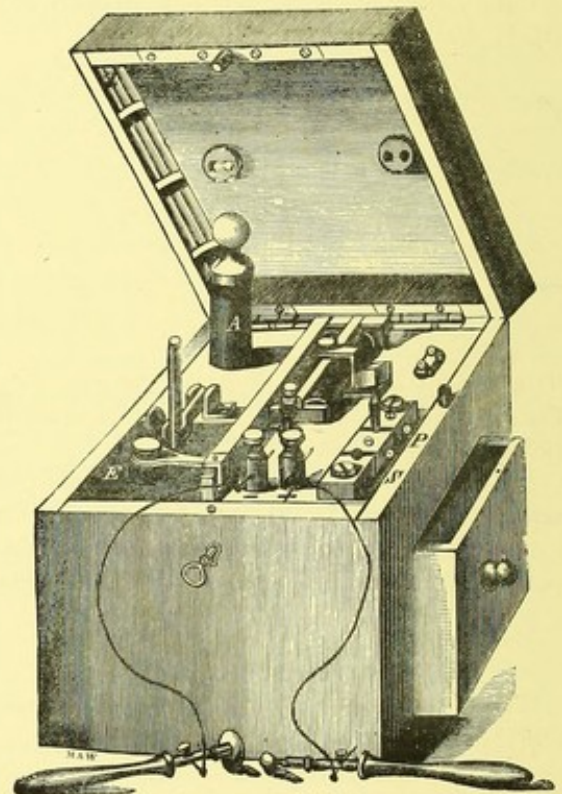
SPAMER'S INDUCED CURRENT, SINGLE CELL.
