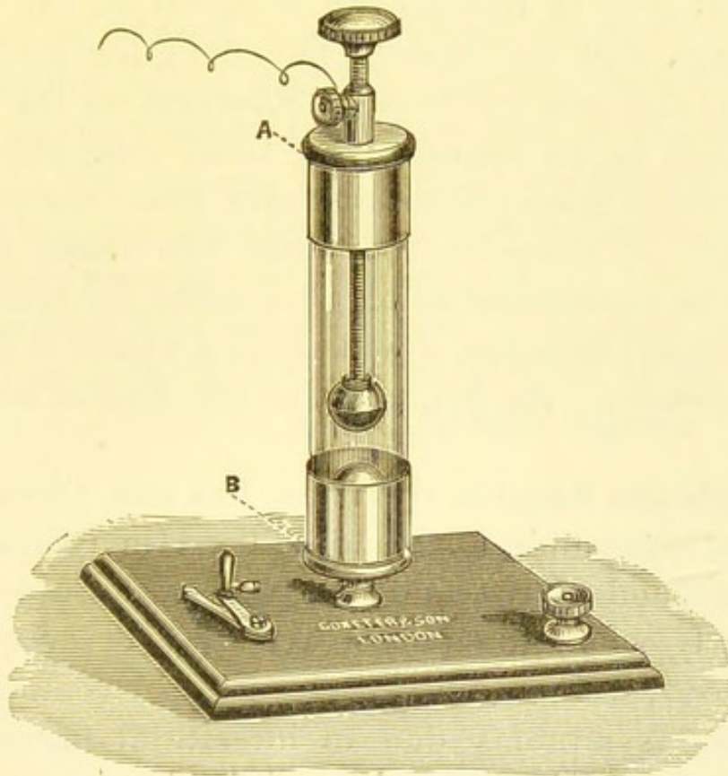
FIG. 70.—Water rheostat to be introduced in the circuit at an indifferent point for regulating the strength of the current (Coxeter).
