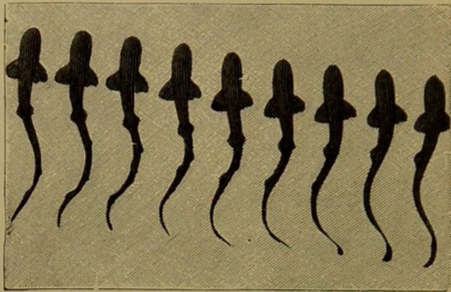
FIG. 191.—Dog-fish swimming.
