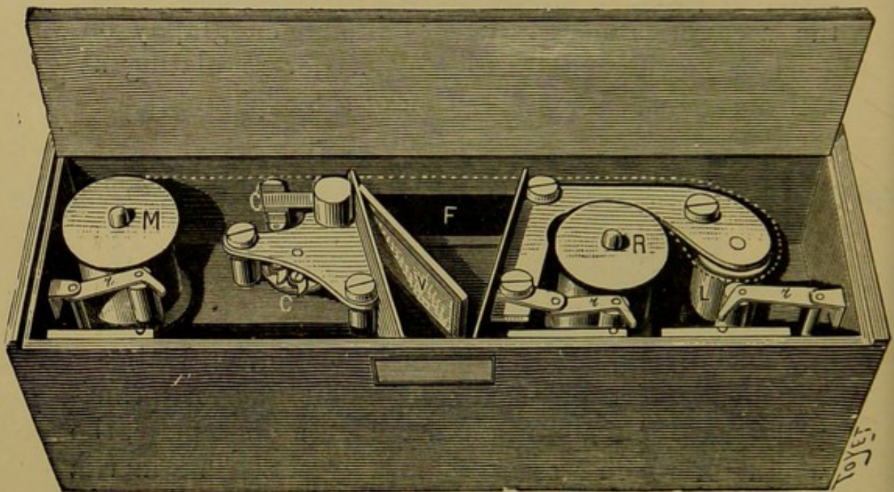
FIG. 80.—Internal structure of the photographic chamber.
