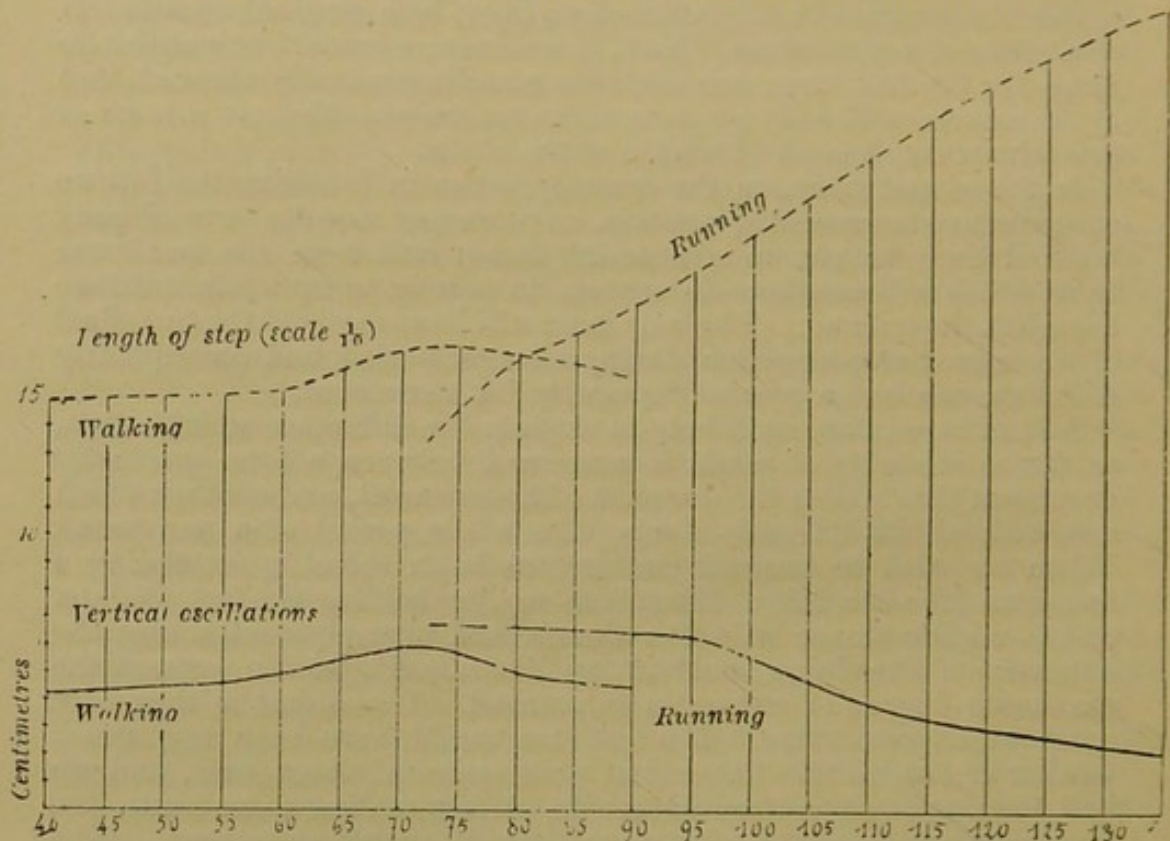
FIG. 108.—Variations in the vertical oscillations of the body in walking and in running. The rate of step varies between 40 and 130 per minute. Comparison between the curve of oscillation and that of the length of stride.
