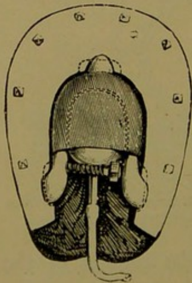
FIG. 6.—Special apparatus for recording the contacts of a horse's feet with the ground; a transmitting tube effects a communication between the air chamber and the chronographic tambour.
