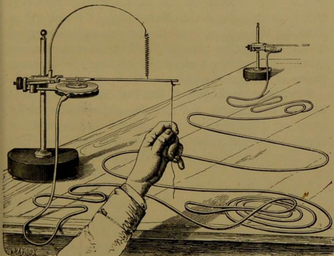
FIG. 2.—Arrangement designed for transmitting a movement to the needle, which records the duration and the phases.
