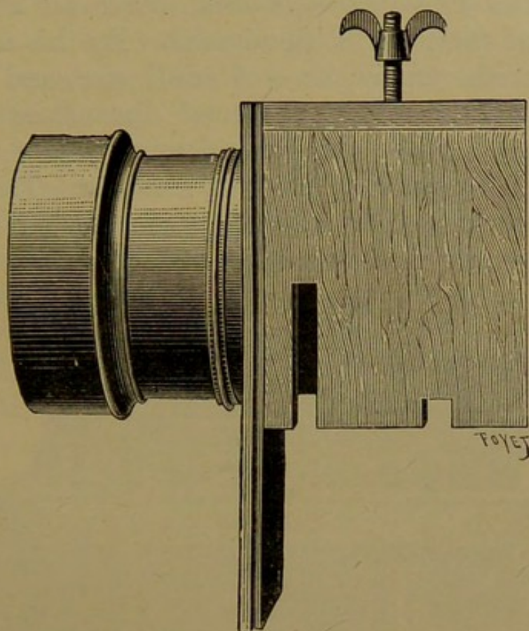
FIG. 46.—Objective mounted in a sliding box. Below can be seen the opening for the passage of the circular diaphragms.
