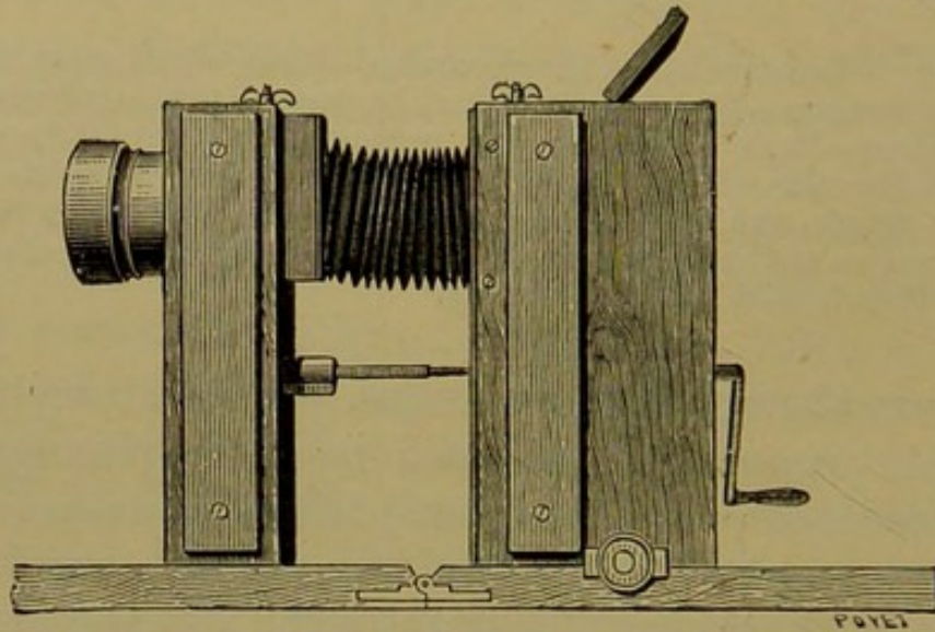
FIG. 45.—Arrangement of an apparatus adapted for all the purposes of chronophotography (scale \frac{1}{10} ).
