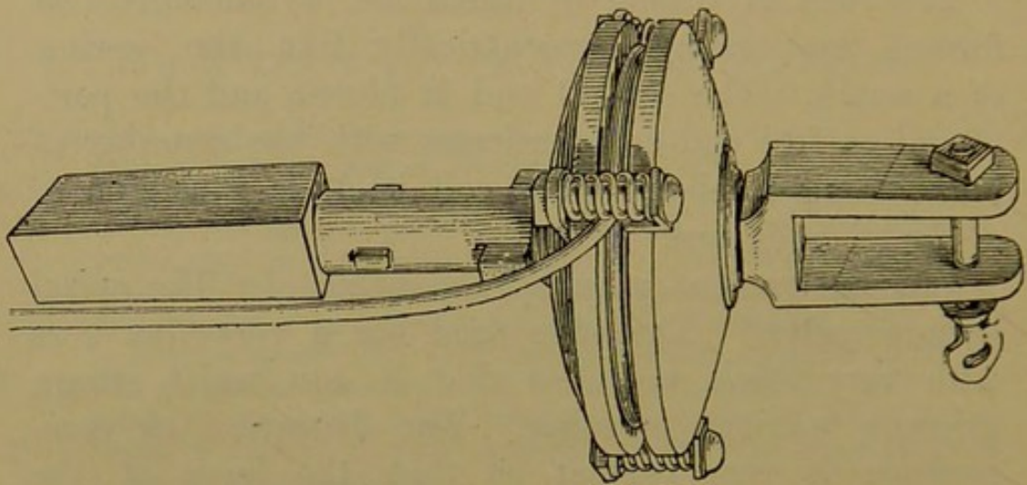
FIG. 99.—Traction dynamograph.
