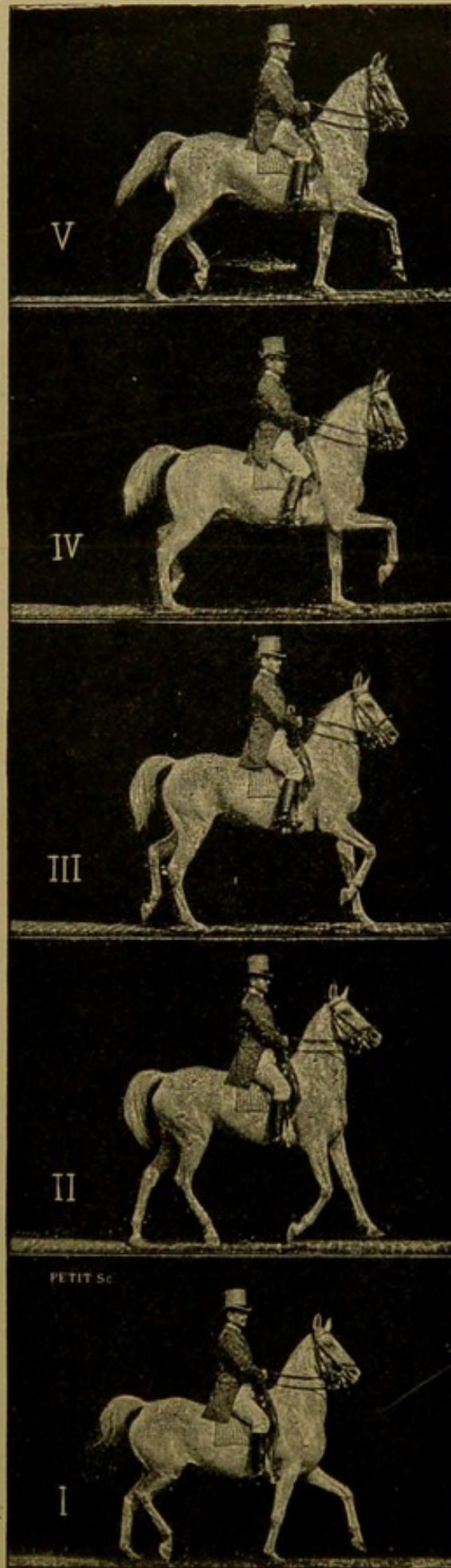
FIG. 131.—Horse walking.
