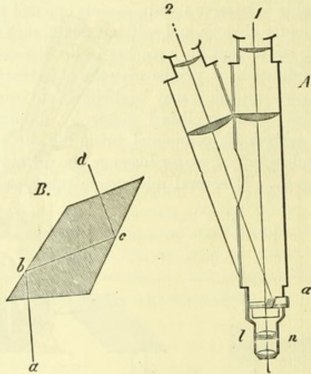
Fig. 42. Wenham's arrangement of the stereoscopic microscope.
