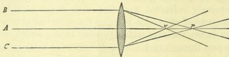
Fig. 13. Chromatic Aberration.
