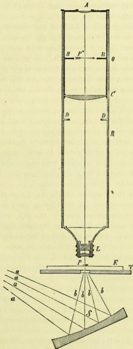
Fig. 17. The compound microscope.
