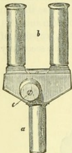
Fig. 44. Hartnack's stereoscopic eye-piece. The two tubes b may be adjusted according to necessity by means of the button c ; a for insertion into the tube of the microscope.
