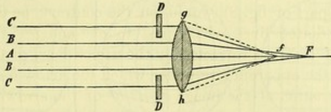
Fig. 9. Spherical Aberration.
