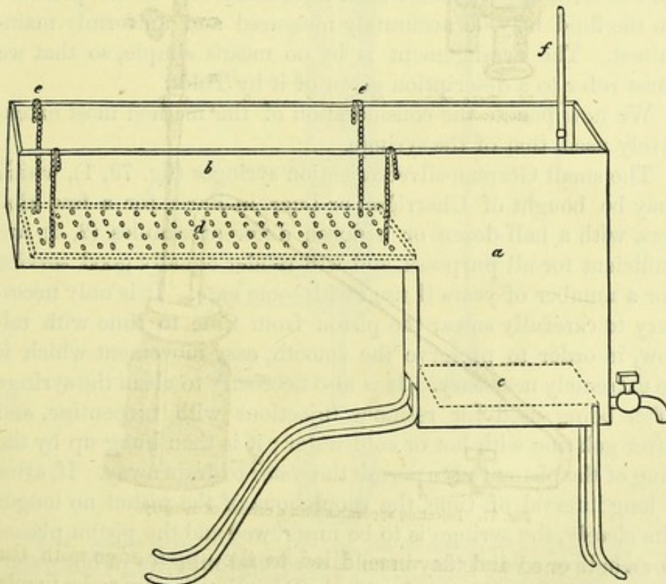
Fig. 78. Harting's injection chest. a chest; c false bottom for the injection bottle; f thermometer; b compartment for the reception of the preparation; d perforated plate, the position of which may be altered by means of the chains e .
