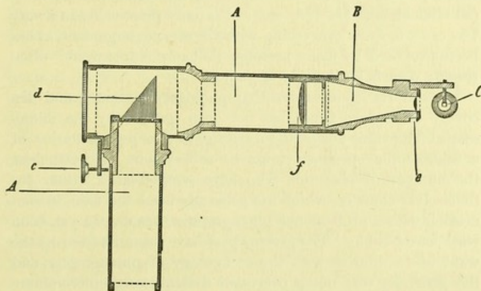
Fig. 36. Camera lucida of Chevallier and Oberhäuser. The piece B is turned 90°.
