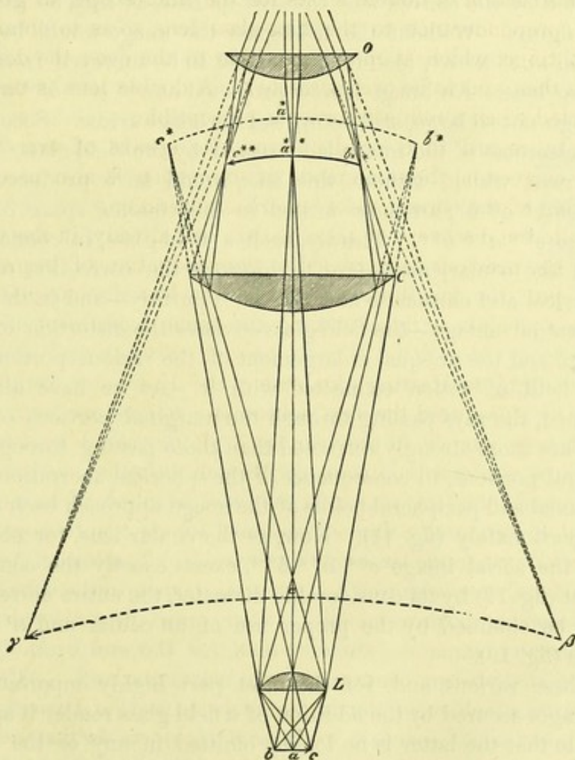
Fig. 15. The compound microscope with a field-glass.
