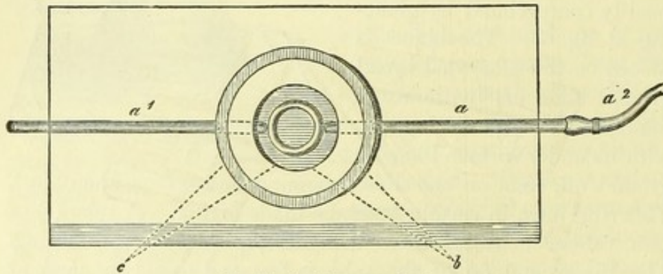
Fig. 65. Stricker's gas-chamber.
