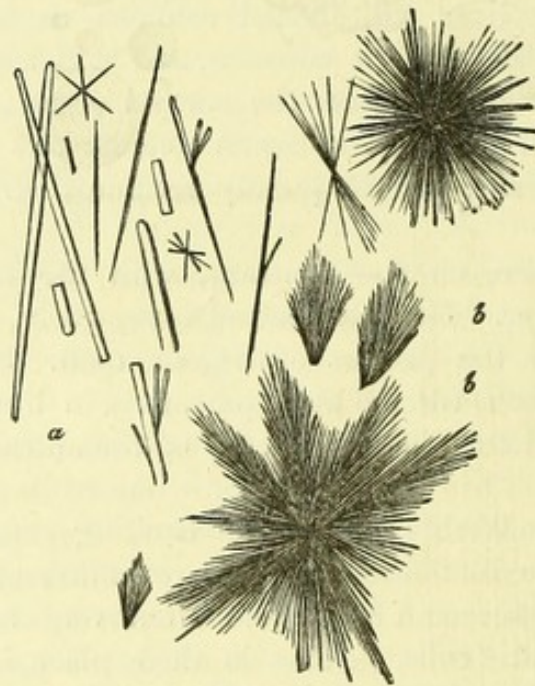
Fig. 257. Crystalline forms of tyrosin.
