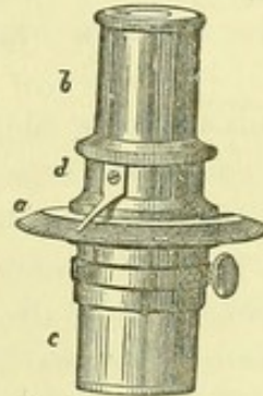
Fig. 47. Hartnack's analyzer, new construction. The eye-piece b c turns in a sheath, which is to be fastened to the microscope by means of the screw at the right; it also has a graduated circle a ; d vernier.
