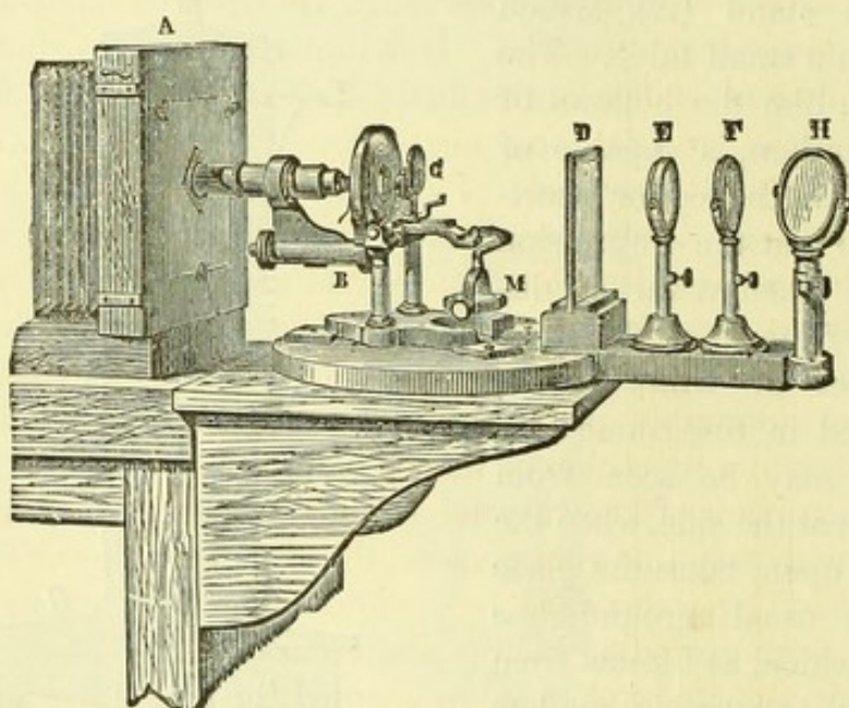
Fig. 39. Horizontal apparatus. A folding camera, B microscope; C achromatic condenser; M the mirror of the microscope turned aside; H the silvered mirror; F the diaphragm; E convex lens; D ground-glass plate.
