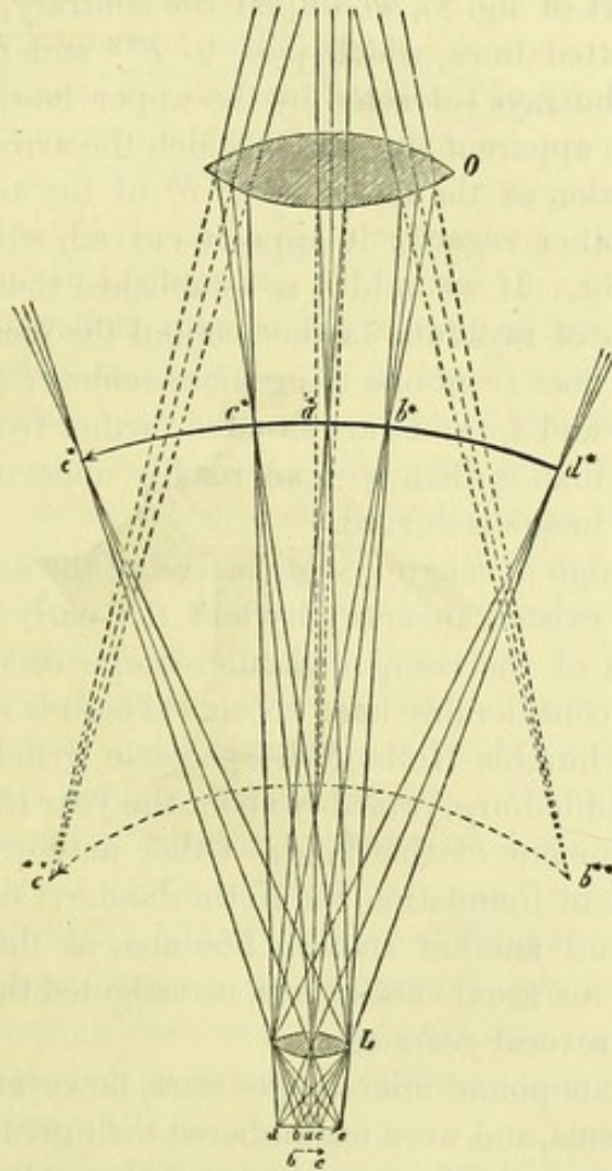
Fig. 8. The compound microscope in simplified form.
