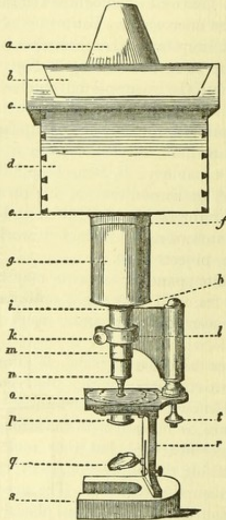
Fig. 37. Gerlach's micro-photographic apparatus: a hollow cone, to be placed on b , the focusing screen; c projection at the upper part of the case d ; e metal ring at its bottom; f metal ring at the upper part of the wooden tube g ; h metal plate at the lower end of the same; i ring at the upper end of the metallic tube; k screw of the metal ring l , which serves to clamp the spring sheath m ; n tube of the microscope with the objectives; o stage; p the metallic cylinder for carrying the diaphragm and illuminating lens; q the mirror; r the metallic bar which supports the stage; s the horse-shoe foot; t the micrometer screw.
