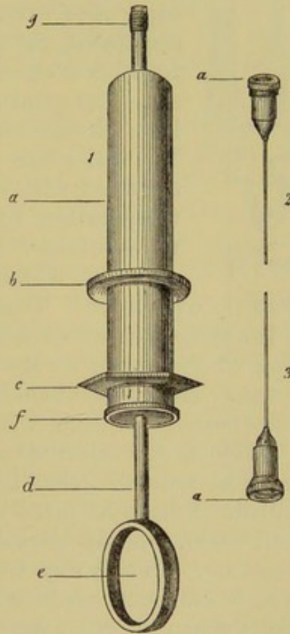
FIG. 93.—Syringe for Injections. 1. a , the tube, with the projecting edges b , and c , (for convenience in holding), and the cap f , which is to be screwed on; d , piston-rod with the ring e ; g , the aperture (mouth-piece) of the syringe, with a silk thread wound round it. 2 and 3. Canules of the finest variety.
