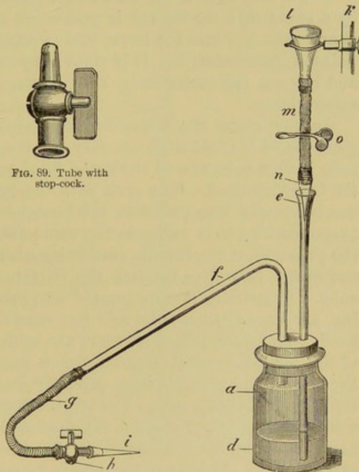
FIG. 90. Injecting apparatus, with a column of mercury.
