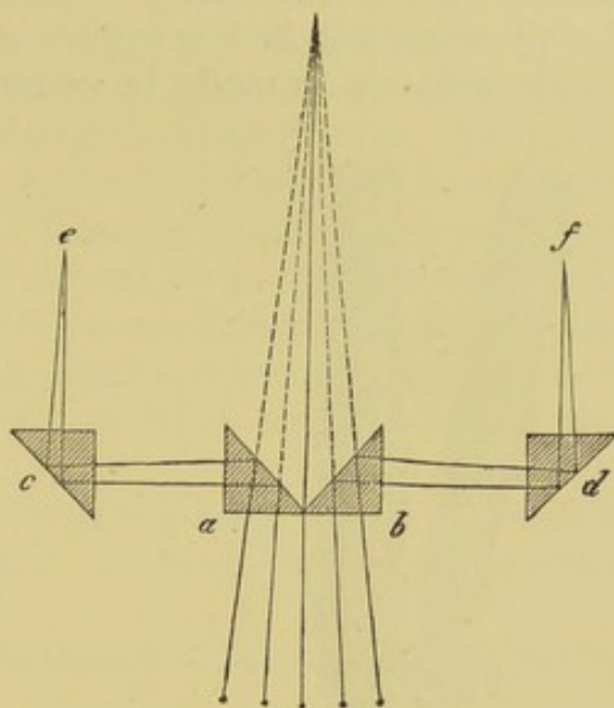
FIG. 53. The prisms in Hartnack's stereoscopic eyepiece.
