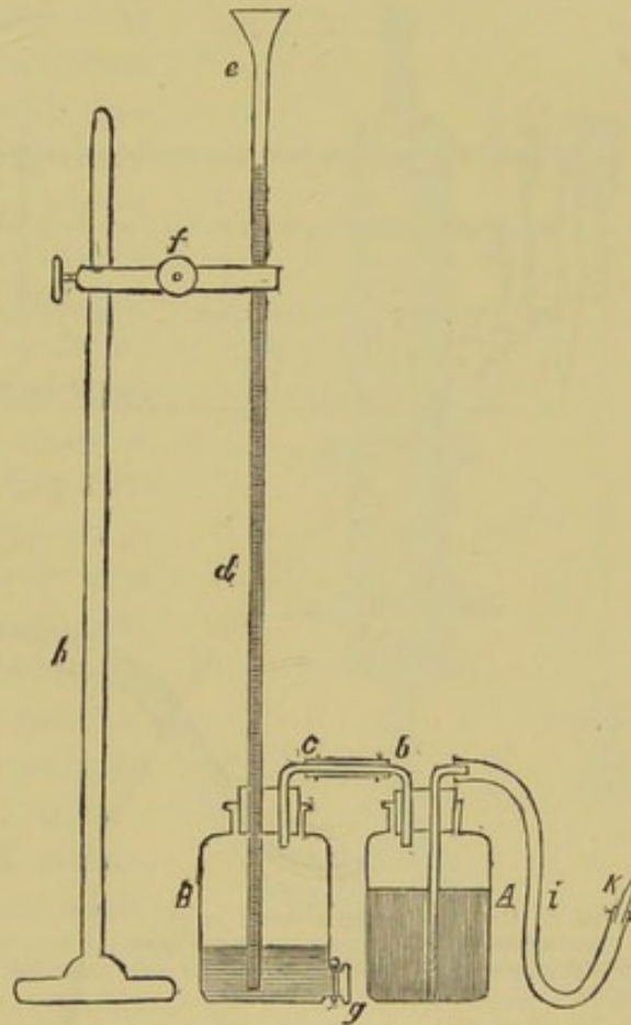
FIG. 91. Apparatus for injection with mercury and compressed air (after Toldt). A , injection bottle; B , air chamber; b , c , glass tubes with connecting rubber tube; d , glass tube for the column of mercury; g , and h , apparatus for securing the tubes; i , rubber tube; k , canule fastened in.
