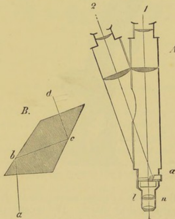
FIG. 49. Wenham's arrangement of the stereoscopic microscope.
