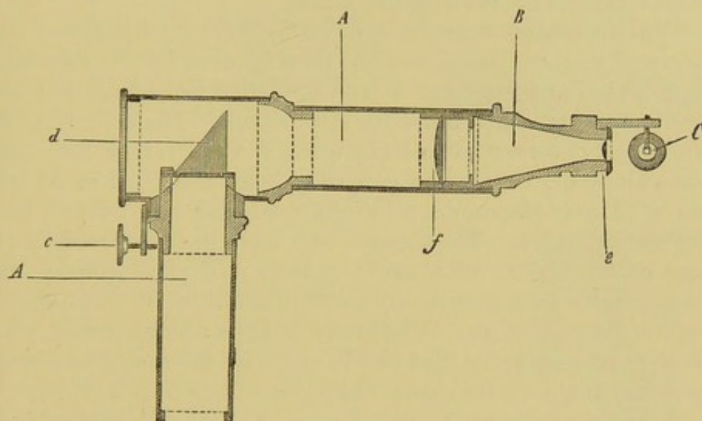
FIG. 43. Camera lucida of Chevalier and Oberhäuser. The piece B is turned 90^\circ .
