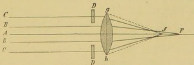
FIG. 9. Spherical aberration.
