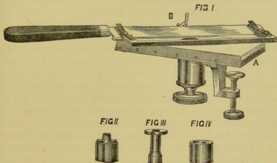
FIG. 83*. Curtis' "section cutter."
