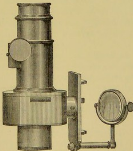
FIG. 57. Complicated spectral eye-piece of Hartnack.
