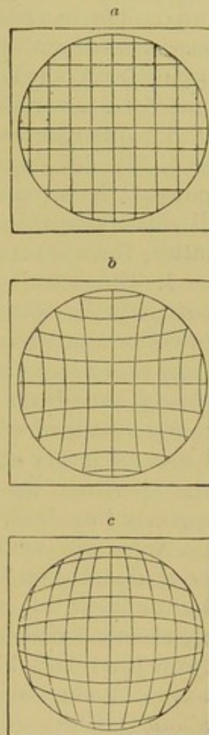
FIG. 58. Quadratic glass micrometer.
