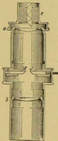
FIG. 56. Simple spectral eye-piece of Merz.
