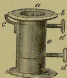
FIG. 83. Schiefferdecker's microtome, about half the actual size.
