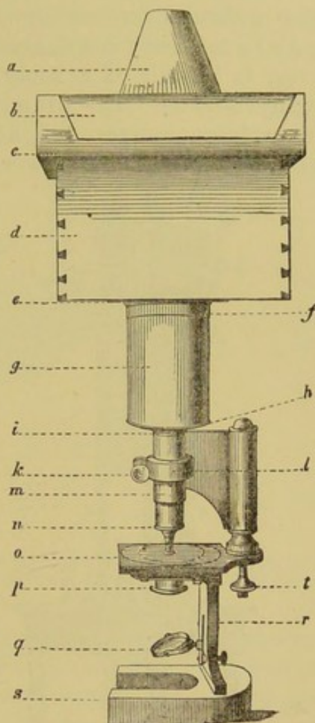
FIG 44. Gerlach's micro-photographic apparatus: a , hollow cone, to be placed on b , the focussing screen; c , projection at the upper part of the case d ; e , metal ring at its bottom; f , metal ring at the upper part of the wooden tube g ; h , metal plate at the lower end of the same; i , ring at the upper end of the metallic tube; k , screw of the metal ring l , which serves to clamp the spring sheath m ; n , tube of the microscope with the objectives; o , stage; p , the metallic cylinder for carrying the diaphragm and illuminating lens; q , the mirror; r , the metallic bar which supports the stage; s , the horseshoe foot; t , the micrometer screw.
