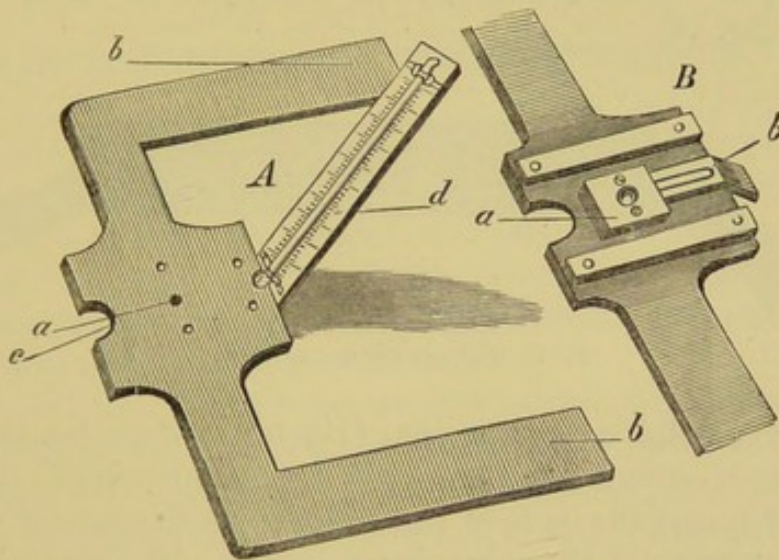
FIG. 77. Schultze's warmable stage.
