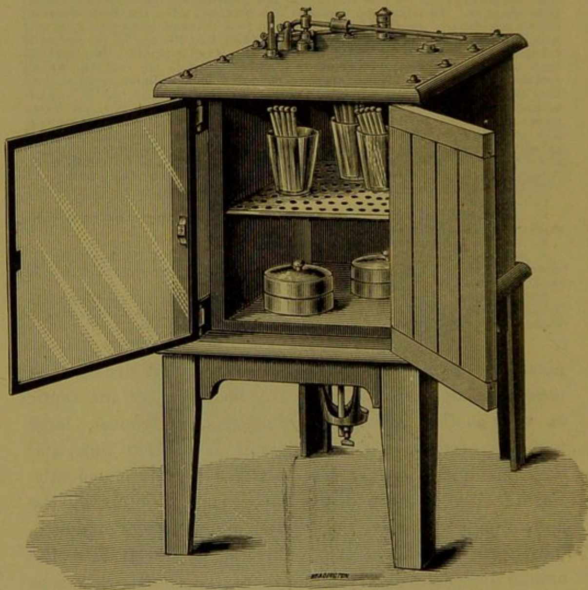
FIG. 2.—HEARSON'S INCUBATOR.
