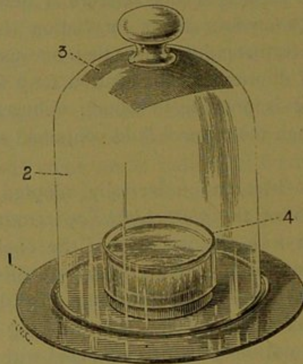
FIG. II.—PLATE-CULTIVATION.
