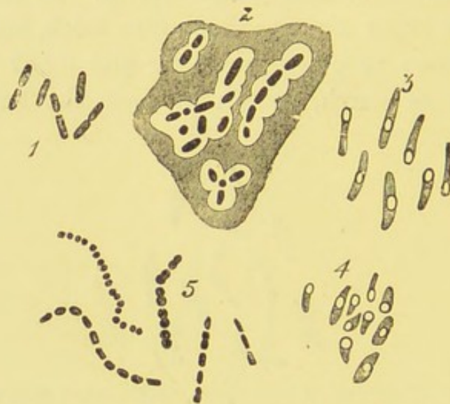
FIG. 52.— BACILLUS SYNCYANUS (AFTER NEELSEN).
