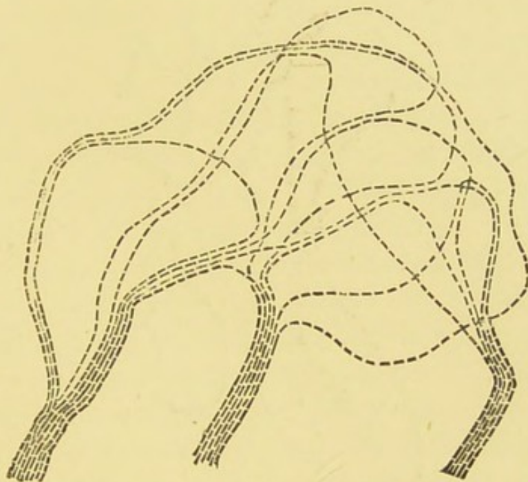
FIG. 81.—FROM AN ARTIFICIAL CULTURE OF BACILLUS ANTHRACIS.
