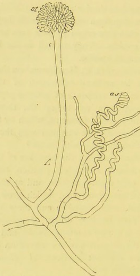
FIG. 116.—ASPERGILLUS GLAUCUS (AFTER DE BARY).
