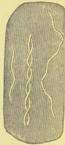
FIG. 105.—VIBRIO SERPENS, ISOLATED (AFTER COHN).
