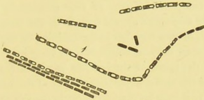
FIG. 41.—THE SAME BACILLUS AS IN PRECEDING FIGURE. At 1, spores have made their appearance.
