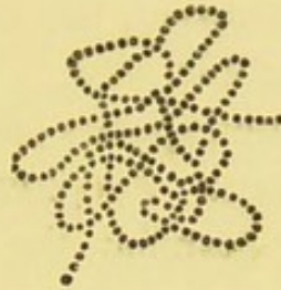
FIG. 13.—PART OF A CONVOLUTION OF CHAINS OF MICROCOCCI; FROM AN ARTIFICIAL CULTIVATION STARTED WITH THE SERUM OF A BLISTER OF A RABBIT'S EAR.
