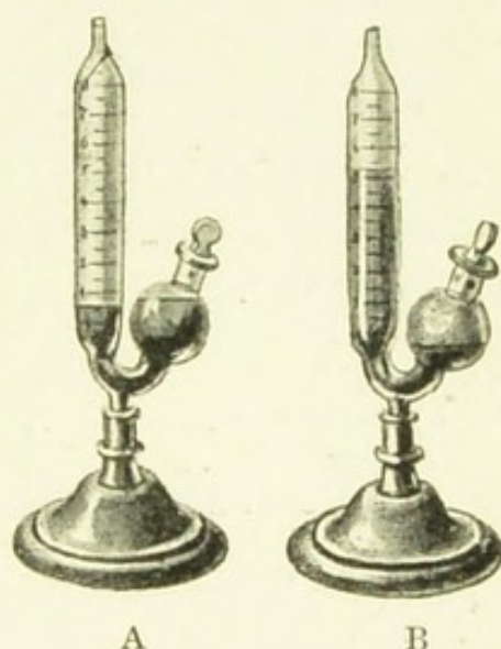
FIG. 26.—Gans' Apparatus. A, before fermentation; B, after.
