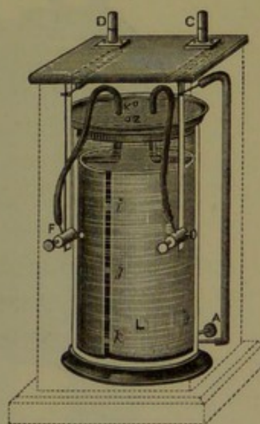
Plante's cell.
