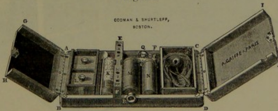
Gaiffé's sulphate of mercury pocket battery.
