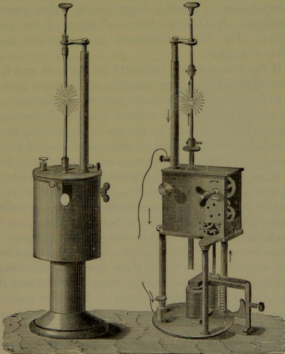
Electric lamps.
