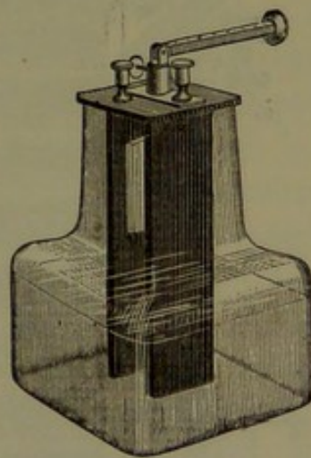
Another form of Grenet's cell.
