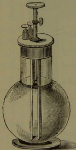
Grenet cell.
