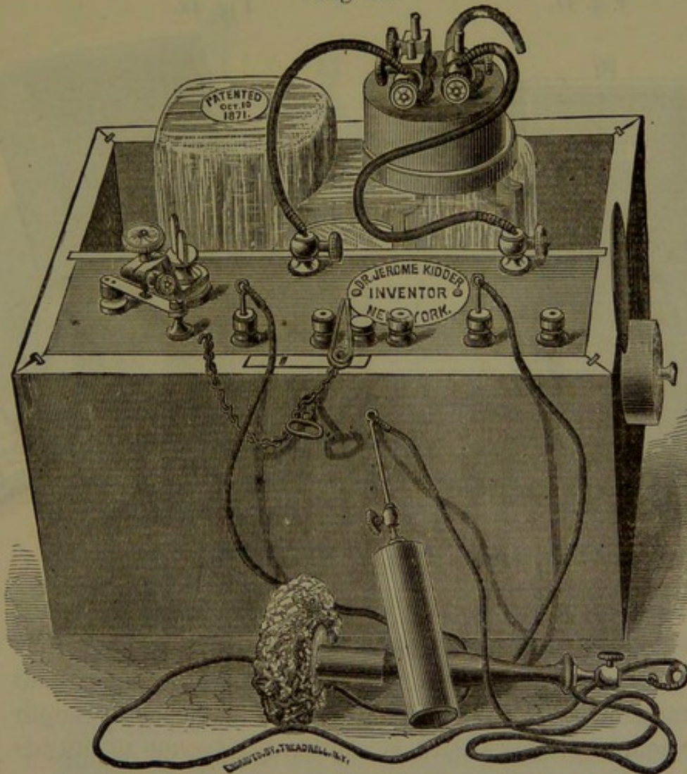
Kidder's faradic battery, with "tip cup."
