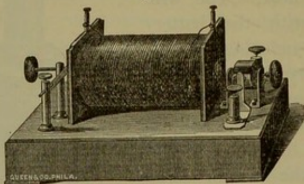
Ruhmkorff's coil.
