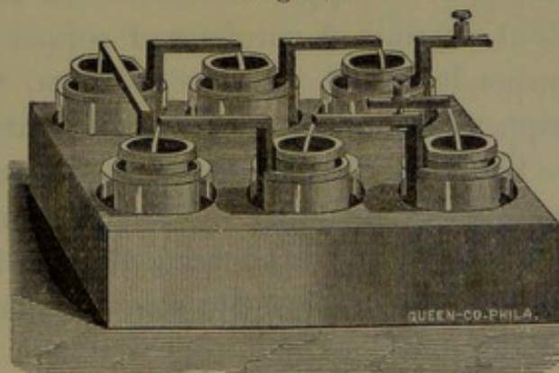
Grove's battery.
