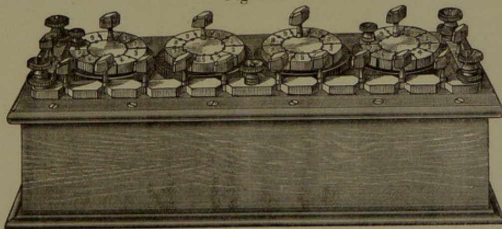
Brenner's resistance coils.
