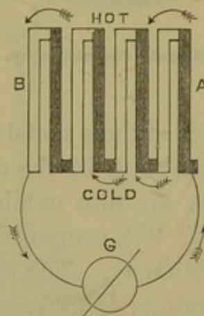
The thermo-electric multiplier.
