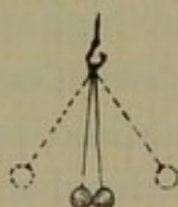
Unlike electricities attract—like, repel.
