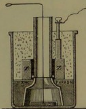
Siemens and Halske's modification of the Daniell element, as made for Remak.
