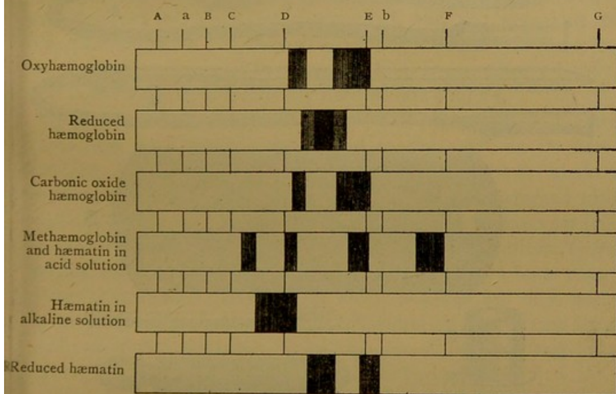
FIG. 15.—Absorption spectra of blood pigment.
