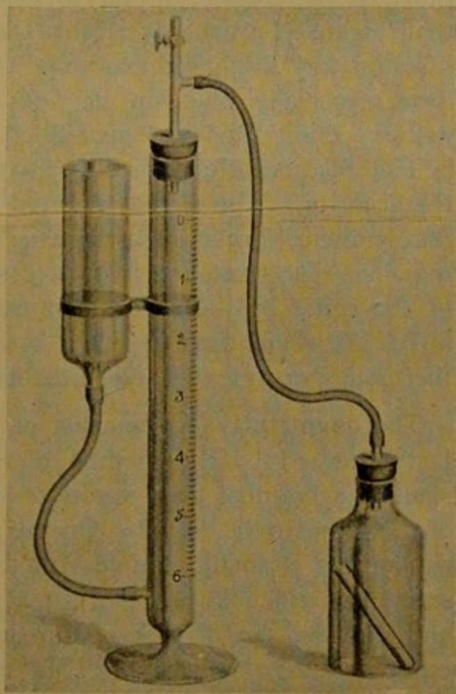
FIG. 66.—Gerrard's Apparatus for estimating Urea.
