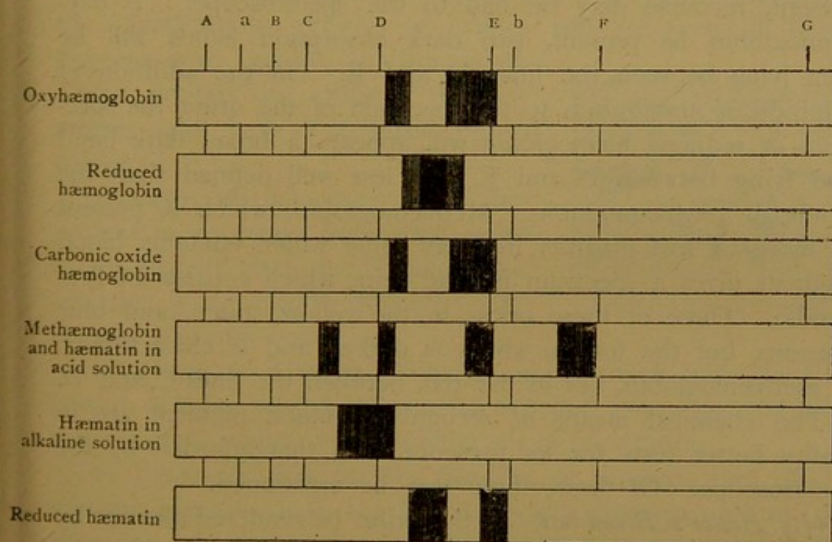
FIG. 68.—Absorption spectra of blood pigment.
