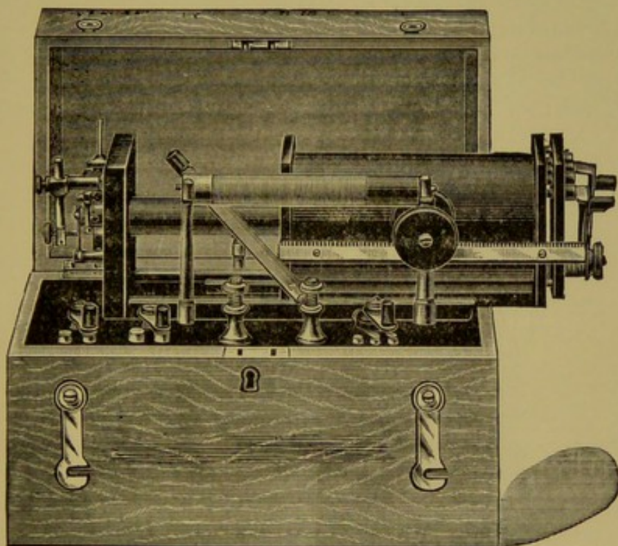
FIG. 63.—High-Tension Apparatus (Kidder).
