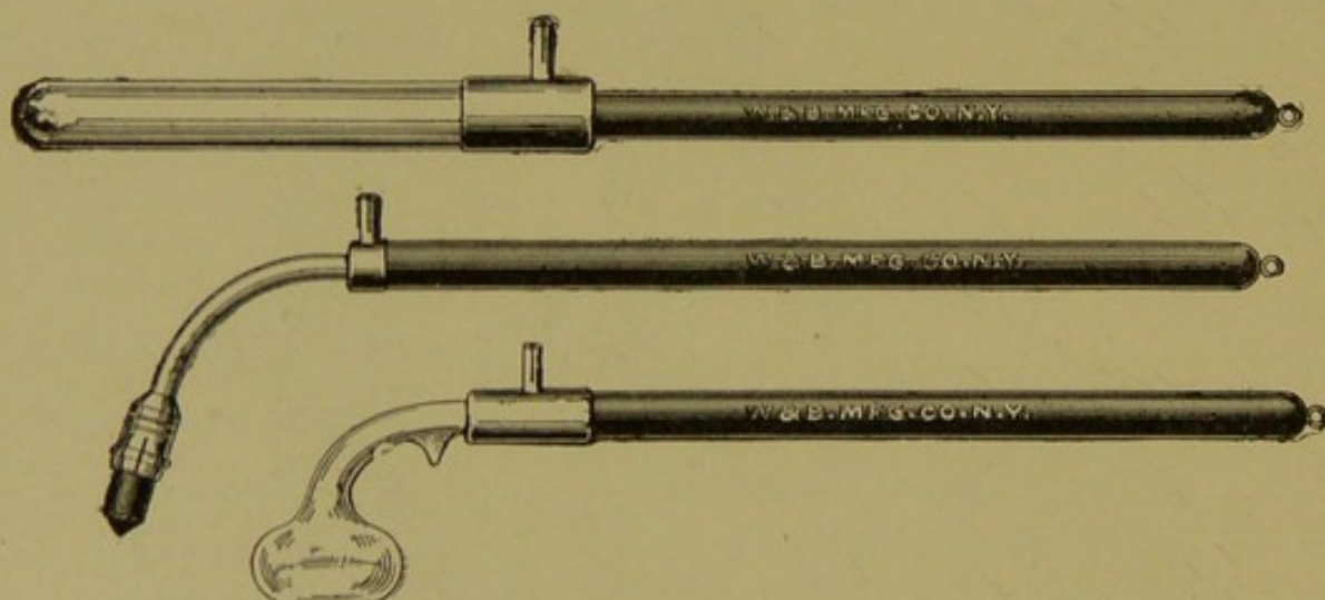
Figs. 250, 251, 252.—Various Electrodes for High Frequency Applications.
