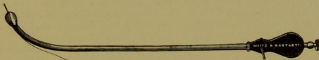
FIG. 195.—Newman's Tunnelled Catheter Electrode (Waite & Bartlett).
