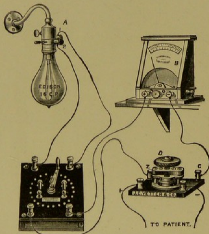
FIG. 71.—Volt Controller for Incandescent Current (Vetter).
