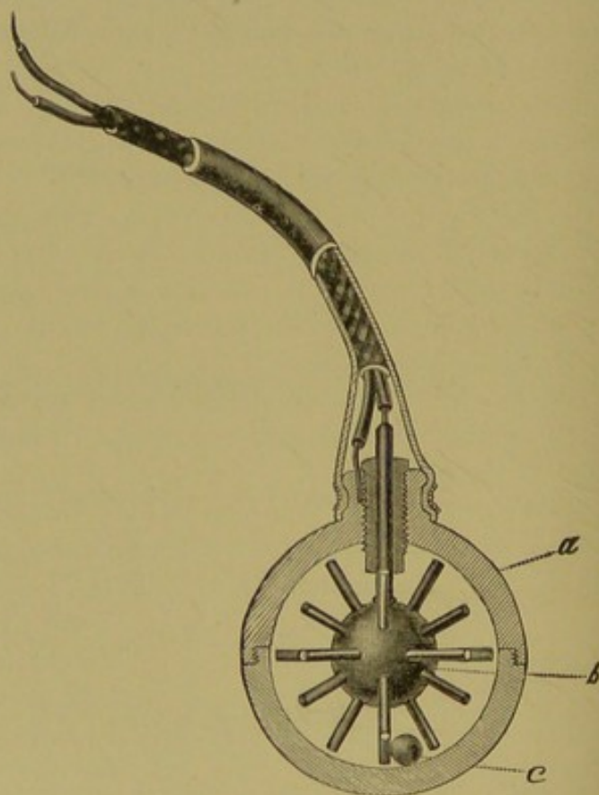
FIG. 139.—Cross-Section of the Ball, showing interior construction. (Enlarged three and a half times.) a, The two hemispheres; b, the spiked ball; c, the platinum ball.
