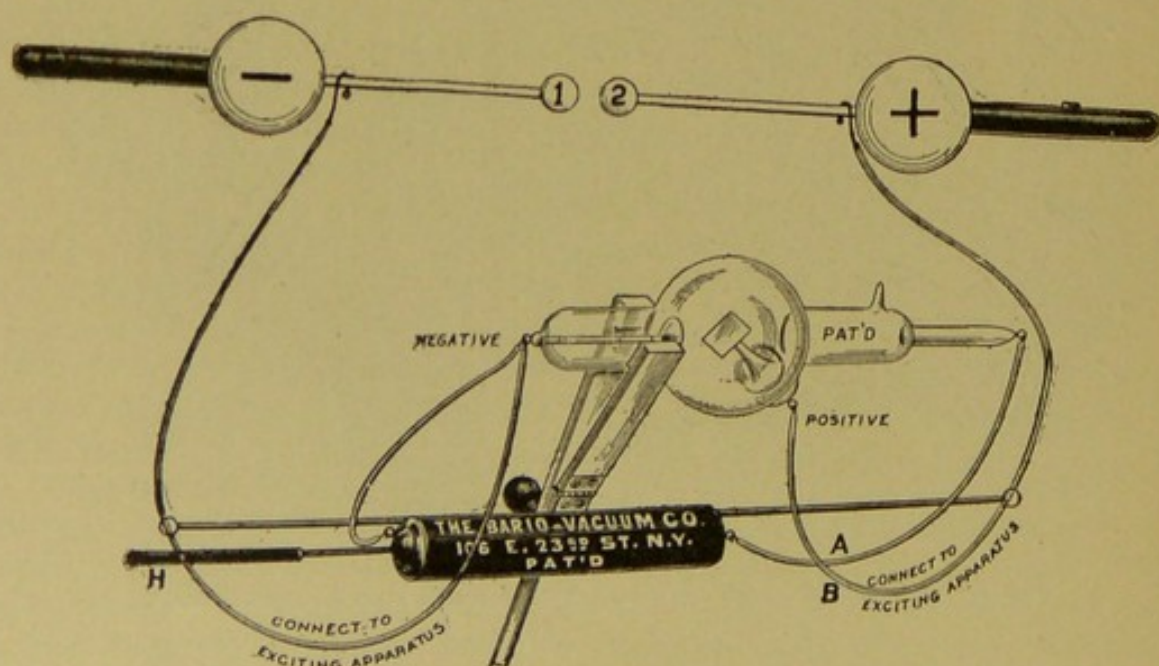
Fig. 209—The tube and vacuum regulator connected with the prime Conductors of a Static Machine. The vacuum is regulated by properly adjusting the rod or piston H.
