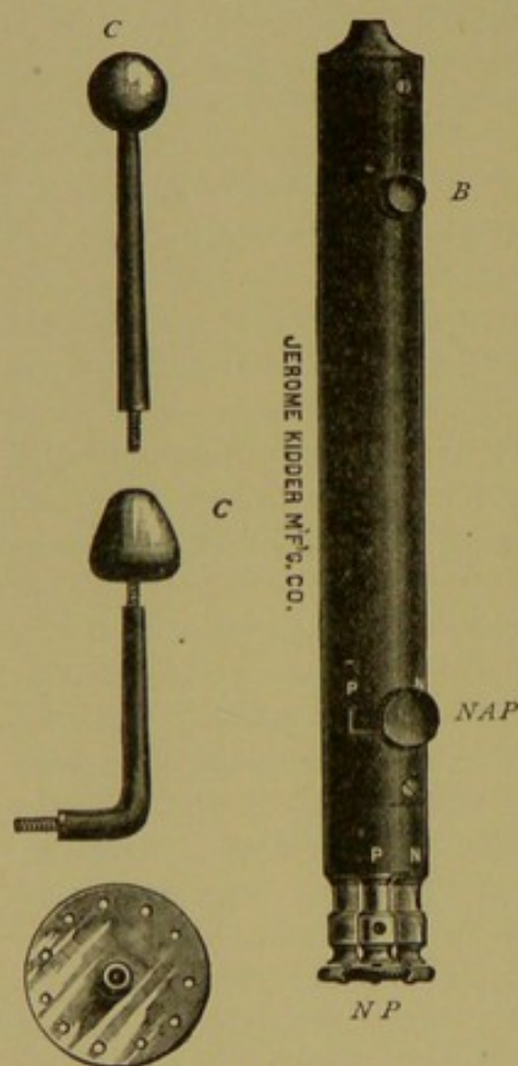
FIG. 52. Electrode for Electro-diagnosis.
