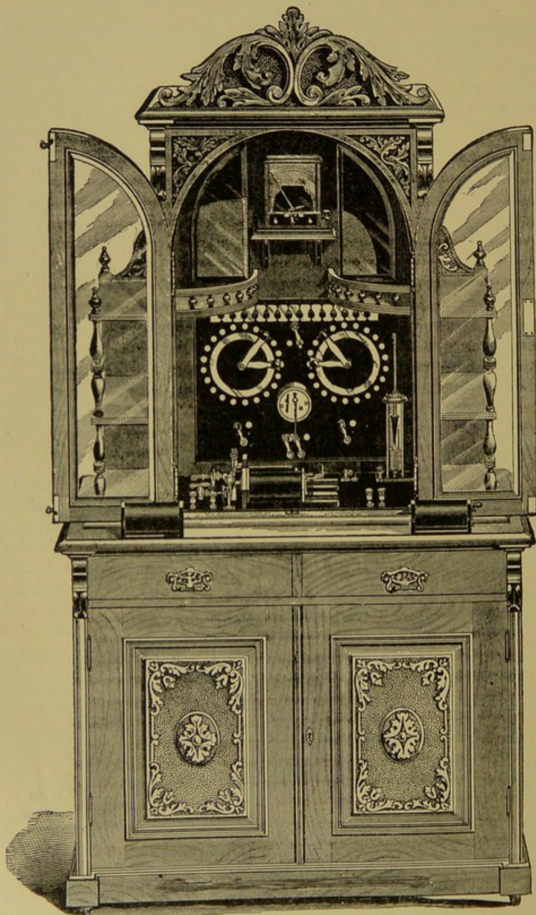
FIG. 69.—Cabinet Battery with High-Tension Coil and Wire Rheostat (Van Houten & Ten Broeck).
