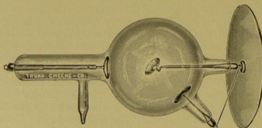
Fig. 205—Double Focus Self-Regulating Tube.
