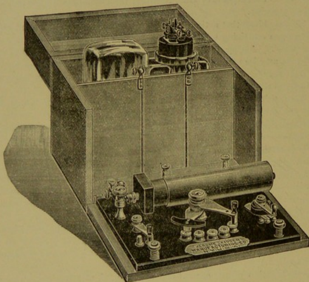
FIG. 57.—Continuous Coil Machine with Tip Battery (Kidder).
