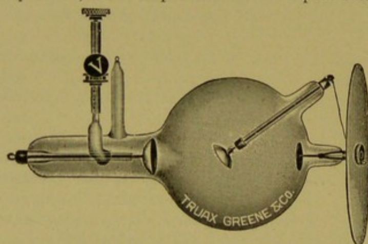
Fig. 204—Double Focus Tube.
