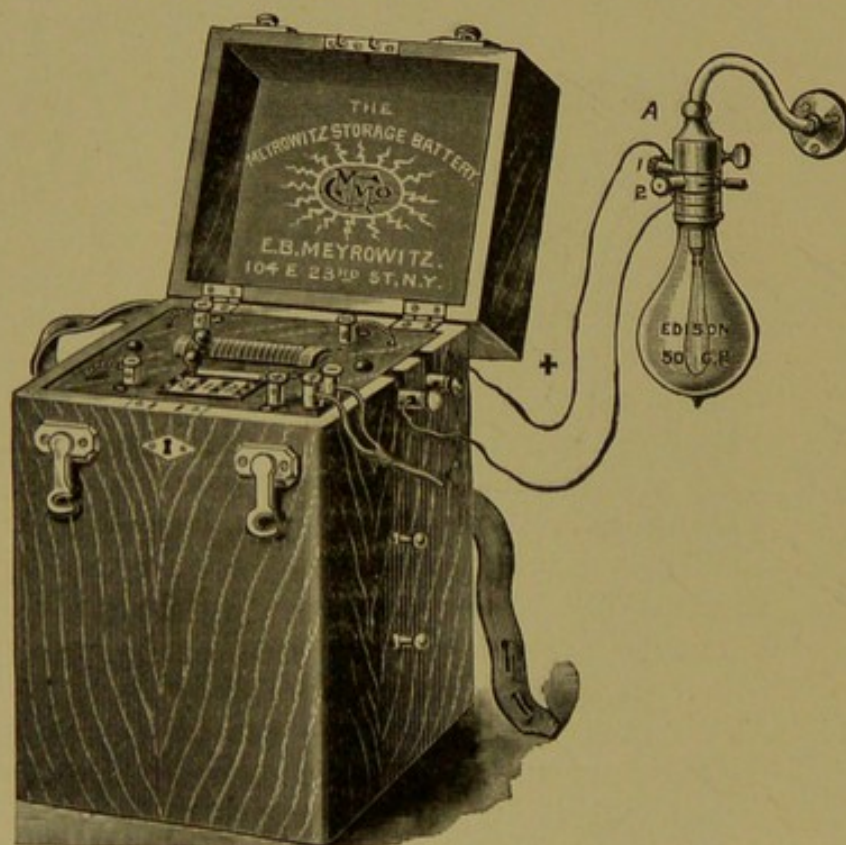
FIG. 182.—Storage Battery with Vetter Current Adapter.
