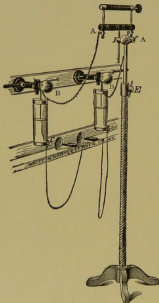
FIG. 121.—Ranney's Static Current Controller (Waite & Bartlett).
