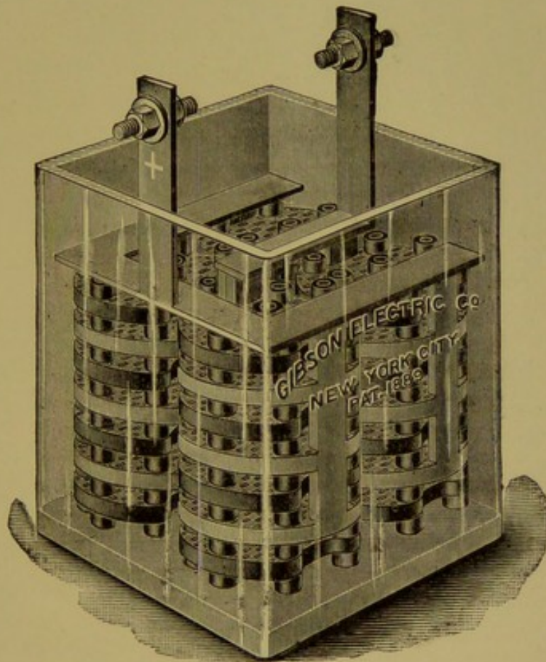
FIG. 183.—Storage Battery.
