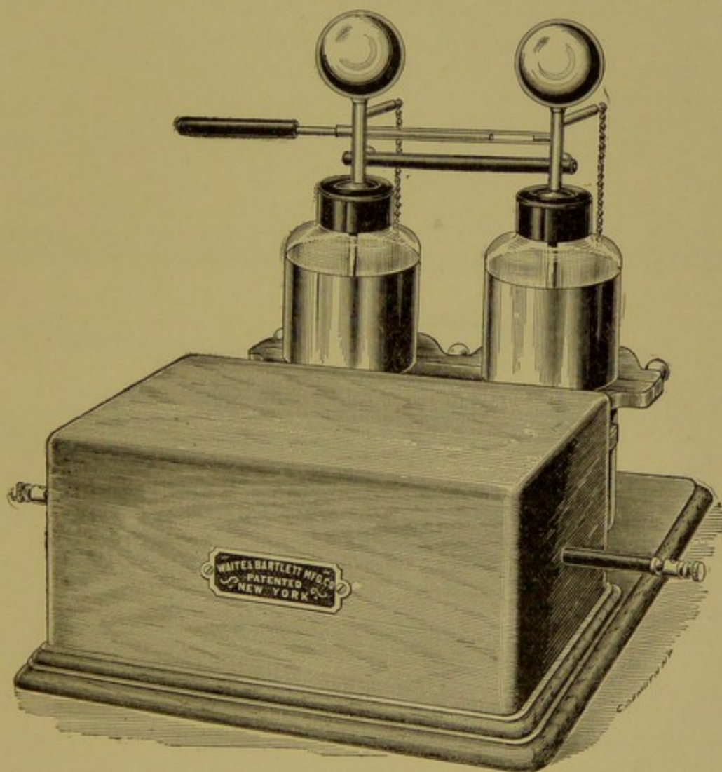
Fig. 249.—Hyperstatic or High Frequency Apparatus.
