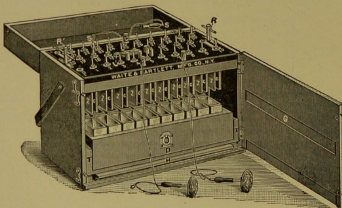
FIG. 66.—Plug and Socket Galvanic Battery (Waite & Bartlett).
