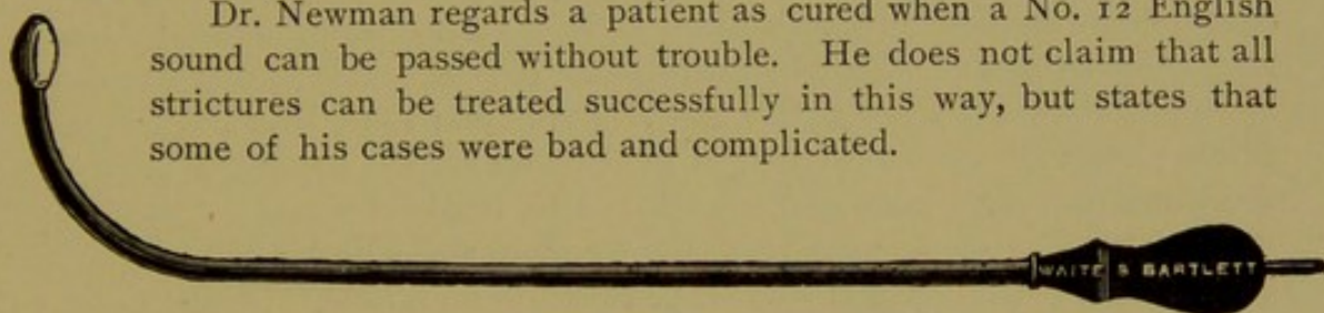
FIG. 196.—Egg-Shaped Urethral Electrode.
