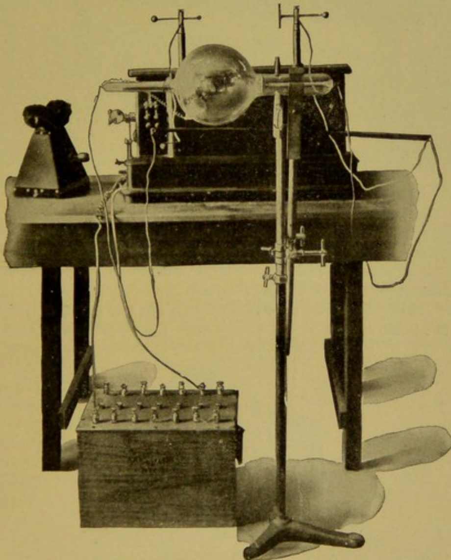
Fig. 211.—Scheidel's Portable Coil with Battery.
