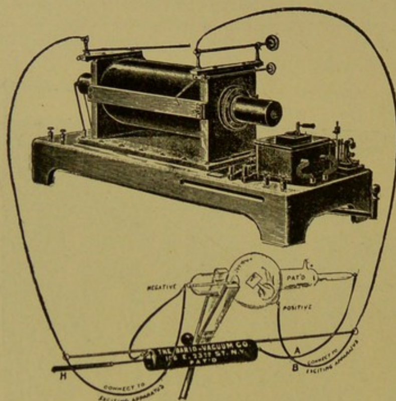
Fig. 208.—Induction Coil connected with vacuum tube and with regulator H for lowering or raising the resistance of the tube at will.
