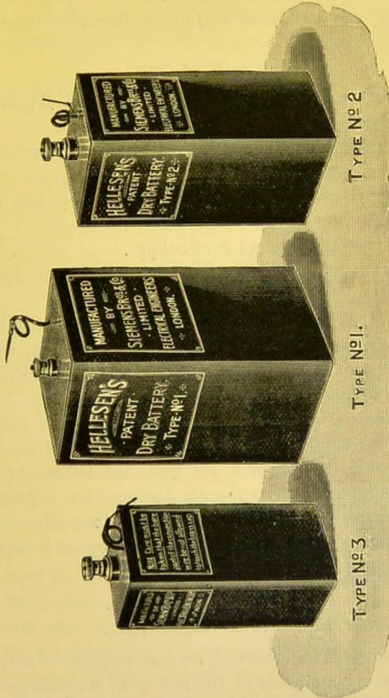
FIG. 22.—HELLESEEN CELLS.
