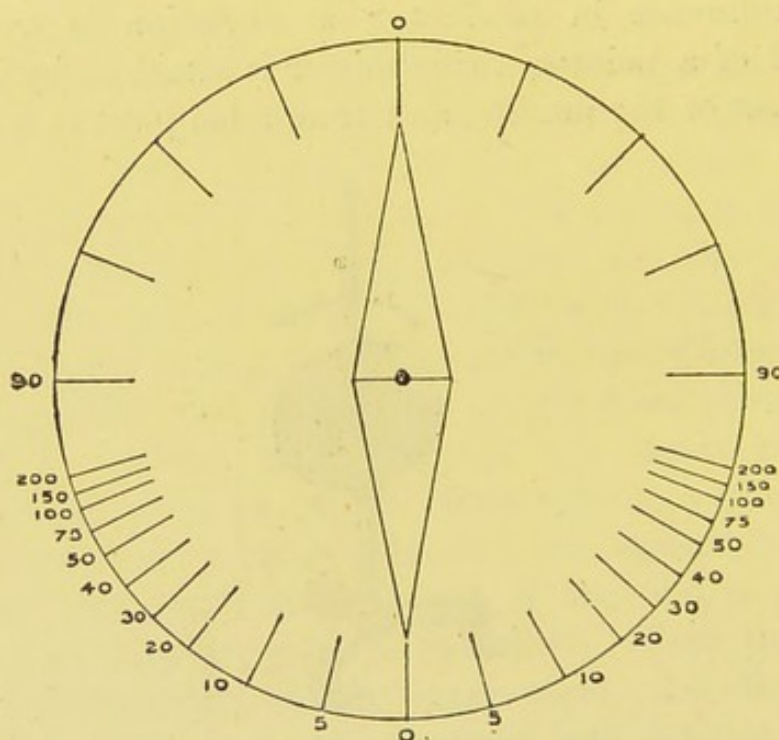
FIG. 39.—DIAGRAM OF A GALVANOMETER, DIVIDED IN ITS UPPER HALF INTO DEGREES, AND IN ITS LOWER HALF INTO MILLIAMPERES.
