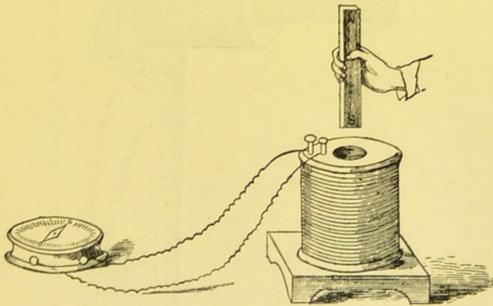
FIG. 64.—INDUCING ACTION OF A MAGNET ON A CLOSED CIRCUIT.
