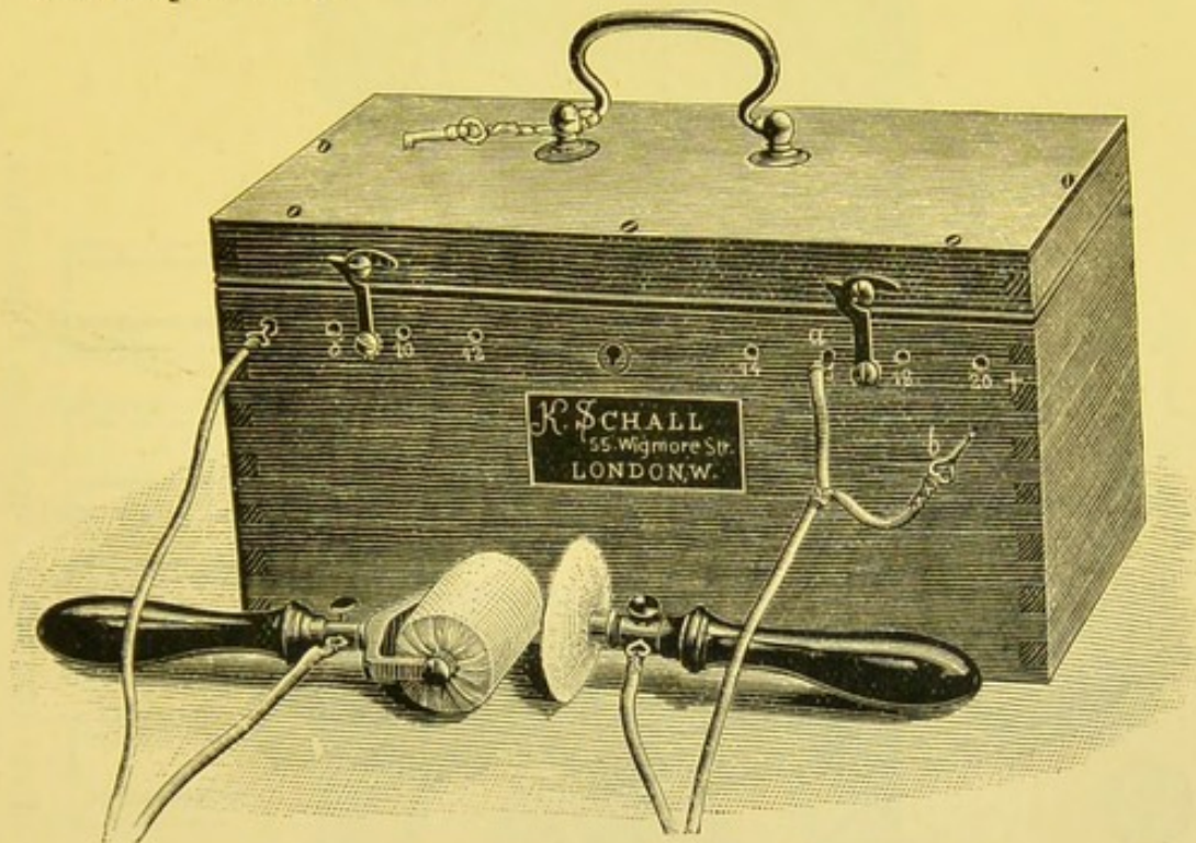
FIG. 46.—BATTERY WITH PLUG COLLECTOR.
