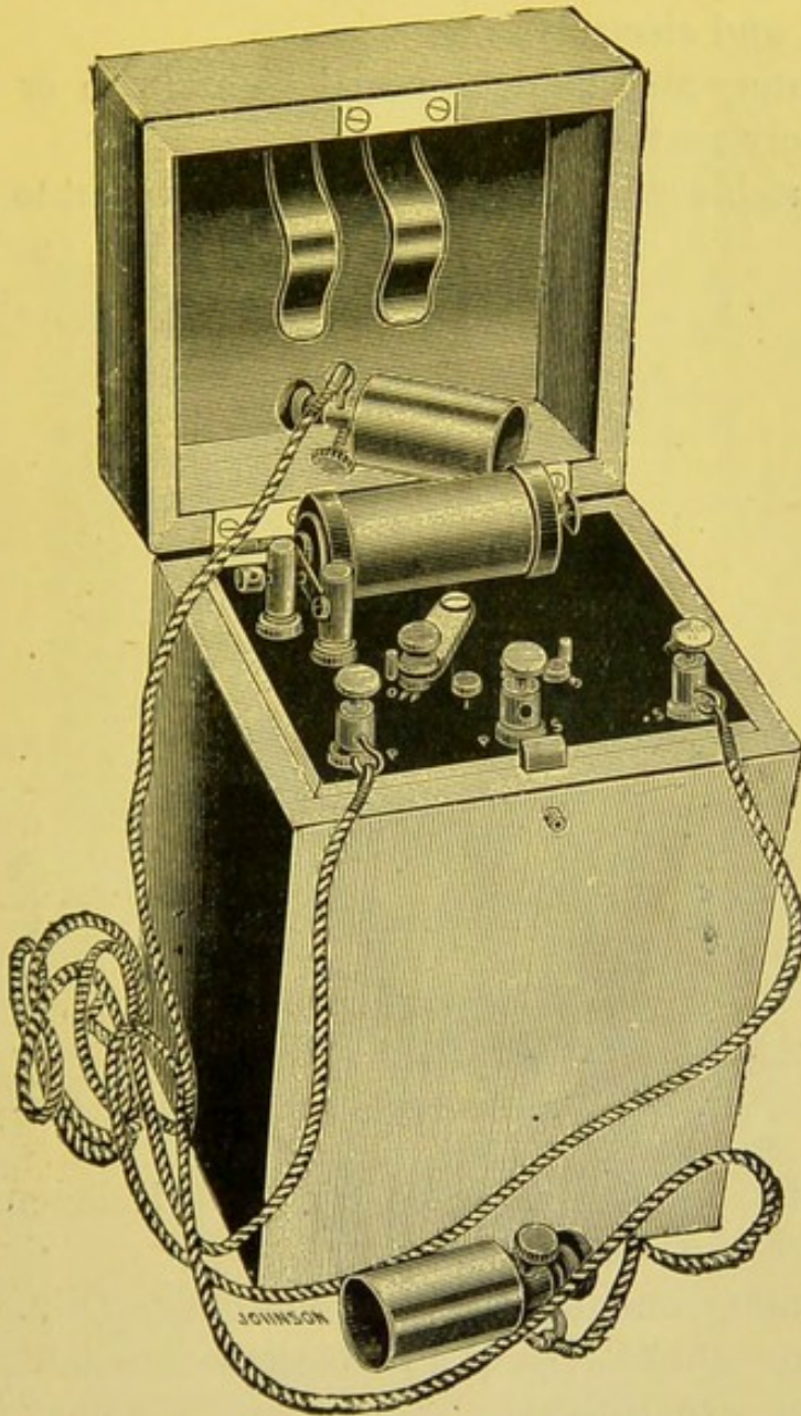
FIG. 83.—FARADIC BATTERY.
