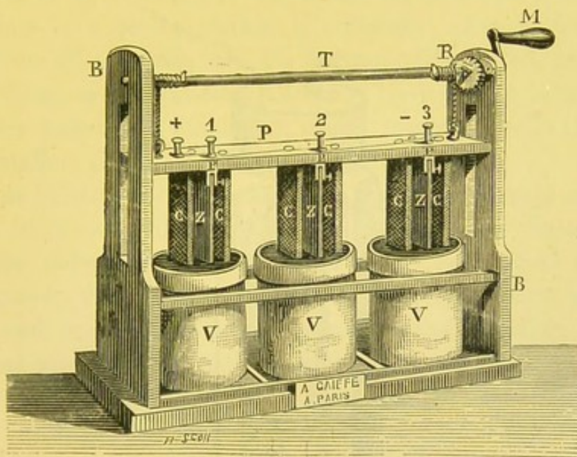
FIG. 18.—BICHROMATE BATTERY.
