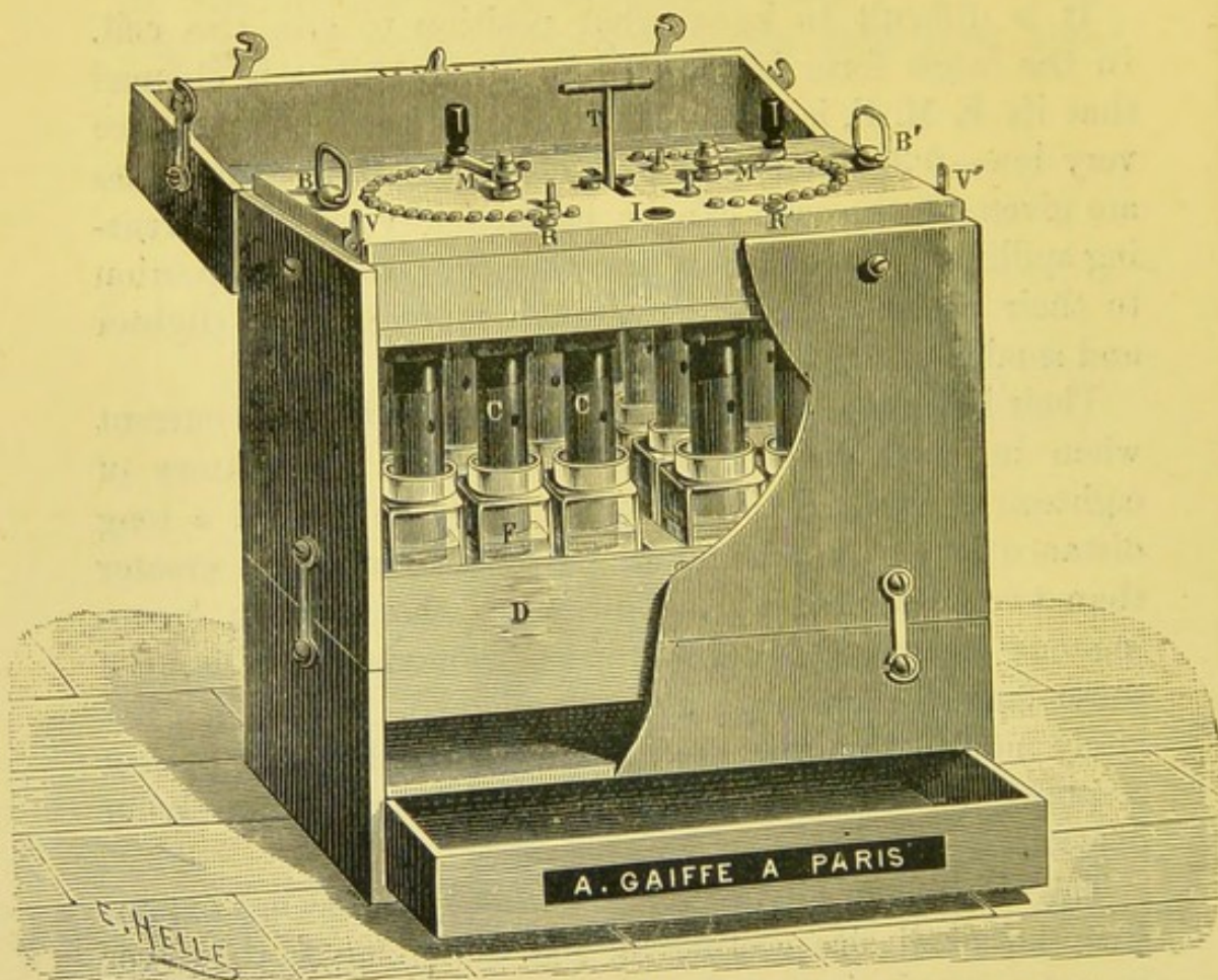
FIG. 20.—PERSULPHATE OF MERCURY CELL BATTERY.
