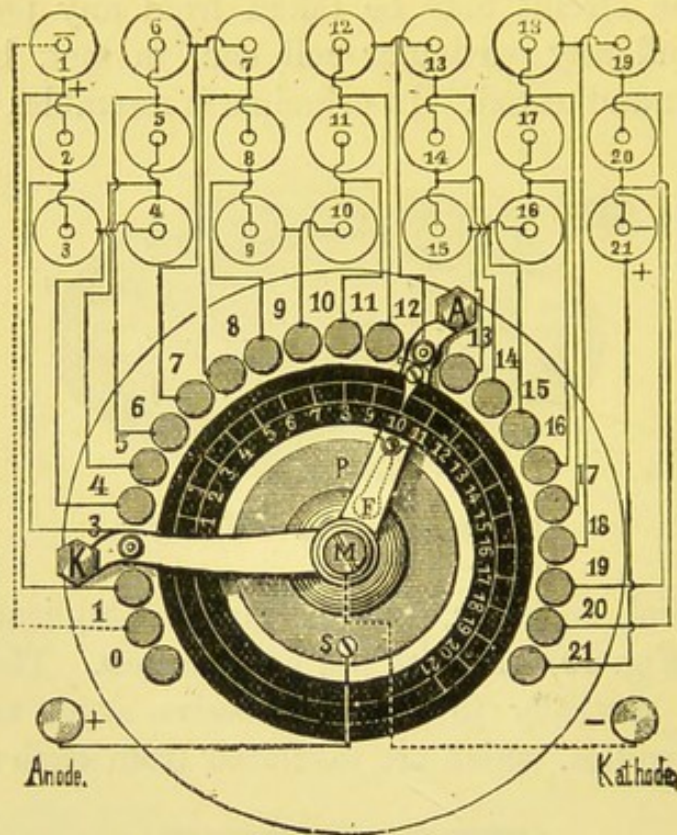
FIG. 50.—CONNECTIONS OF DOUBLE COLLECTOR.
