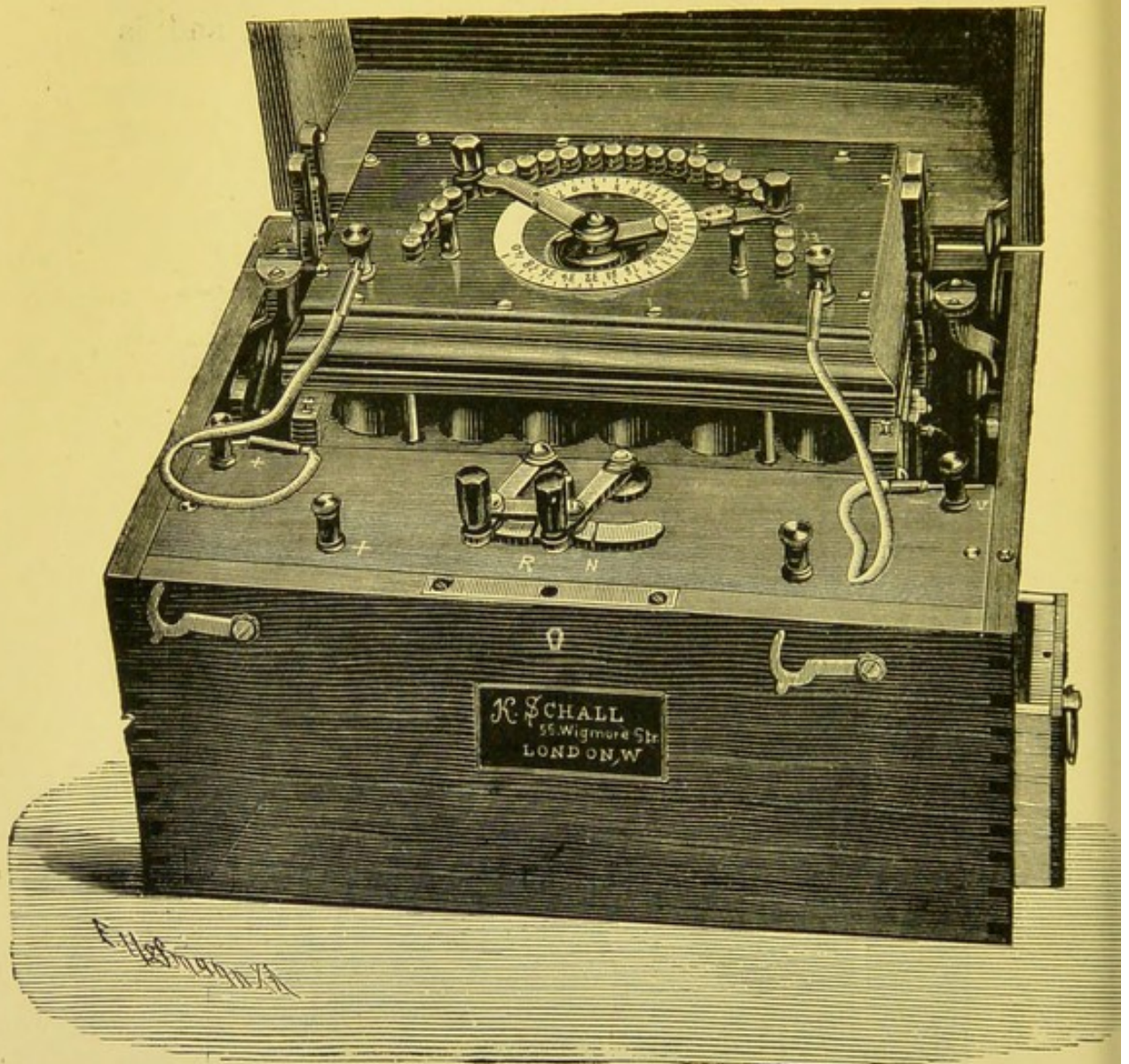
FIG. 86.—REINIGER'S BATTERY WITH AUTOMATIC PLUNGE APPARATUS.
