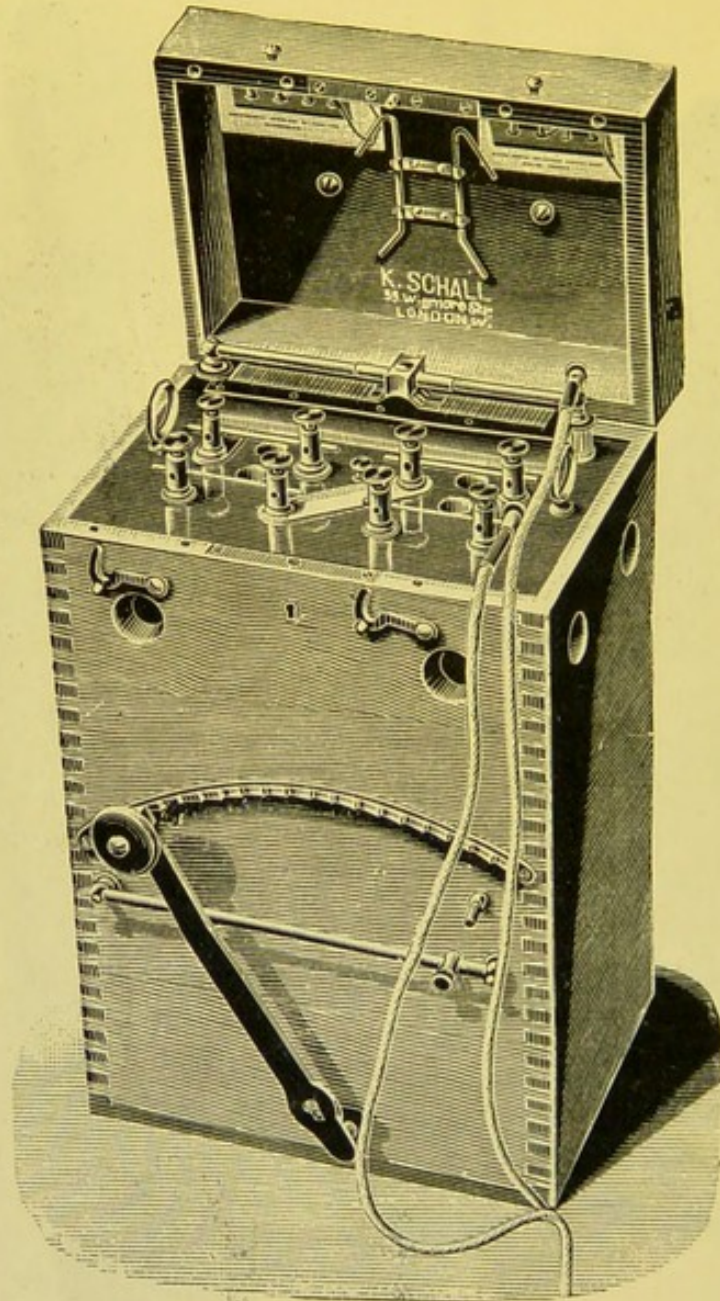
FIG. 82.—VOLTOLINI'S BATTERY.
