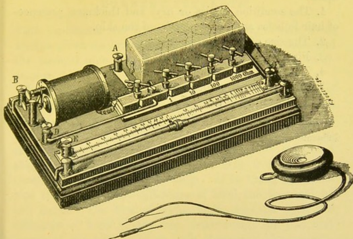
FIG. 30.—Kohlrausch's BRIDGE.
