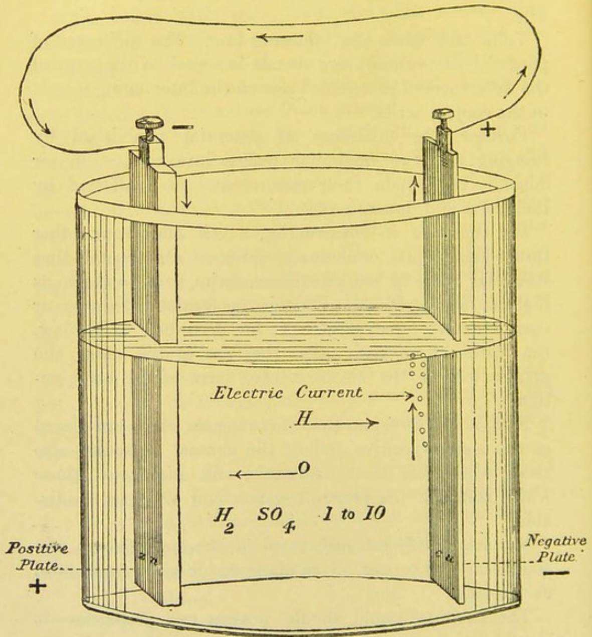
FIG. 12.—SIMPLE CELL.
