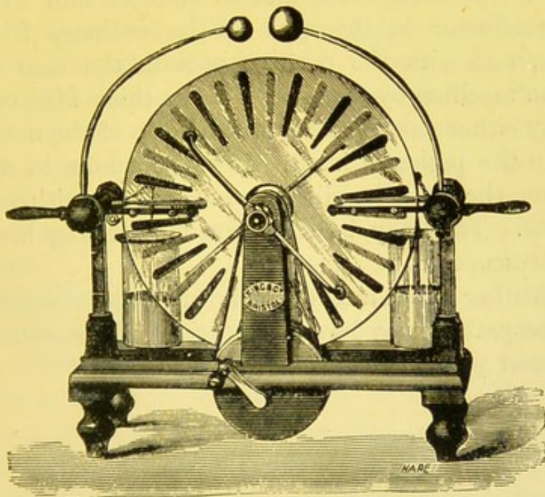
FIG. 6.—WIMSHURST MACHINE.
