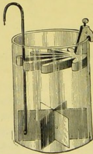
FIG. 25.—GRAVITY CELL.
