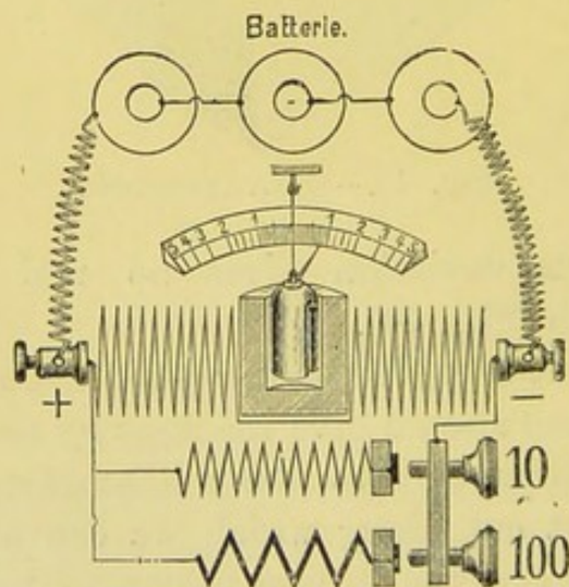
FIG. 42.—GALVANOMETER SHUNTS.
