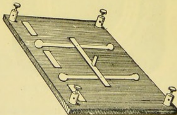
FIG. 51.—CURRENT REVERSER.
