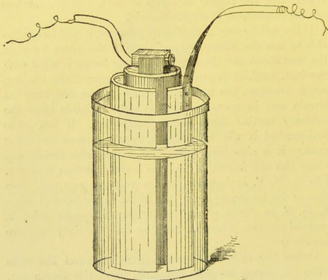
FIG. 26.—BUNSEN CELL.
