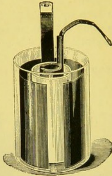
FIG. 24.—DANIELL CELL.
