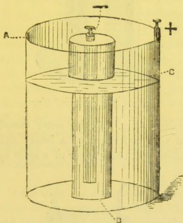
FIG. 23.—DANIELL CELL.
