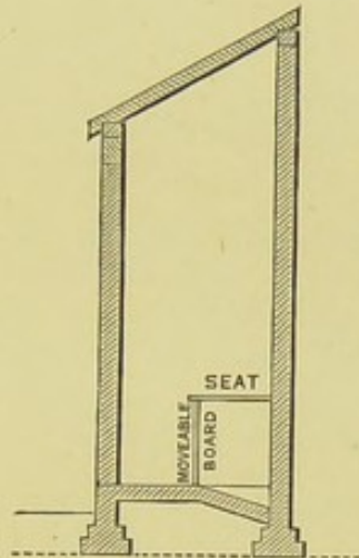
SECTION OF PRIVY
