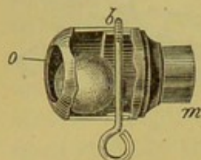
FIG. 165.—Luer's ball valve with side removed. m , mouth which fits into the end of the tracheal canula; b , wire to limit the movement of the ball; o , orifice.
