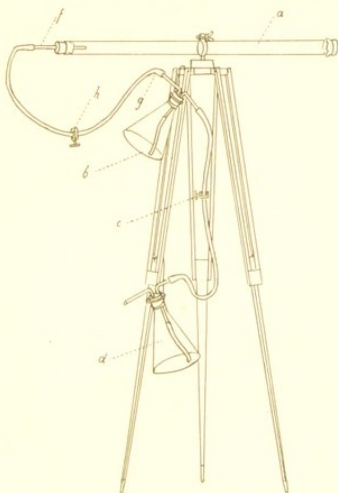
FIG. 46.—Hesse's tube, mounted for use.
