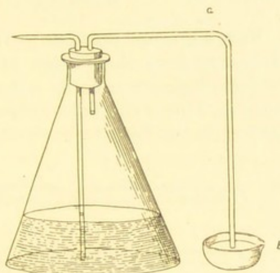
FIG. 25.—Flask arranged for culture of anaerobes which develop gas.
