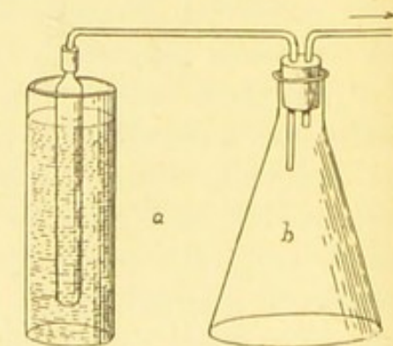
FIG. 31.—Chamberland's candle and flask arranged for filtration.
