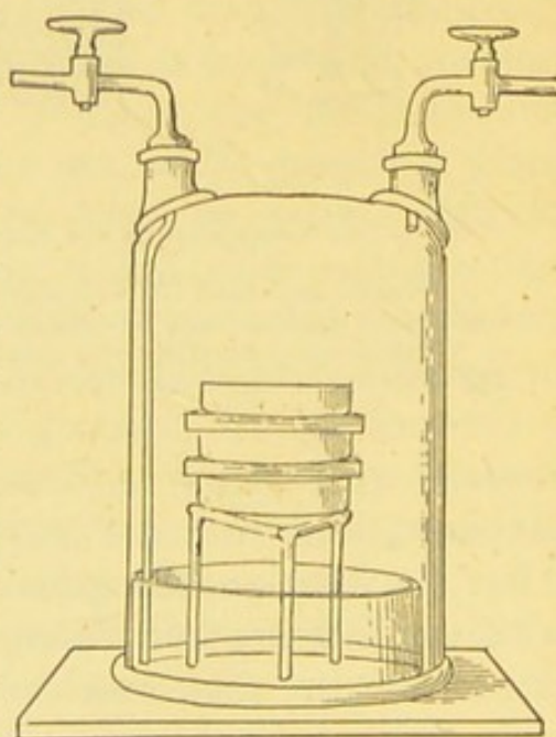
FIG. 23.—Bulloch's apparatus for anaerobic plate cultures.
