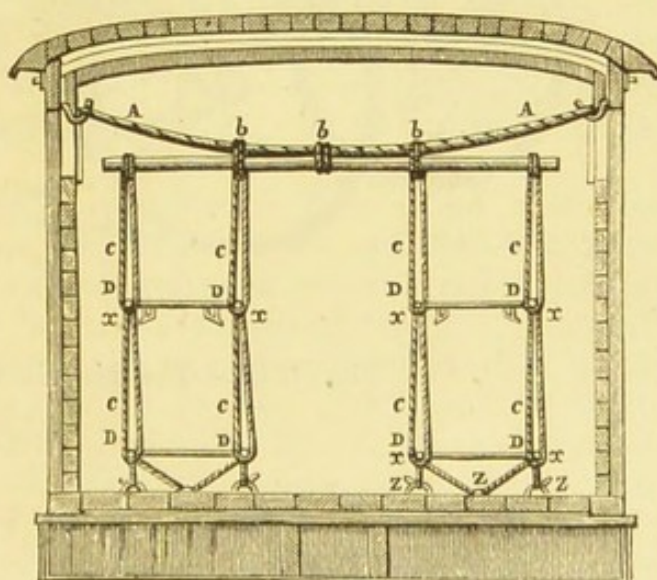
Fig. 151.—Plan of railway ambulance waggon (Zavodovski).
