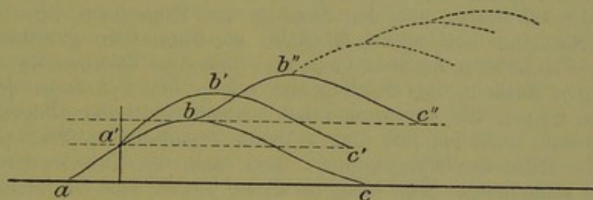
Fig. 78. Summationscurve.
