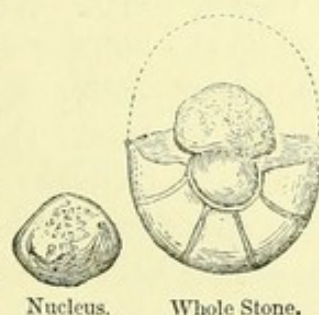
Nucleus.
