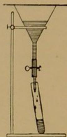
FIG. 2. Apparatus for filling test-tubes.
