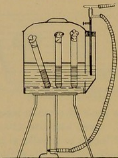
FIG. 17. Water-bath for cooling agar.
