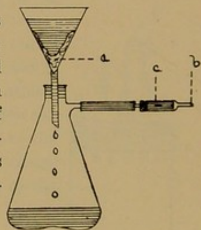
FIG. 5. Apparatus for filtering media through absorbent cotton; a, coil of wire overlaid with layer of absorbent cotton; b, tubes for making connection with air pump; c, Bunsen valve to prevent entrance of water into flasks.
