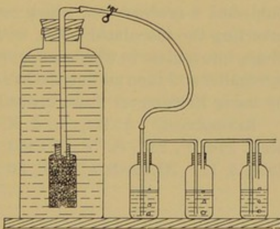
FIG. 32. Hydrogen Generator.
