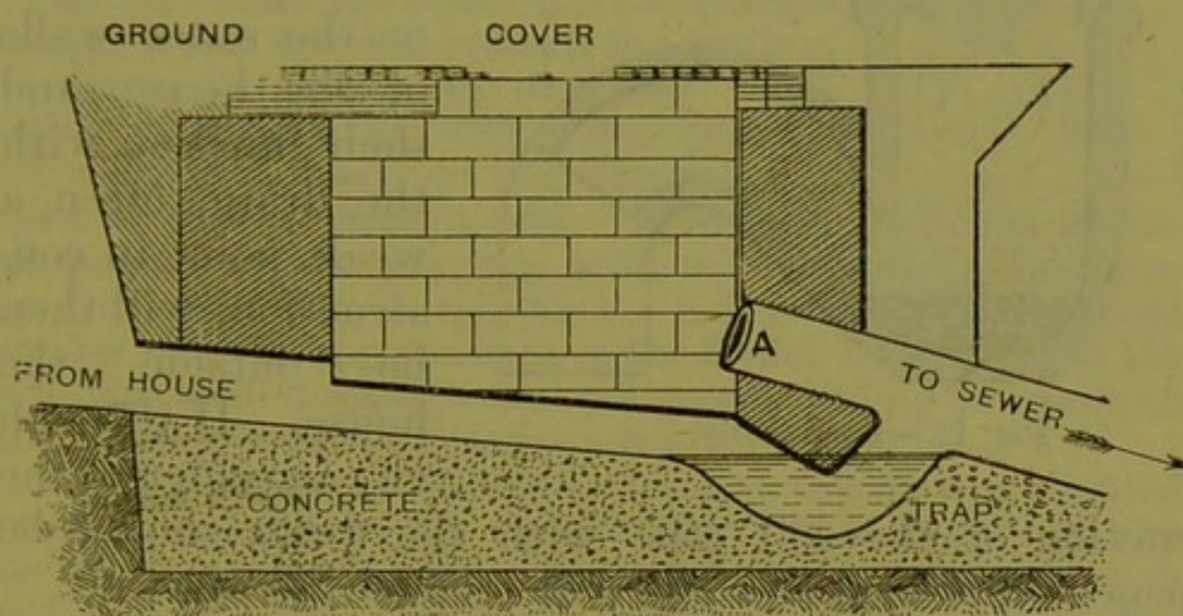
Fig. 11.—Disconnection (Inspection) Chamber.
