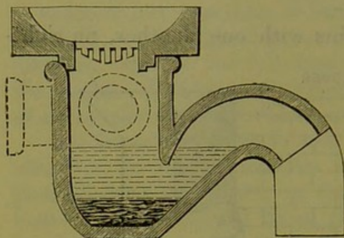
Fig. 12.—Yard Gully.
