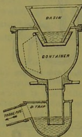
Fig. 22.—Pan Closet, with D-trap.
