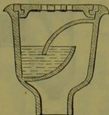
Fig. 15.—Antill's Trap.
