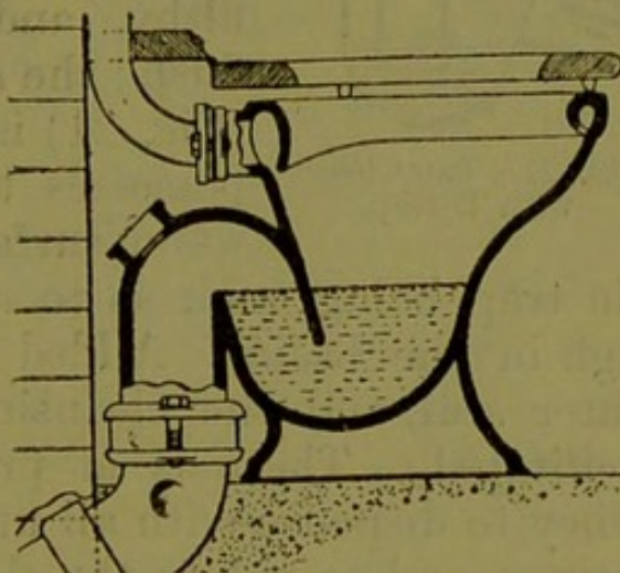
Fig. 21.—Wash-down or Short Hopper Closet.
