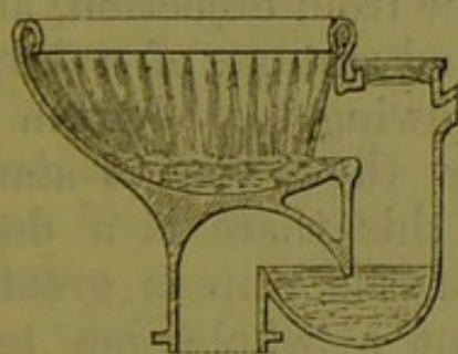
Fig. 20.—Wash-out Closet.
