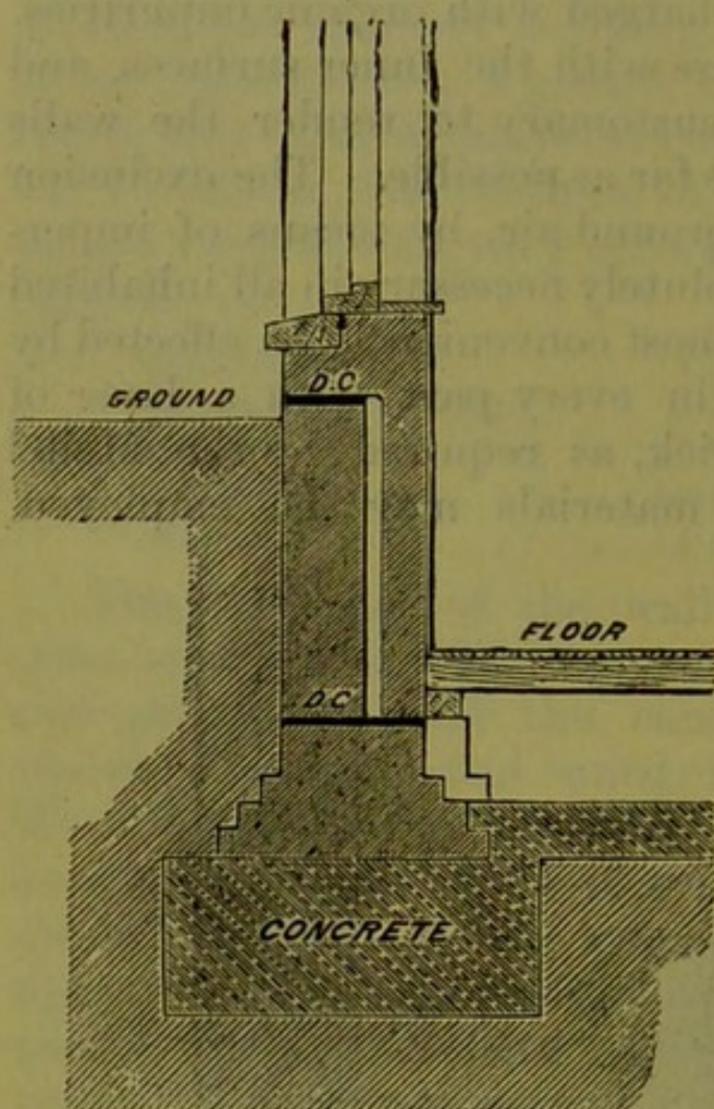
Fig. 6.—Double damp-course. Soil abutting upon hollow wall.
