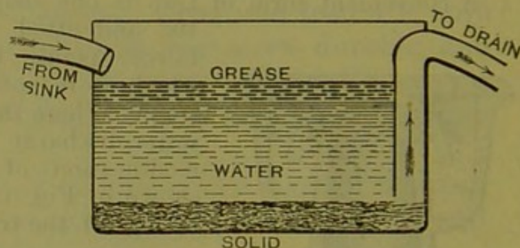
Fig. 16.—Grease Trap.
