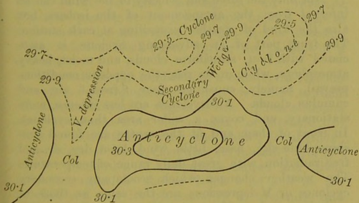
Fig. 3.—Distribution of Pressure over the North Atlantic, and parts of the United States and Europe, Feb. 27th, 1865.
