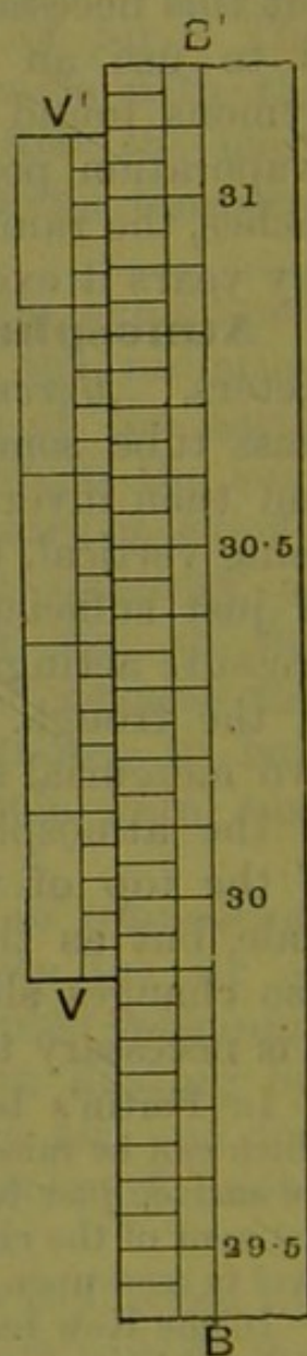
Fig. 1.—Barometer Scale and Vernier, showing a reading of 29.85 + 18 \times \cdot 002 = 29.886 inches.
