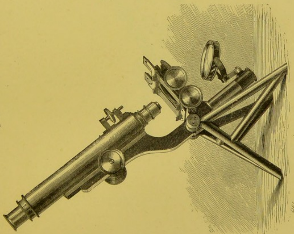
Complete microscope, designed by Mr. Higbly.
