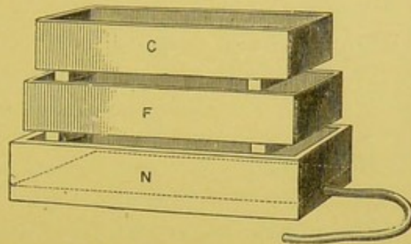
Dredging sieves, C and F, and draining tray, N. The dredge, Fig. 228 drag hook, Fig. 230, net, Fig. 231, all pack into N. Designed by Mr. Highley. p. 149.
