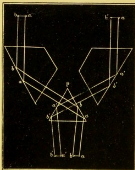
Arrangement of prisms in Nachet's binocular microscope. p. 11.
