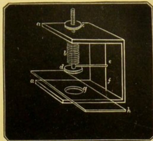
Instrument for applying graduated pressure to objects under thin glass. p. 51.
