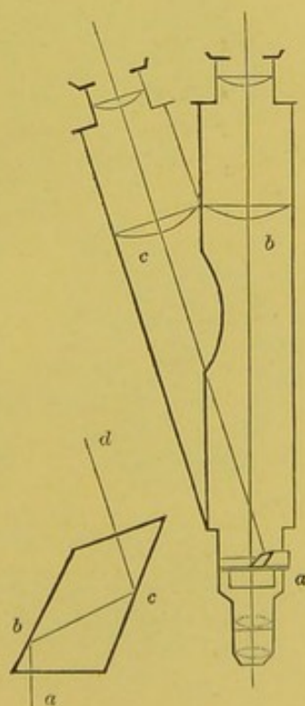
Binocular microscope as recently arranged by Mr. Wenham, and now generally adopted. p. 11.
