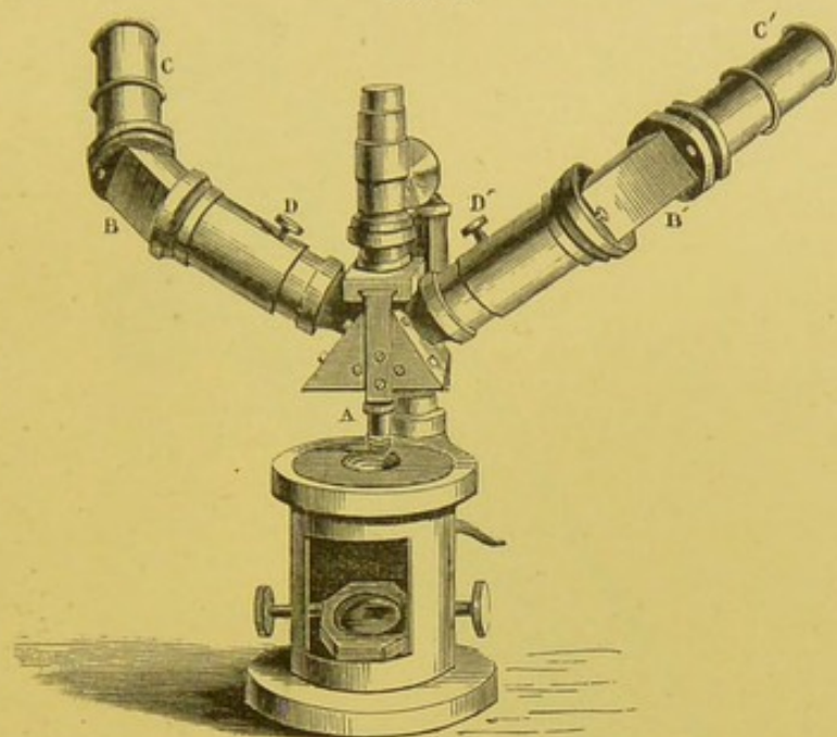
M. Nachet's microscope, to enable two observers to examine an object at the same time.
