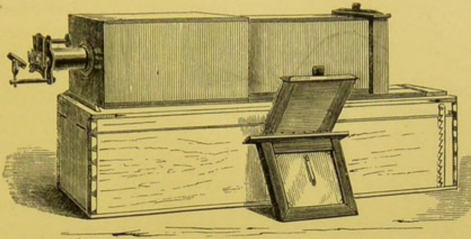
Photographic microscope camera used by Mr. Delves, arranged by Mr. Highley. p. 231.
