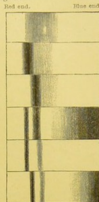
Absorption bands produced by different substances. p. 211
