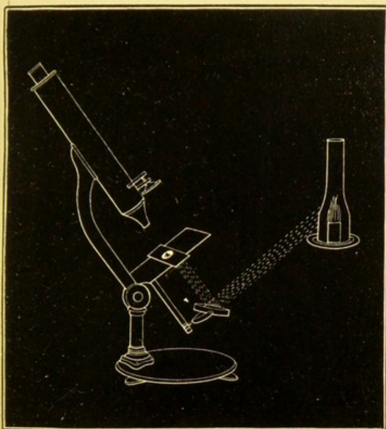
Diagram to show the arrangement for examining objects by transmitted light p. 18.
