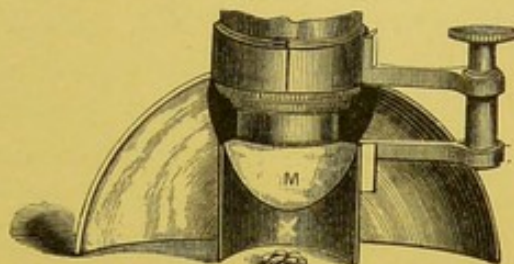
Beck's parabolic reflector, with Mr. Sorby's modification. p. 21.
