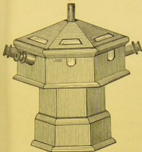
Octagonal box for holding eight microscopes, illuminated by one lamp in the centre. p. 16.
