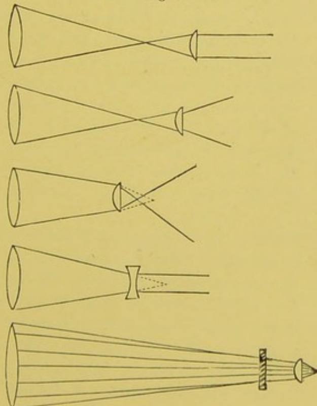
To illustrate the observations of Dr. Moitessier on illumination and the position of the condensing lens. p. 251.
