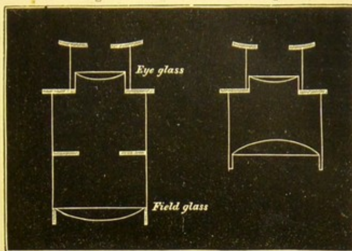
Negative or Huyghenian eye-piece. p. 5.
