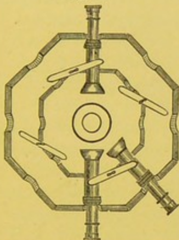
Section of Fig. 31, showing relative positions of microscope and lamp, mode of fixing, &c. p. 16.
