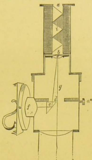
Mr. Sorby's spectrum eye-piece for the microscope, with arrangement for producing two spectra for comparison p. 219
