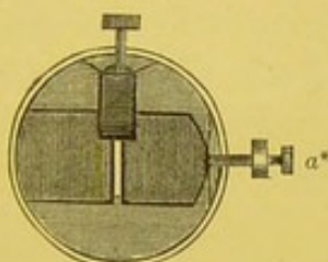
Arrangement for altering the length and breadth of the spectrum. p. 219.
