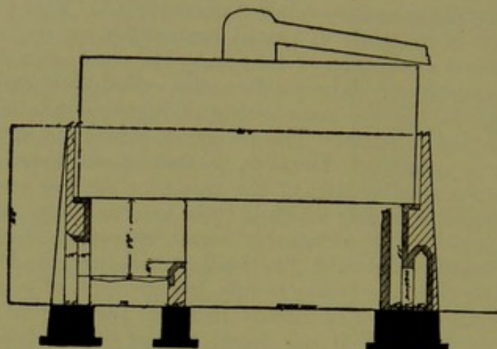
Lateral vertical section of cylindrical still.
