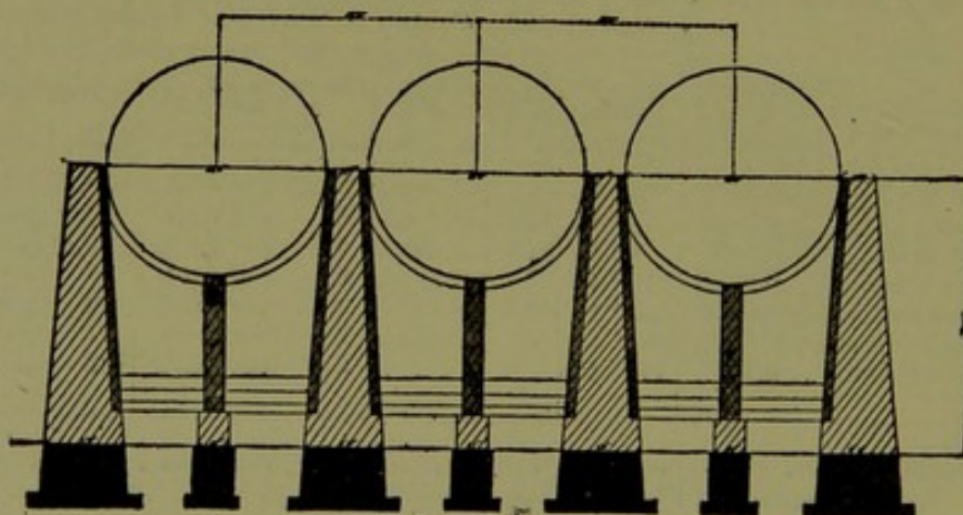
Transverse vertical section of cylindrical still.
