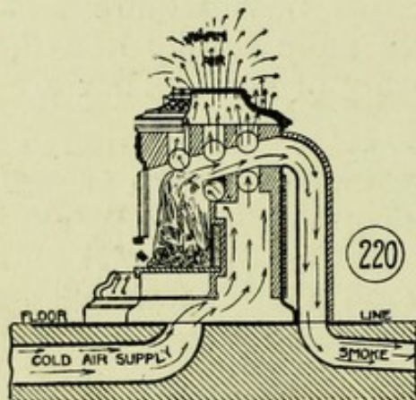
SECTION OF SHORLANDS PATENT MANCHESTER STOVE
