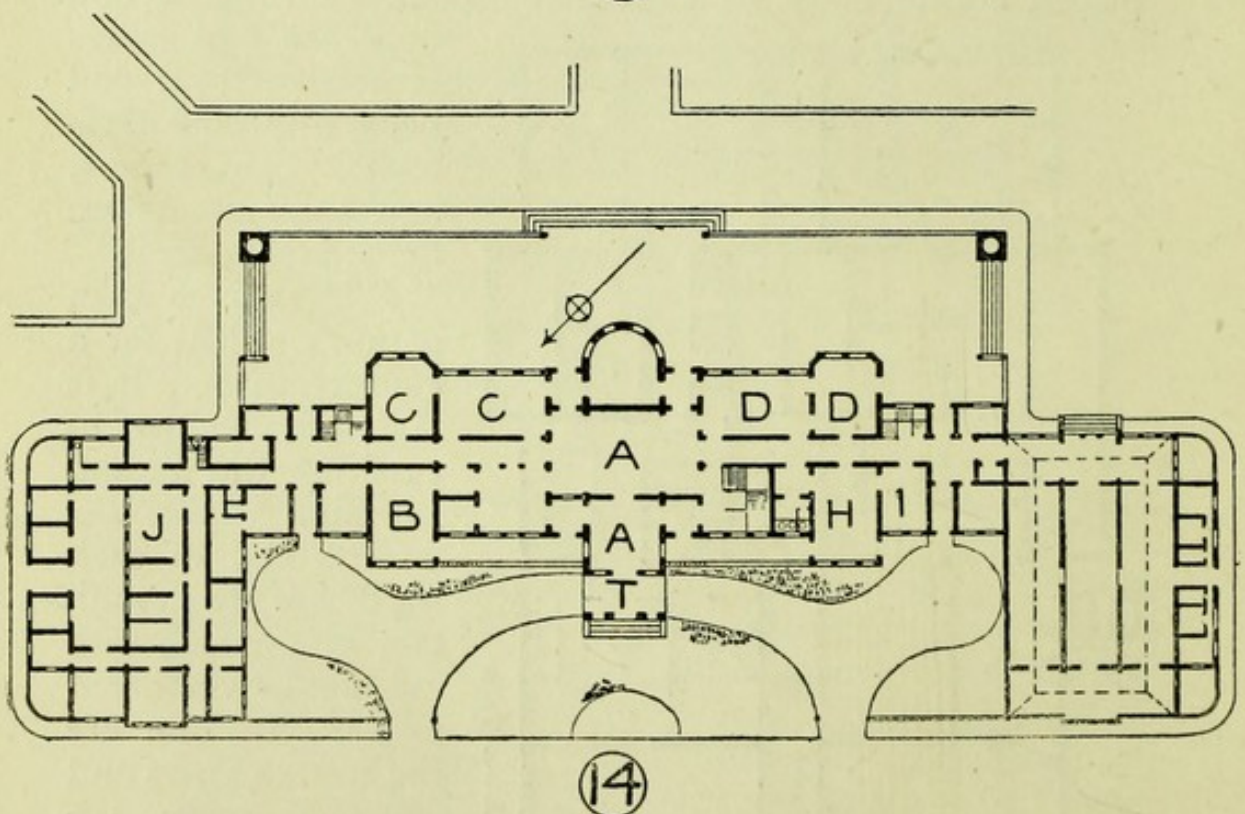
Fig. 14 is the ground plan of a large country house . It forms a crescent shape on plan so that all the living rooms may, as far as possible, get the sun's rays at some portion
