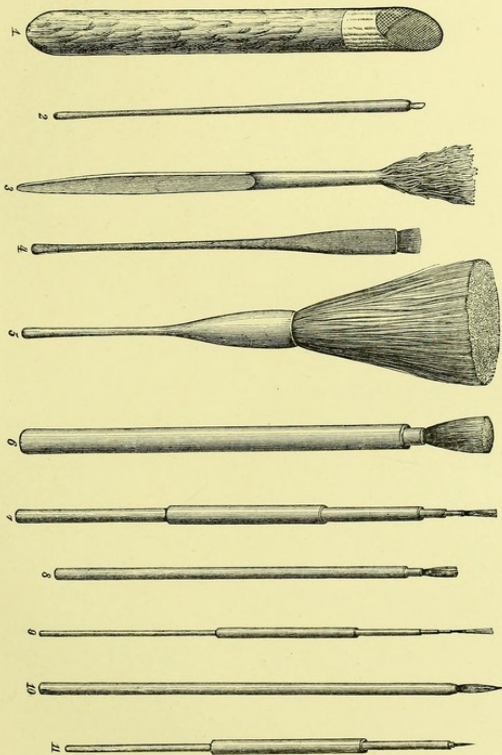
TOOLS USED IN LACQUER INDUSTRY.
