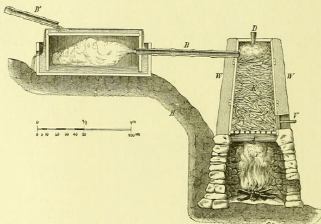
Fig. 8. APPARATUS FOR PRODUCING CAMPHOR IN TOSA, JAPAN.
