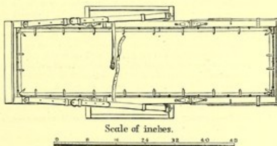
FIG. 16.—Plan of MCELDERRY'S single mule-litter.
