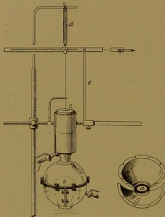
FIG. 111. — Roy's Cardiometer to measure the output of blood from the heart. b , heart in cardiometer chamber; c , piston recorder working on lever against rubber band, d .
