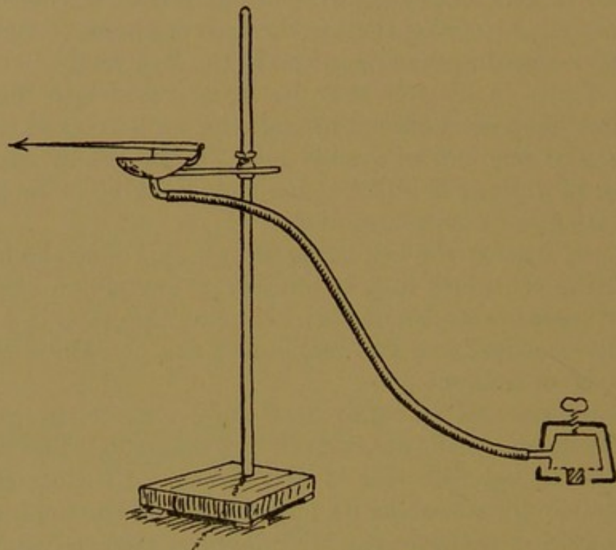
FIG. 107.—Cardiograph consisting of a Receiving Tambour, with a button on the Membrane which is placed upon the Cardiac Impulse, and a Recording Tambour connected with a Lever.
