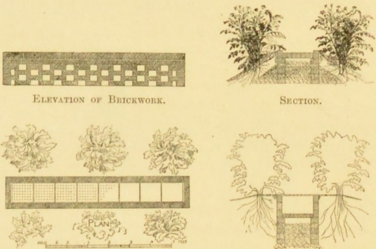
FIG. 27.—FILTRATION GUTTER ON BANK.
