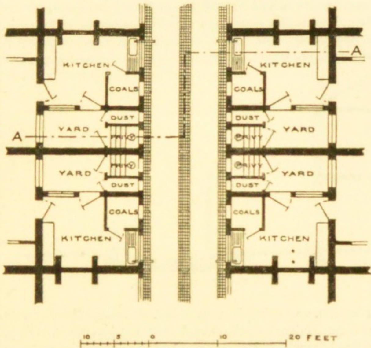
FIG. 29.—ARRANGEMENT FOR SMALL TENEMENTS.
