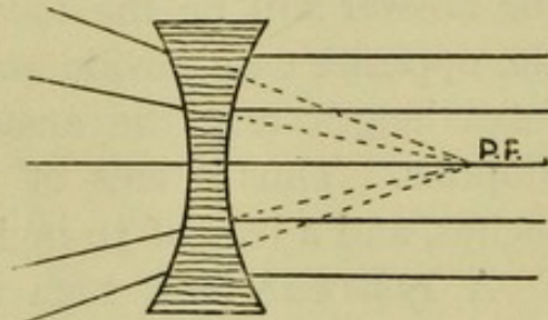
FIG. 9.—Action of a concave spherical lens upon parallel rays. P.F. is the (negative) principal focus.
