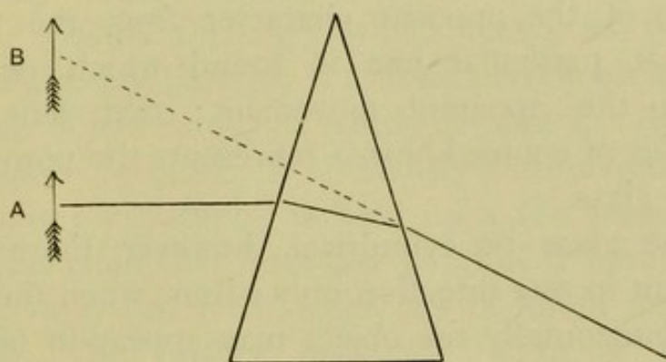
FIG. 10.—Action of a prism.
