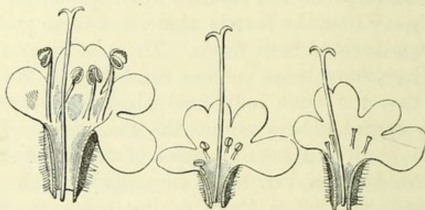
Hermaphrodite.
