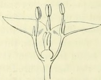
Long-styled male.
