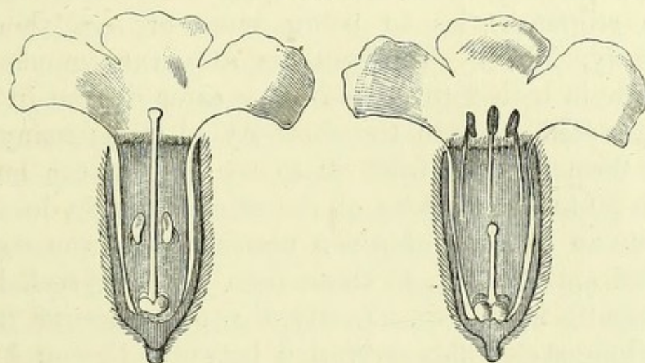
Long-styled form.
