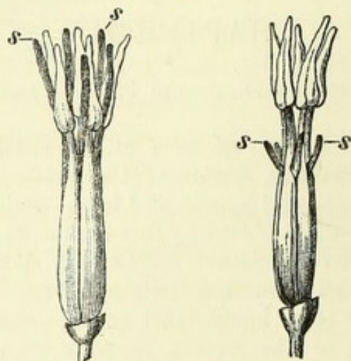
Long-styled form.
