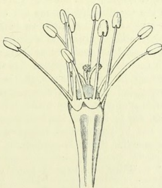
Short-styled form.
