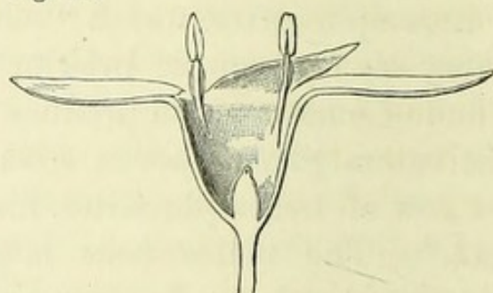
Short-styled male.
