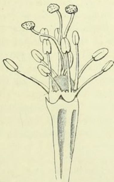
Long-styled form.
