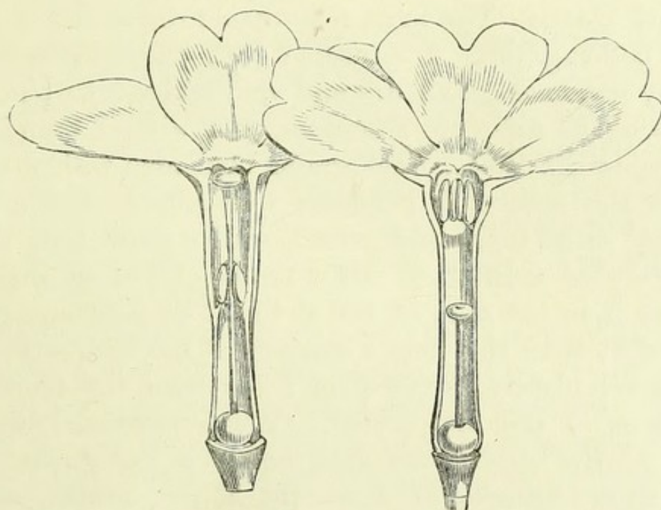
Long-styled form.
