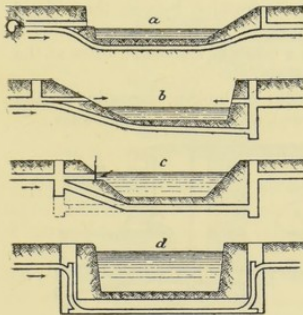
FIG 52.—INVERTED SIPHONS.
