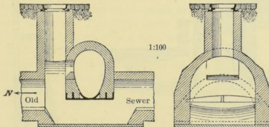
FIG. 41.—INTERSECTION OF SEWERS, BERLIN.
