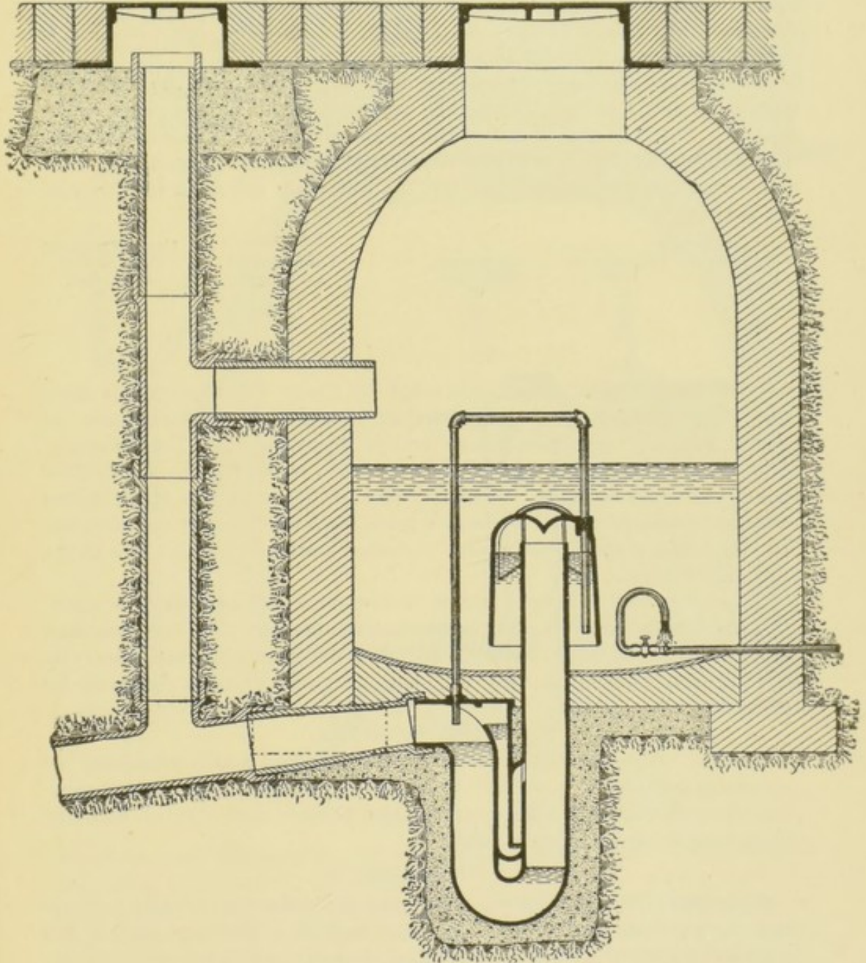
RHOADS-WILLIAMS SIPHON.
