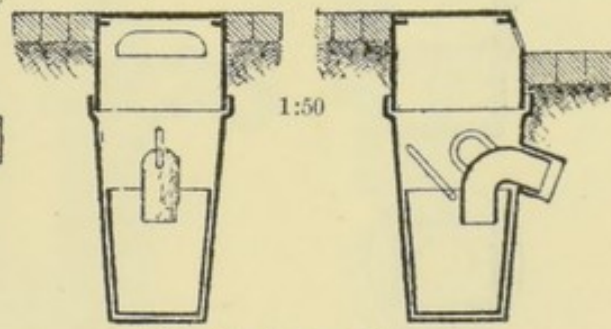
FIG. 66.—STREET INLET AT WIESBADEN.
