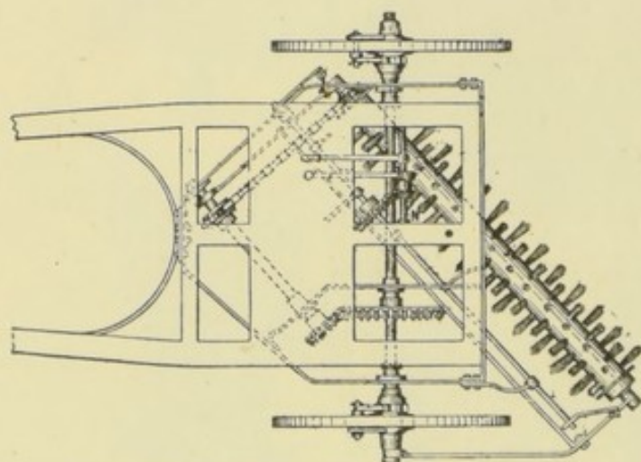
FIG. 213.—STACKPOLE STREET SWEEPER.
