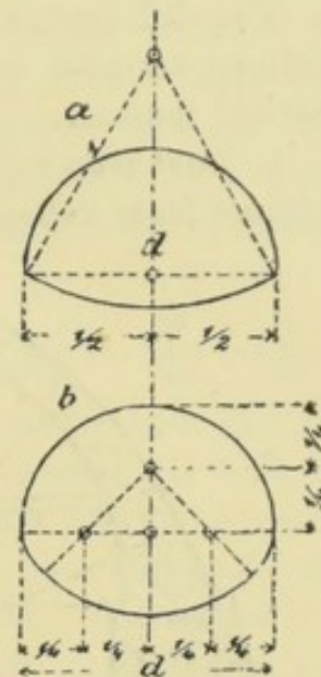
FIG. 14.—ENGLISH SECTIONS.
