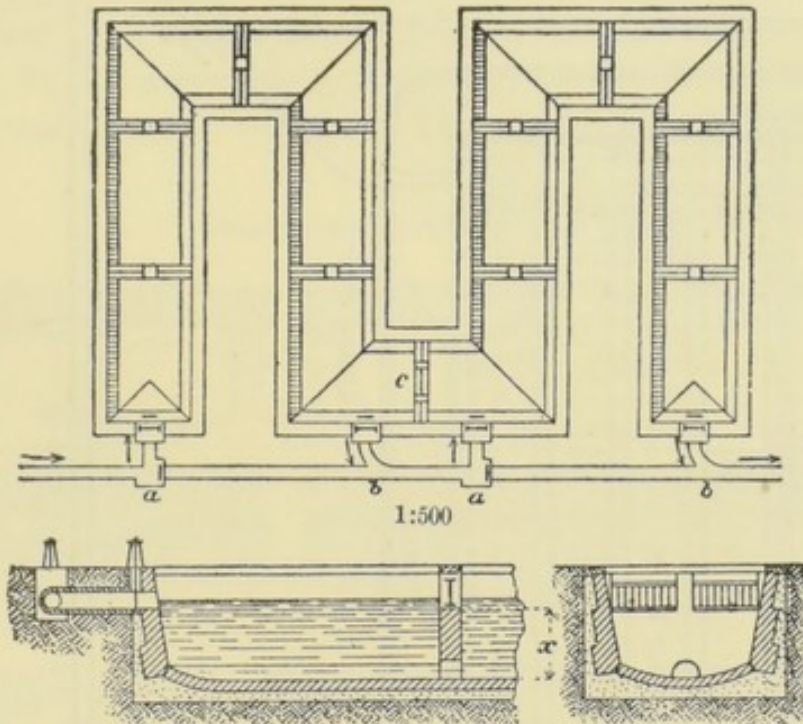
FIG. 131.—PRECIPITATING TANK AT TUNBRIDGE WELLS.
