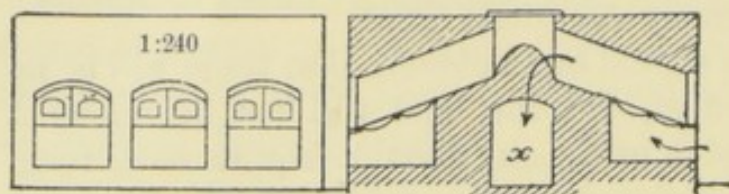
FIG. 154.—GARBAGE FURNACE.
