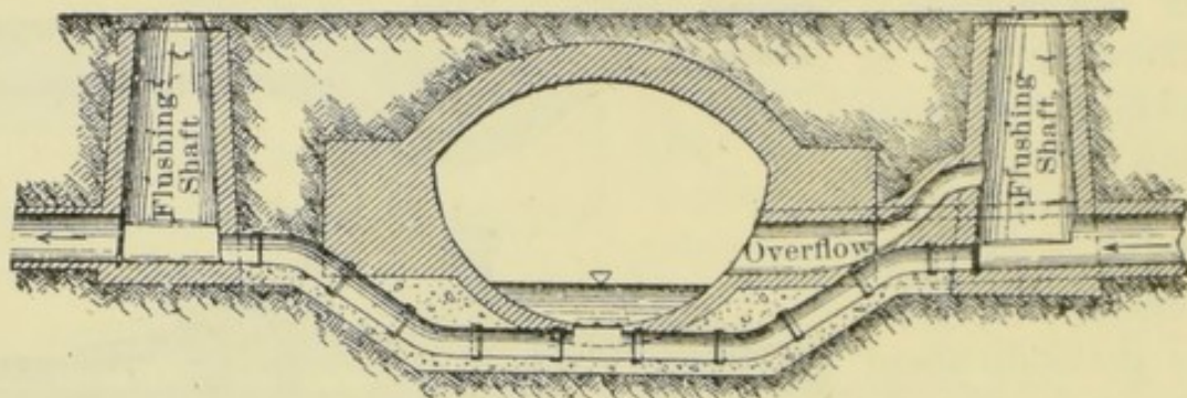
FIG. 51.—INVERTED SIPHON AT WIESBADEN.
