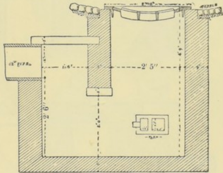
FIG. 192.—ALLEY AND GUTTER DROP.
