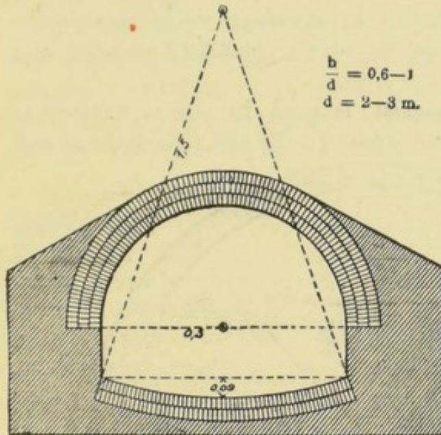
FIG. 13.—SECTION OF BERLIN SEWERS.
