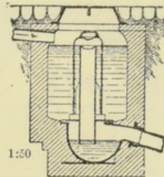
FIG. 96.—FLUSHING TANK, SYSTEM BOECKING.
