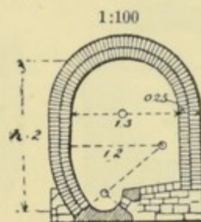
FIG. 6.—SECTION IN WIESBADEN; h = 2 meters.
