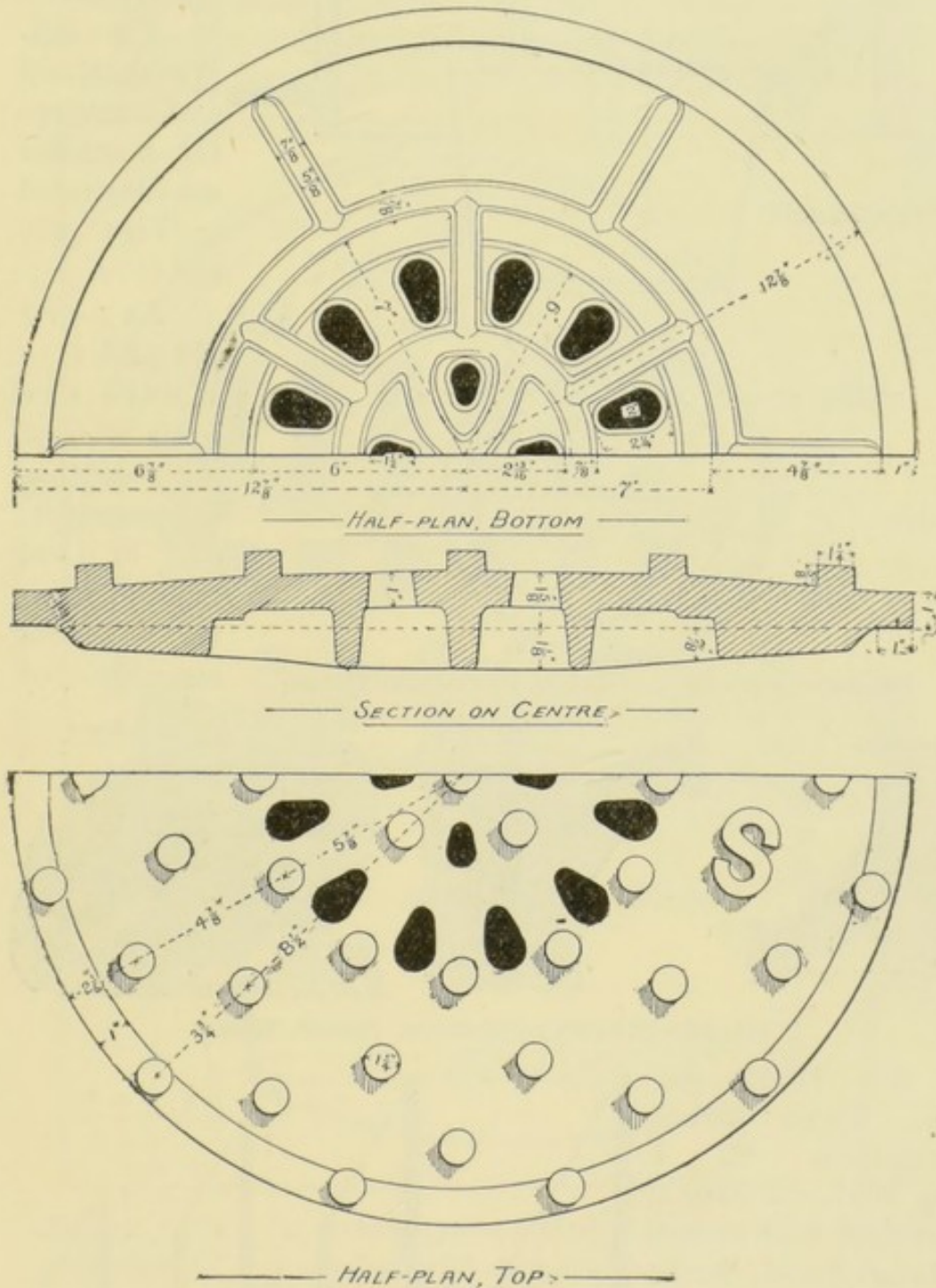
FIG. 199.—VENTILATED MANHOLE COVER.
