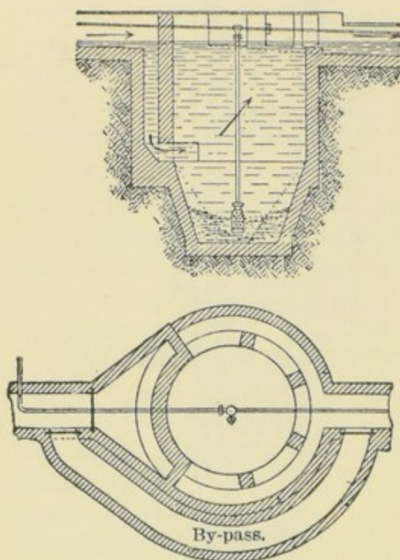
FIG. 136.—PRECIPITATION TANKS IN HALLE, MUELLER-NAHNSEN SYSTEM.
