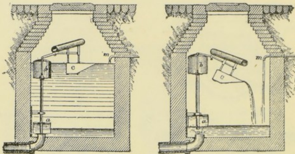
FIG. 99.—FLUSHING TANKS, SYSTEM FRUEHLING.
