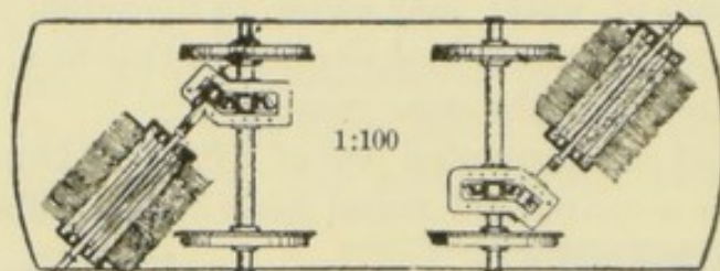
FIG. 160.—TRAMWAY SWEEPER.
