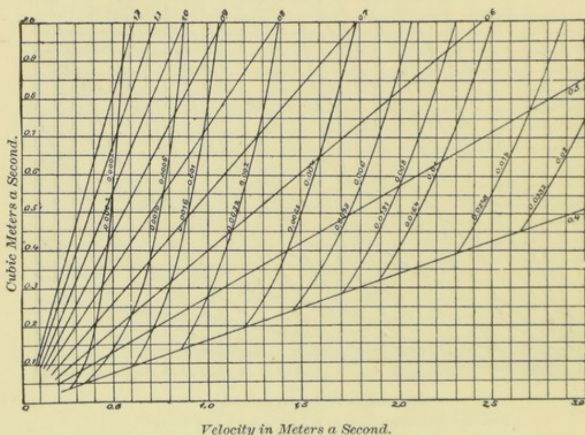
FIG. 26.—GENERAL DIAGRAM FOR EGG SECTIONS.
