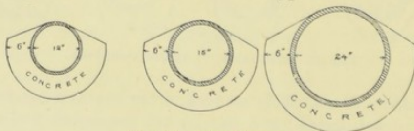
FIG. 198a.—PIPE SEWERS.
