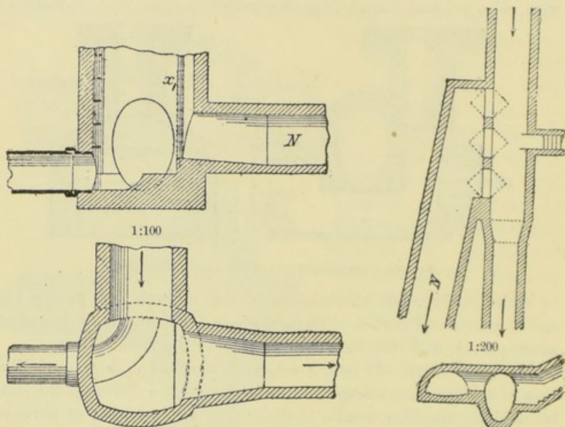
FIG. 45.—RELIEF OUTLET WITH FLASHBOARDS.
