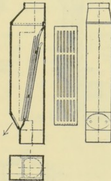
FIG. 75.—GRATINGS IN RAIN PIPES.
