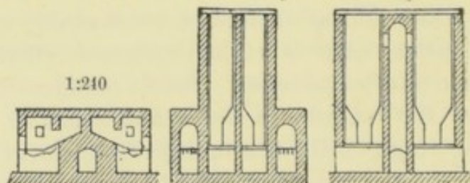
FIG. 155.—CHARRING FURNACE.
