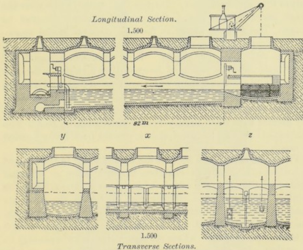
FIG. 134.—SECTIONS OF THE CLEARING BASINS.
