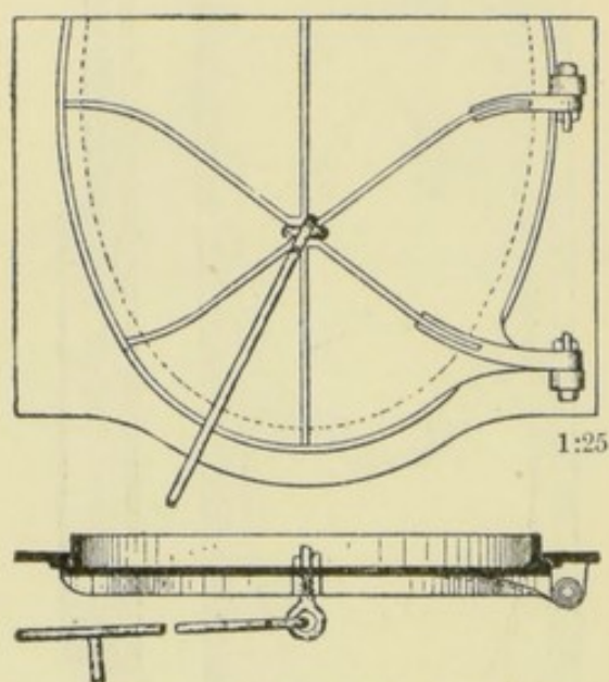
FIG. 88.—FLUSHING GATE AT HAMBURG.
