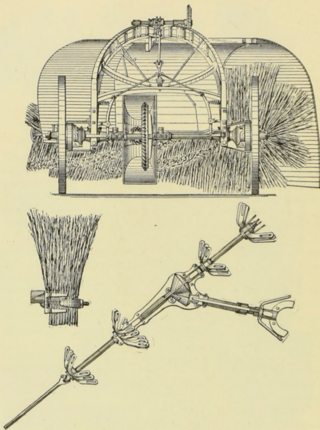
FIG. 215.—STREET SWEEPER, WASHINGTON, D. C.
