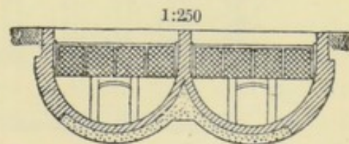
FIG. 132.—SECTION OF PRECIPITATION TANKS, DORTMUND.
