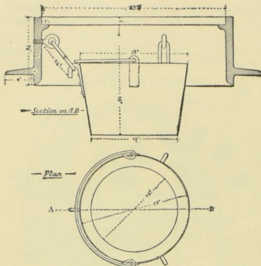
FIG. 200.—CATCH-BUCKET UNDER VENTILATED COVER.
