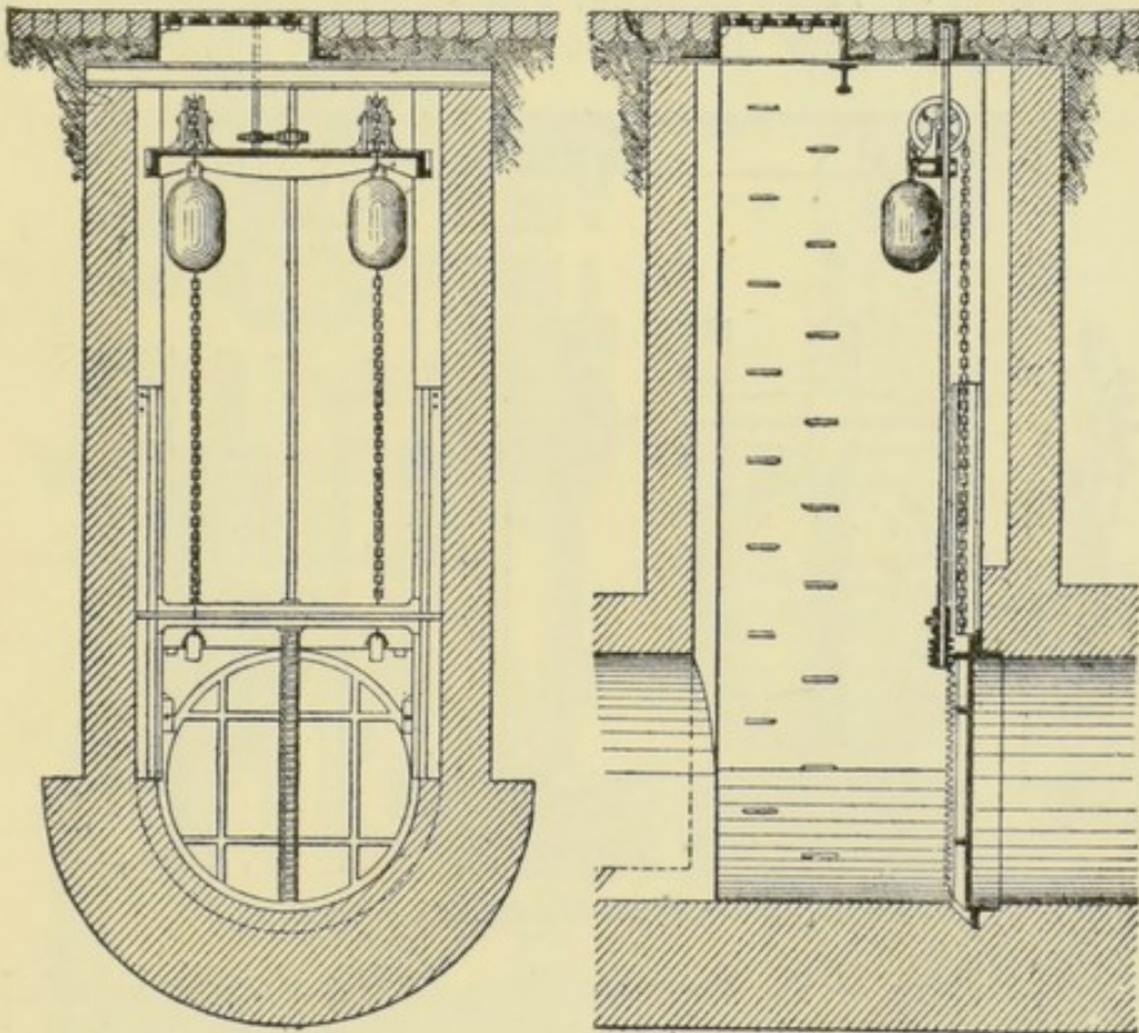
FIG. 93.—FLUSHING PENSTOCK.
