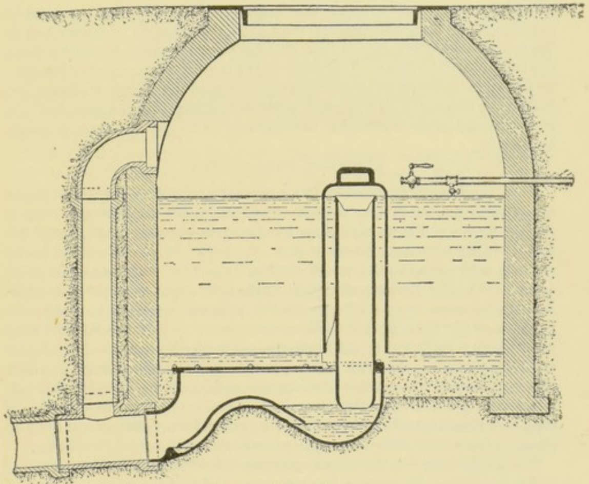
ROGERS FIELD SIPHON.
