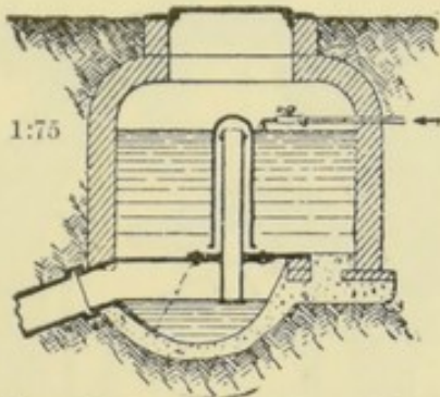
FIG. 95.—FLUSHING TANK, FIELD SYSTEM.
