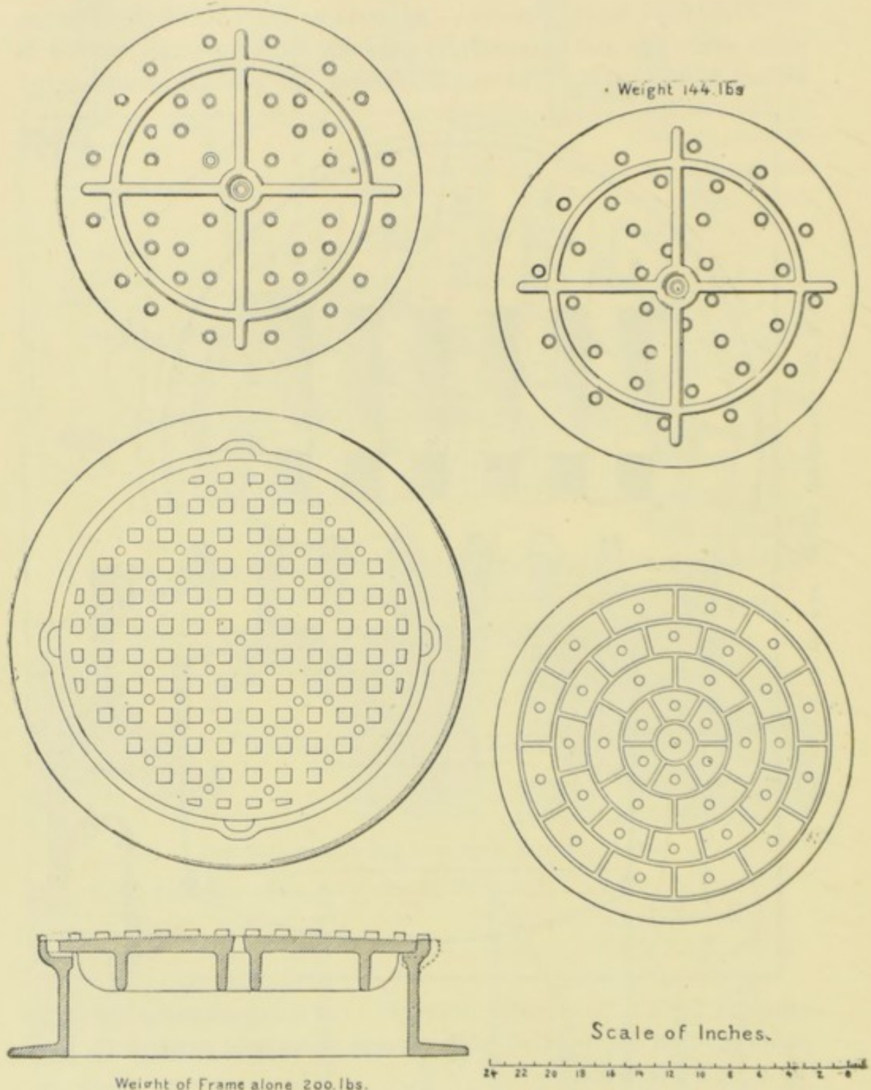
FIG. 202.—KNOBBED MANHOLE COVER.
