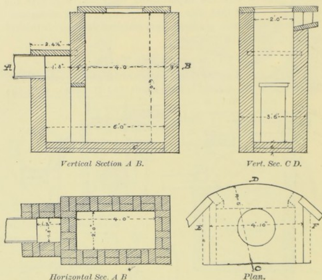
FIG. 191.—CATCH BASIN, WASHINGTON, D. C.
