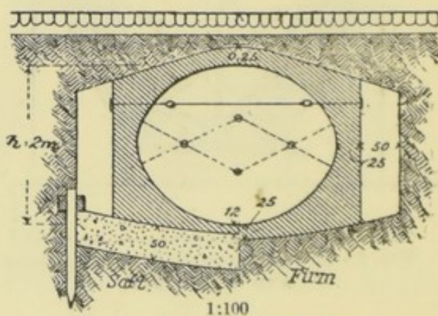
FIG. 12.—SEWER SECTION, BREMEN.
