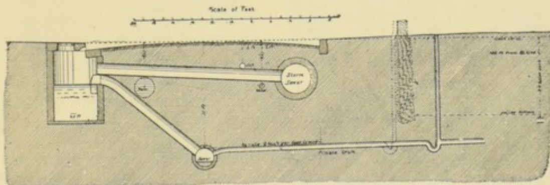
FIG. 212.—SECTION ILLUSTRATING DRAINAGE.
