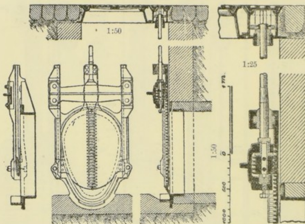
FIG. 91.—FLUSHING GATE, GEIGER SYSTEM.
