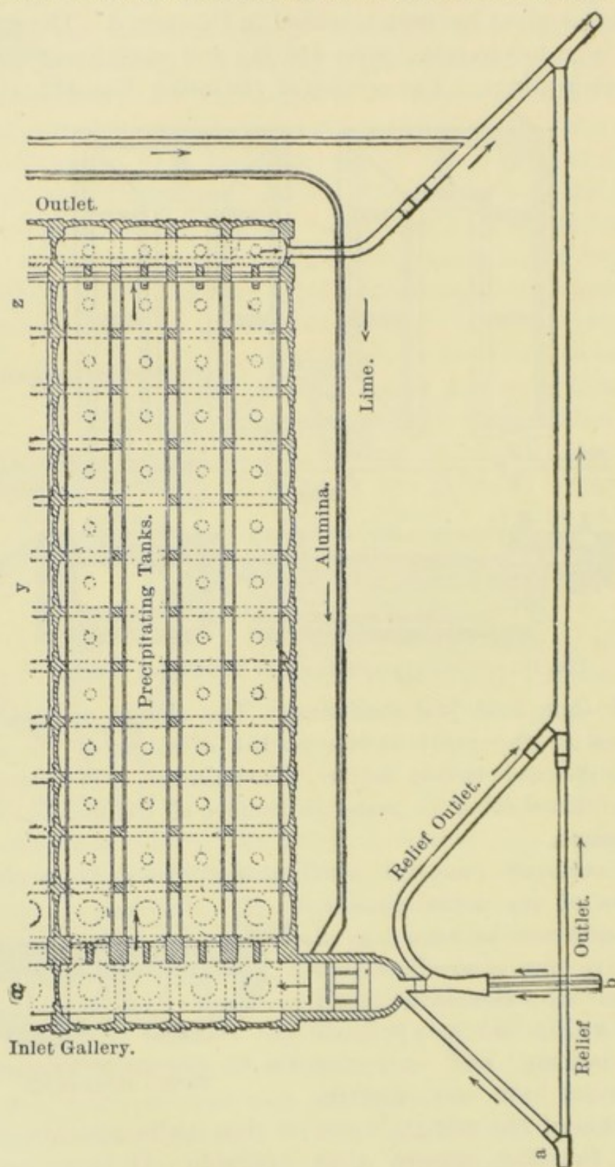
FIG. 133.—PRECIPITATION TANKS IN FRANKFURT. 1:1000
