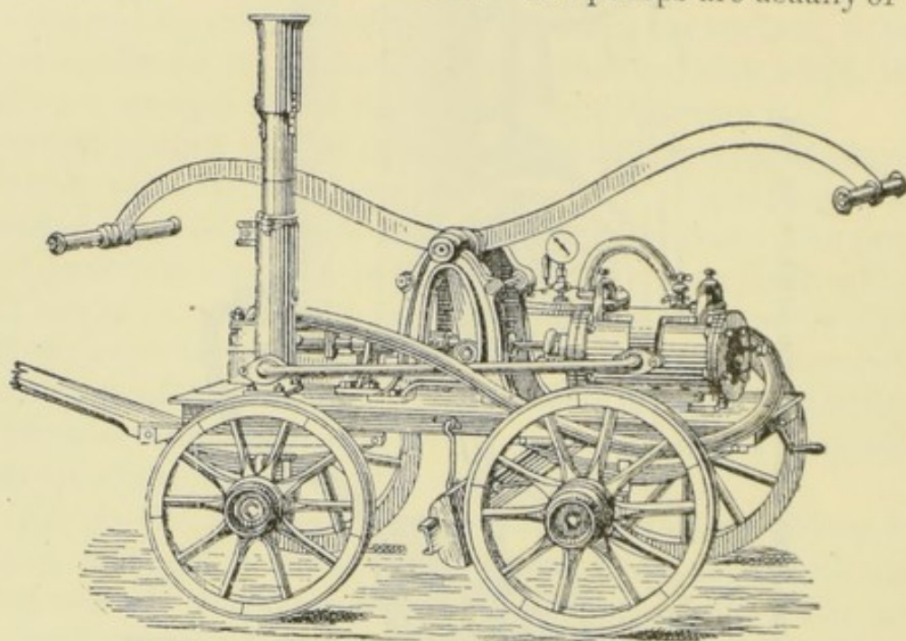
FIG. 165.—CESSPOOL PUMP.
