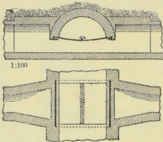
FIG. 49.—INTERSECTION OF SEWERS, BERLIN.
