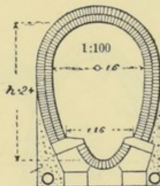
FIG. 7.—SECTION IN STUTTGART; h = 2.4 meters.
