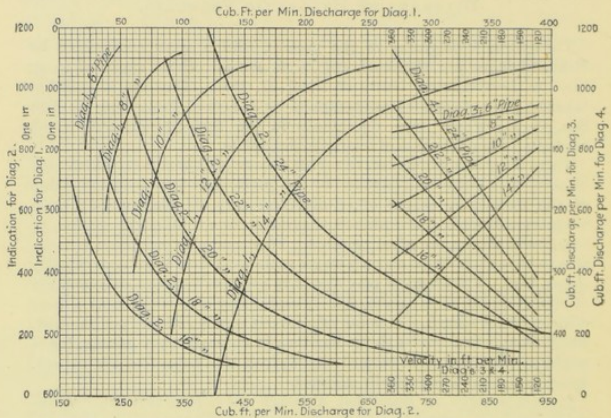
PLATE 1. DISCHARGE AND VELOCITY OF FLOW IN 6 TO 24 IN. PIPE SEWERS.
