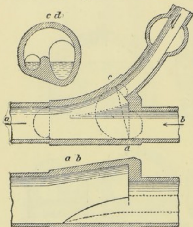
FIG. 38.—INTERSECTION OF CONCRETE SEWERS, HEIDELBERG.
