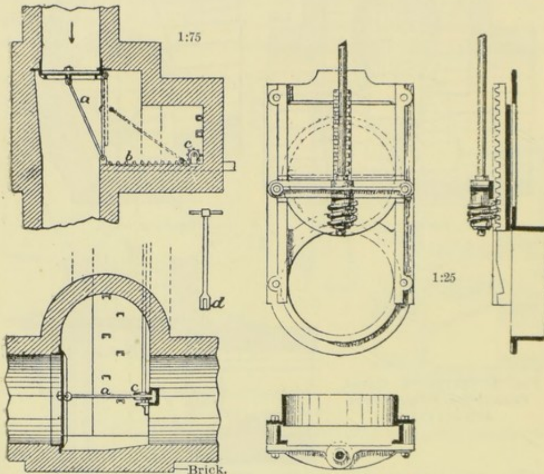
FIG. 91.—FLUSHING GATES, DANZIG.
