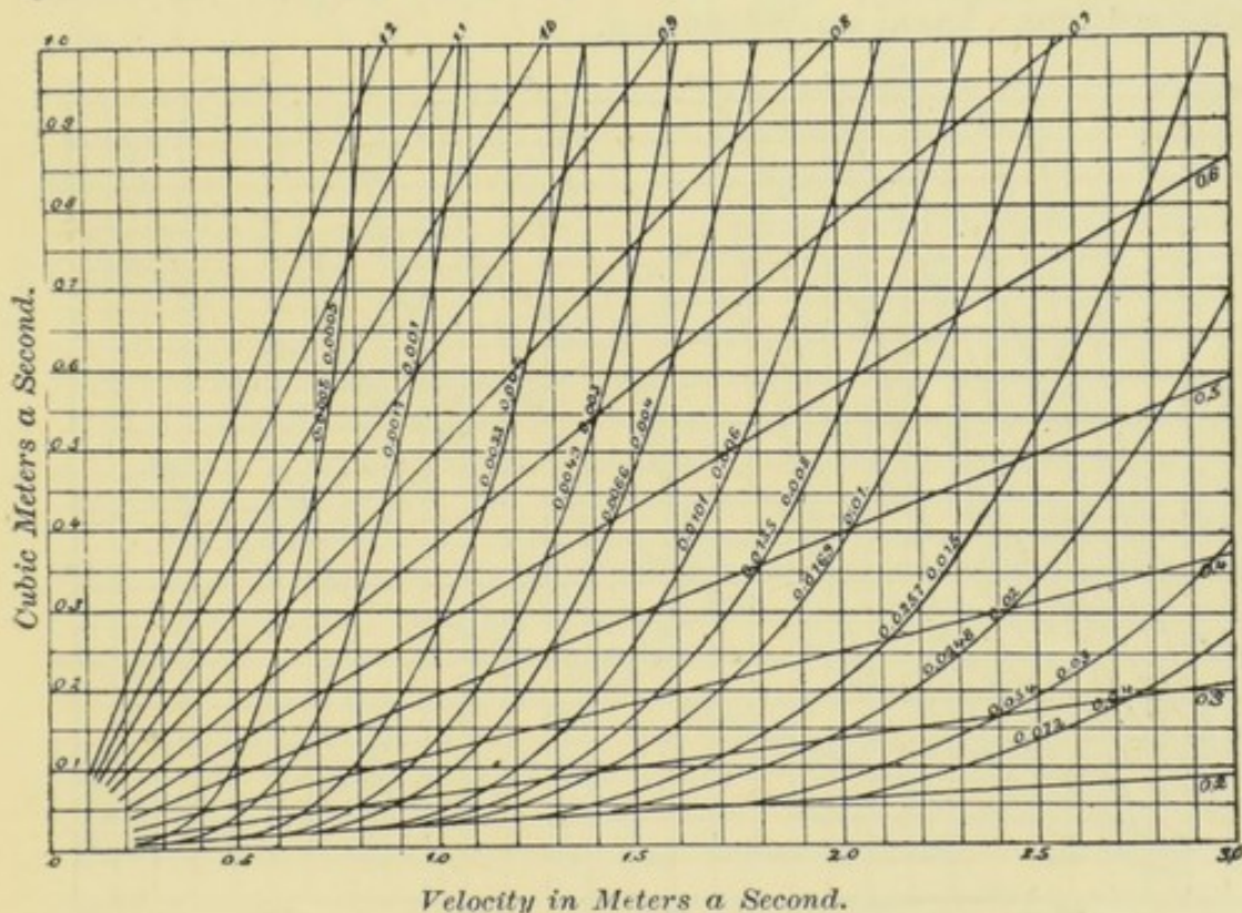
FIG. 25.—GENERAL DIAGRAM FOR CIRCULAR SECTIONS.
