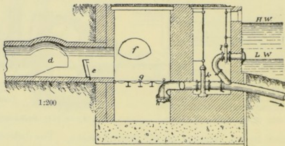
FIG. 55. - INLET TO INVERTED SIPHON.
