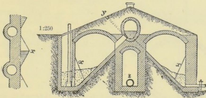
FIG. 129.—PRECIPITATION CHAMBERS, SYSTEM PARJE.
