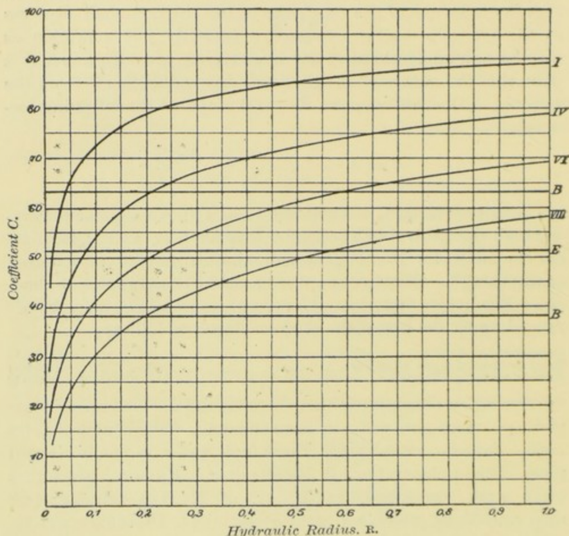
FIG. 24.—DIAGRAM GIVING VALUES OF C IN FORMULA FOR FLOW OF WATER.
