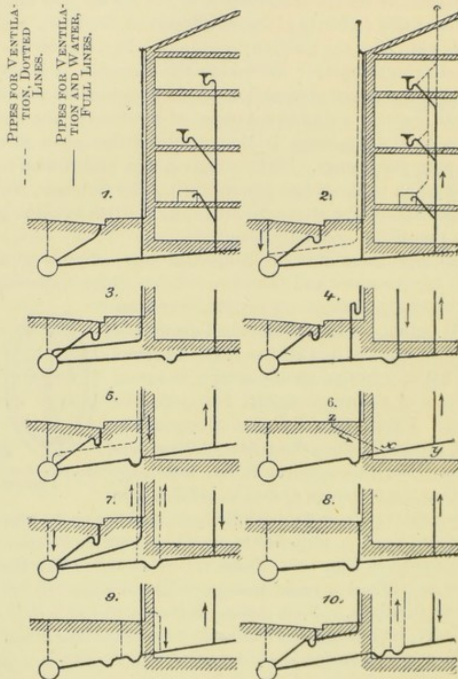
FIG. 104.—DIAGRAMS OF HOUSE CONNECTIONS.
