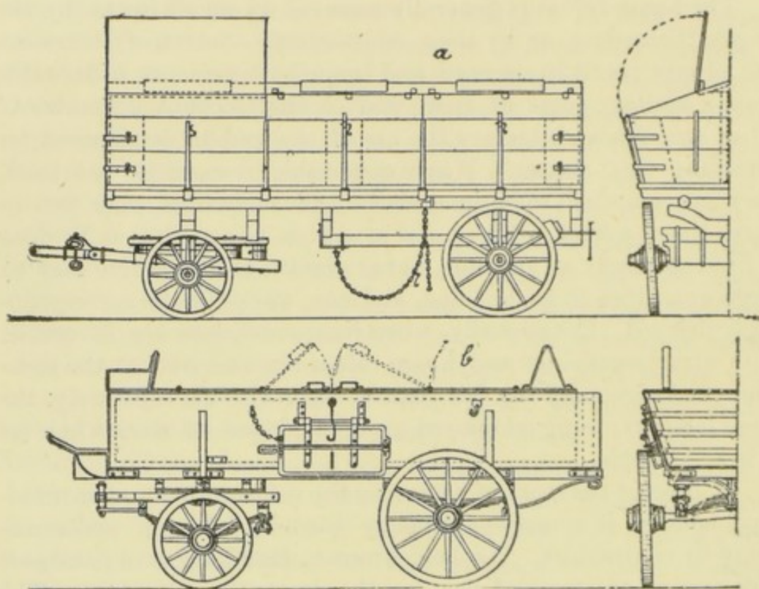
FIG. 152. — GARBAGE WAGONS.
