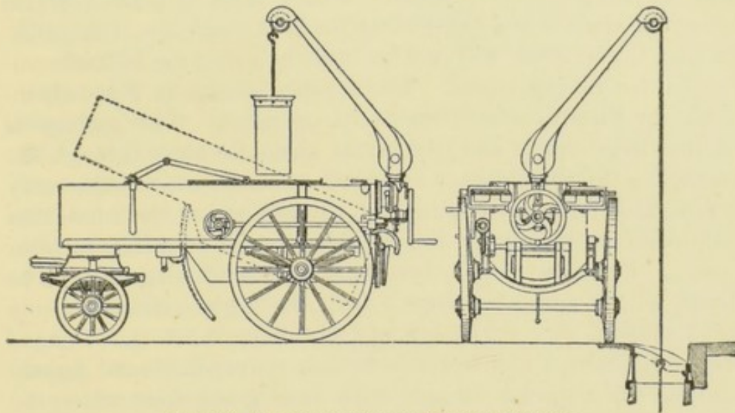
FIG. 153.—GARBAGE WAGON, GEIGER SYSTEM.
