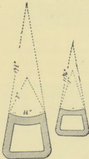
FIG. 208.—INVERT BLOCK.
