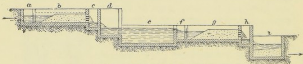
FIG. 143.—PRECIPITATION TANKS, PETRI SYSTEM.
