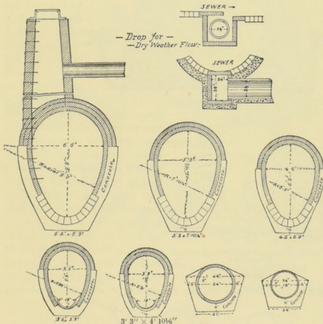
FIG. 197.—STANDARD SEWERS, WASHINGTON.
