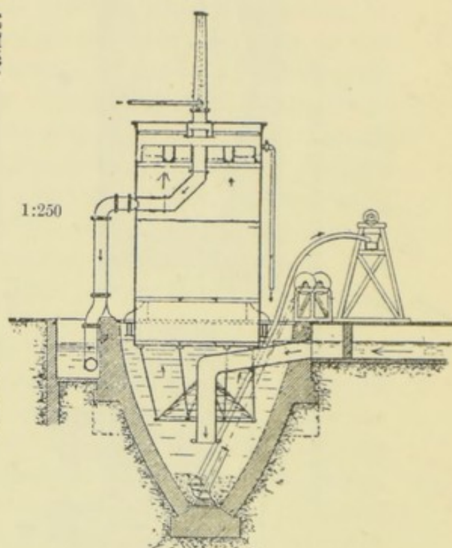
FIG. 137.—UPRIGHT TANKS, ROECKNER-ROTHE SYSTEM.
