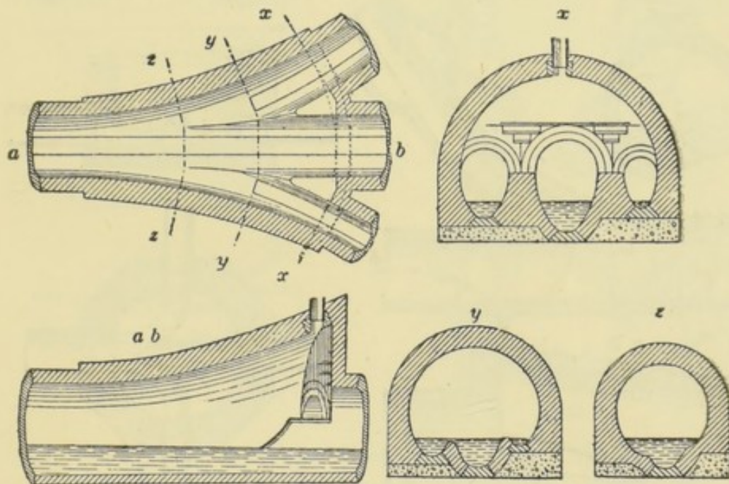
FIG. 37.—INTERSECTION OF BRICK SEWERS, FRANKFURT.
