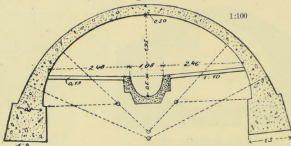
FIG. 16.—SEWER SECTION IN ALTENBERG.—DIMENSIONS IN METERS.
