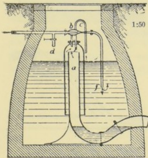
FIG. 97.—FLUSHING TANKS, CUNTZ SYSTEM.
