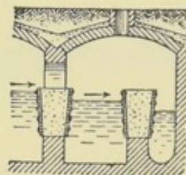
FIG. 142.—FILTERS AT COVENTRY. 1:250
