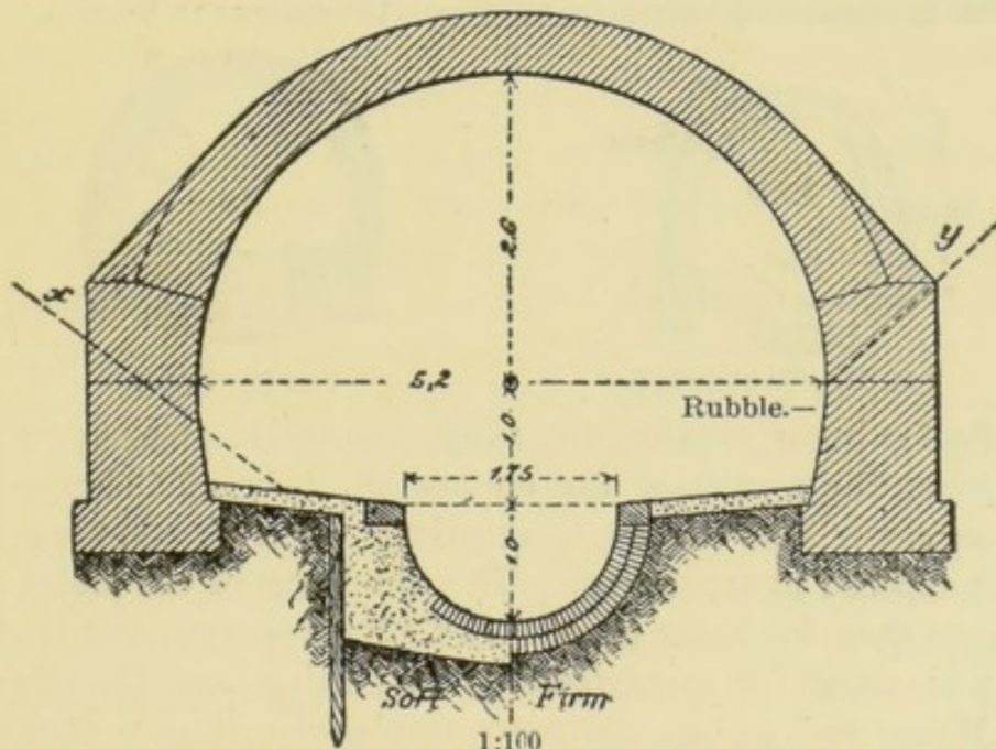
FIG. 15.—SEWER SECTION IN KARLSRUHE.—DIMENSIONS IN METERS.
