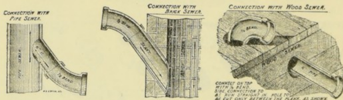
FIG. 203.—SEWER CONNECTIONS, BOSTON, MASS.
