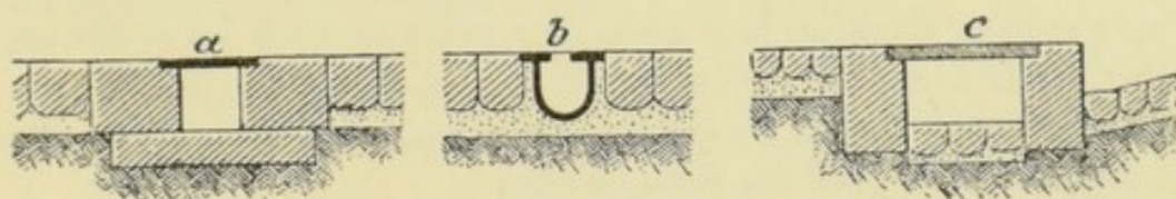
FIG. 145.—SECTIONS OF GUTTERS.
