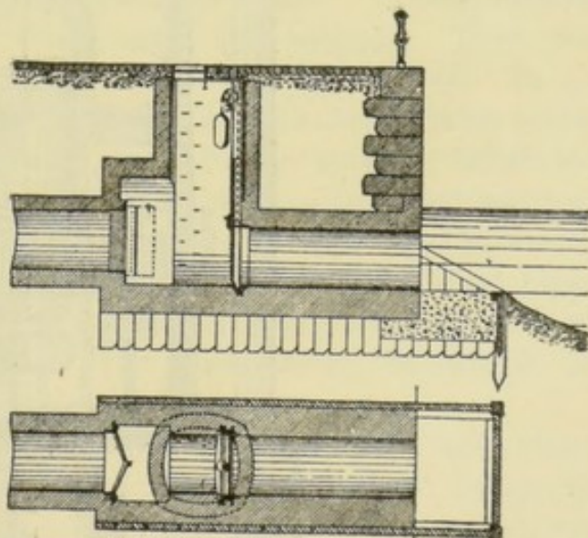
FIG. 114 a .—RELIEF OUTLET AT HAMBURG.
