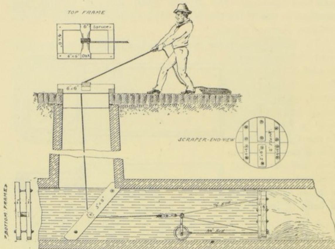
FIG. 211.—SMALL SEWER FLUSHING.
