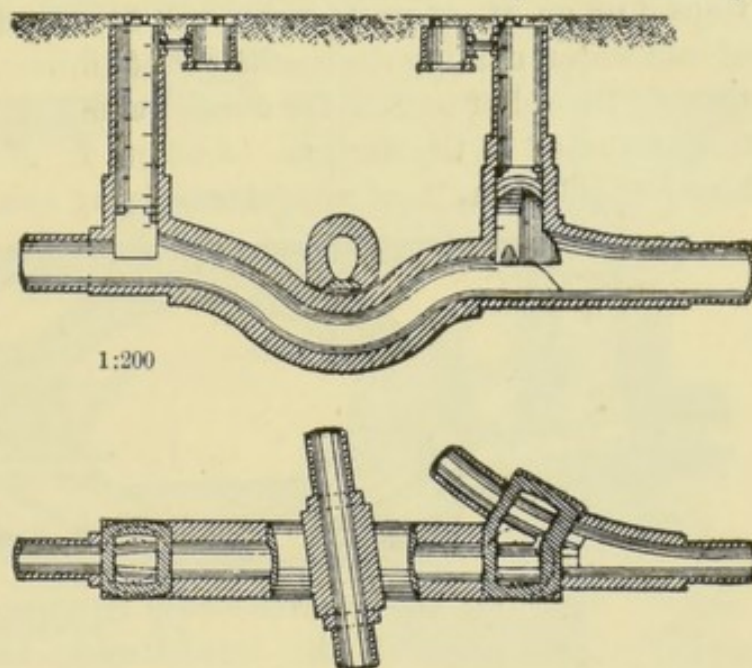
FIG. 50.—SEWER INTERSECTIONS AT FRANKFURT.
