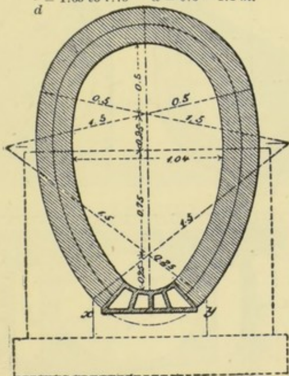
FIG. 5.—SEWER SECTIONS, MAINZ, COLOGNE AND WIESBADEN.
