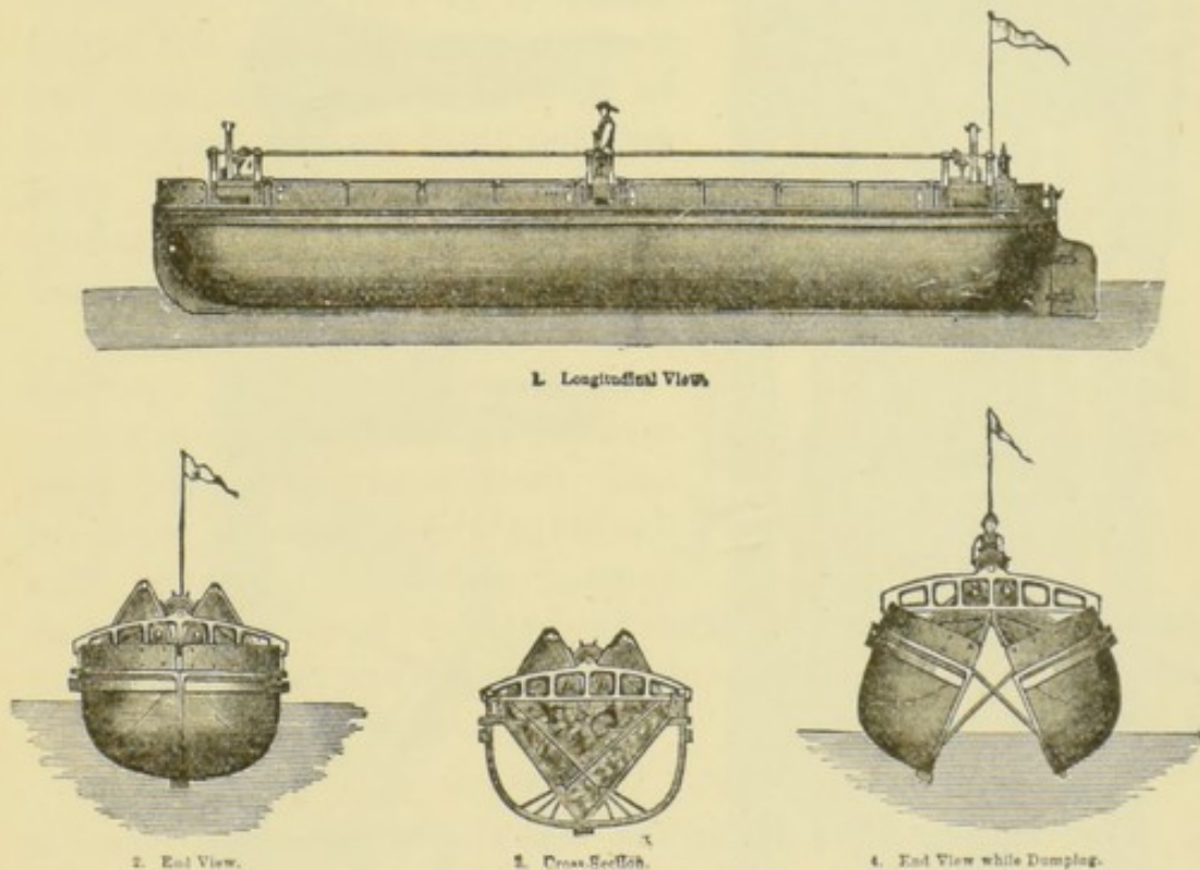
FIG. 220.—BARNEY DUMPING SCOW.
