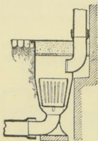
FIG. 77.—RAIN PIPE IN-LET AT ERFURT.
