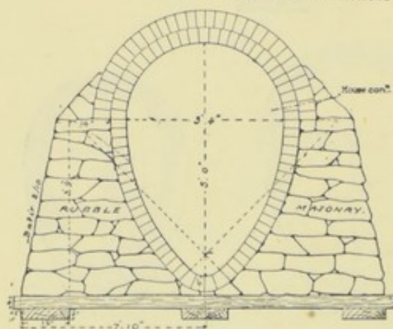
Type of Maximum Section on Artificial Foundation.
