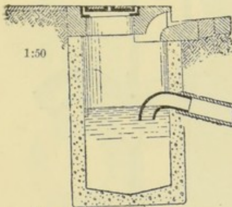
FIG. 65.—STREET INLET AT HEIDELBERG.
