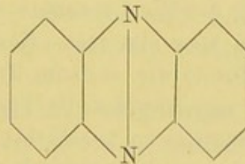
Phenazin.
