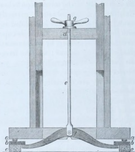
FIG. 2. Transverse section of car and track, to show the rails and the apparatus for clamping the car to the same: a a , small brass wheels, grooved; b b , flat iron rails, with \Delta -shaped projection to fit the groove in the wheels; c c , wooden rails; d , crosspiece connecting the sides of the car; e , vertical iron rod passing through the same; f , cast-iron crosspiece to clamp under the iron rails; g , screw nut, with handles, to elevate the same.
