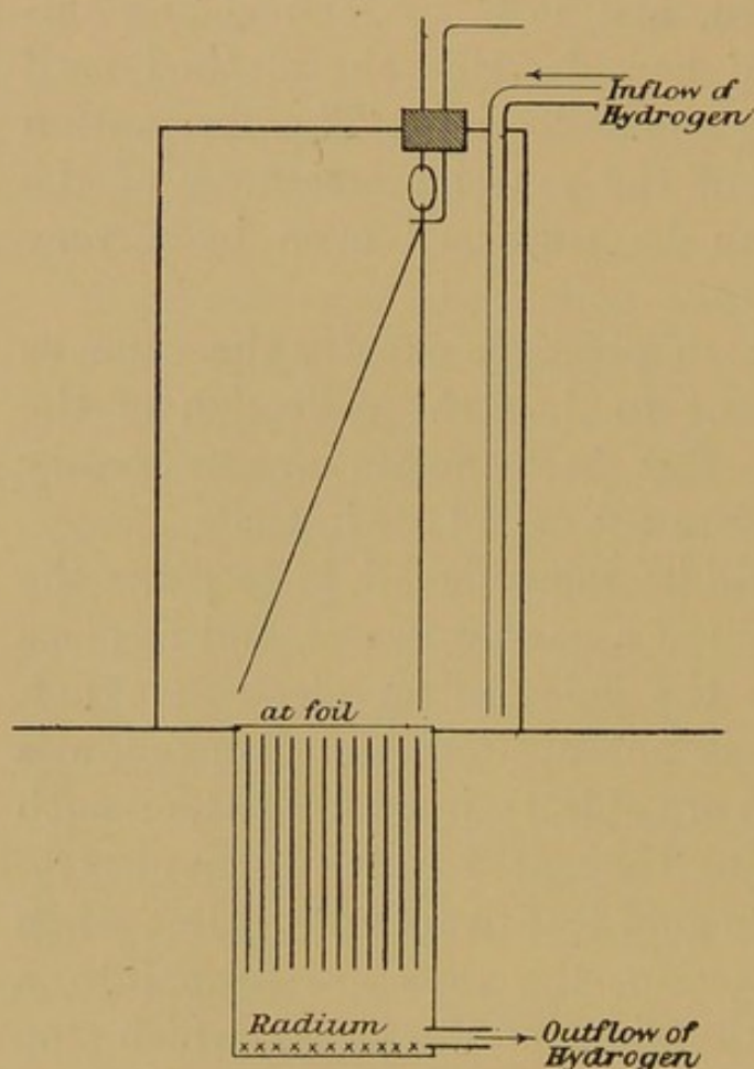
FIG. 17.—Rutherford's arrangement for observing magnetic deviation of \alpha -rays. The rays pass up between the metal slits, and enter the electroscop, causing discharge. When a magnetic field is applied perpendicular to the paper, the rays are curved, and can no longer get through the slits. Thus discharge is stopped.
