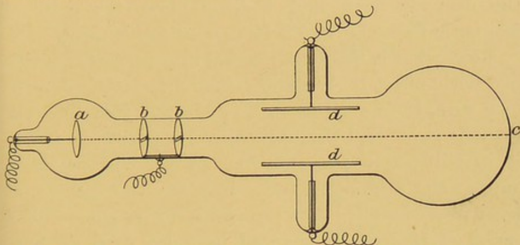
FIG. 5.—Tube for observing and measuring the magnetic and electrostatic deflection of the cathode rays. The beam of cathode rays from the flat disc, a , represented by the dotted line, is deflected by passage through the two slits in the metal discs, b b . These discs are connected to the anode. The cathode rays form a well-defined fluorescent patch on the wall at c . They can be deflected magnetically by means of flat coils of wire carrying a current, which lie on either side of the tube, in planes parallel to the paper. Electrostatic deflection is produced by the plates d d , connected to the poles of a battery.
