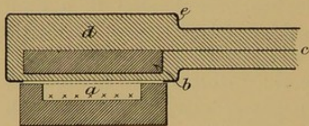
FIG. 15.—Section of Curie's apparatus for observing the charge conveyed by radium to surrounding conductors. a is the radium, contained in a cavity in a lead block. b is the block of lead which receives the rays, and becomes charged. It is entirely surrounded by paraffin wax, d . This prevents the charge acquired from leaking away. b is connected by the wire, c , to the electrometer, which indicates the charge acquired. The whole of the receiving arrangement is surrounded by a metal case, e , connected to earth, but this metal is very thin on the face where the rays enter.
