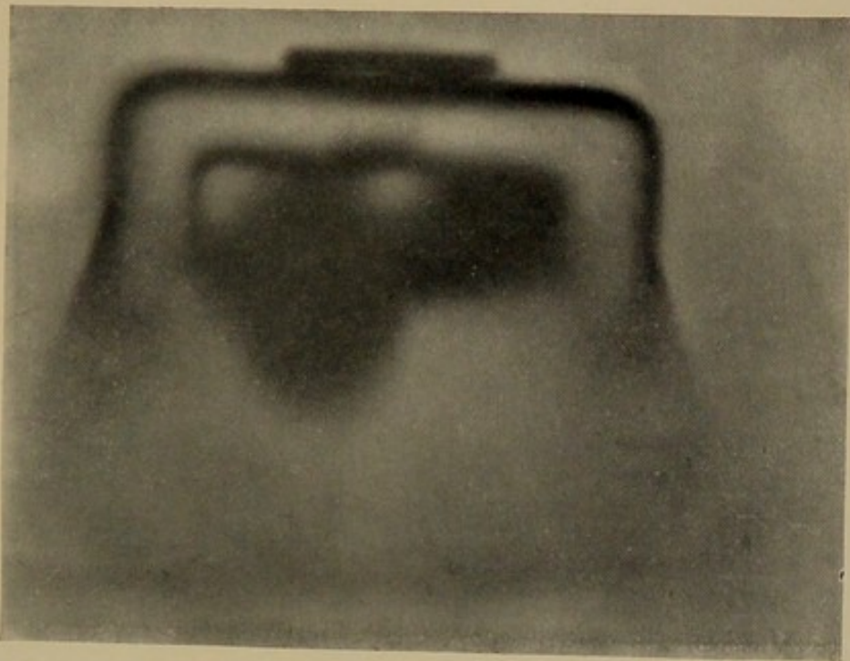
RADIOGRAPH OF A PURSE CONTAINING COINS, TAKEN BY RADIUM. THE METAL FRAME OF THE PURSE AND THE ENCLOSED COINS STOP THE RAYS MUCH MORE THAN THE LEATHER, SINCE THEY ARE DENSER. THUS IN THE POSITIVE PICTURE THEY SHOW BLACK ON A LIGHT GROUND.
