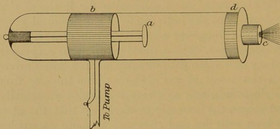
FIG. 7.—Tube for showing penetration of the cathode rays into the open. a is the disc-shaped cathode; a metal tube, b , serves as anode. Opposite the cathode is the thin aluminium window, c , carried by the brass cap, d . The rays issue from this window.
