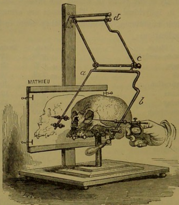
FIG. 31.—Stereograph of M. Broca. The skull is placed on the craniophore in the position shown in the drawing. The same support, if turned, serves for the views in front and behind. A special support is substituted when we wish to have drawings according to the norma verticalis of the superior or inferior surface of the skull.
