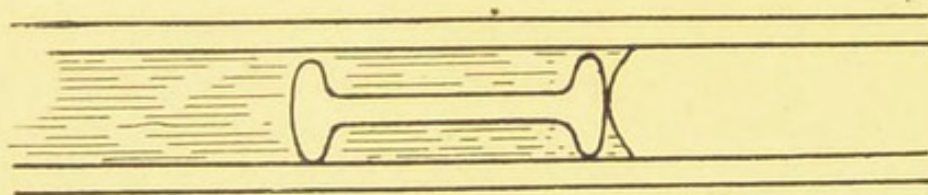
FIG. 2.—Column and index of minimum thermometer.
