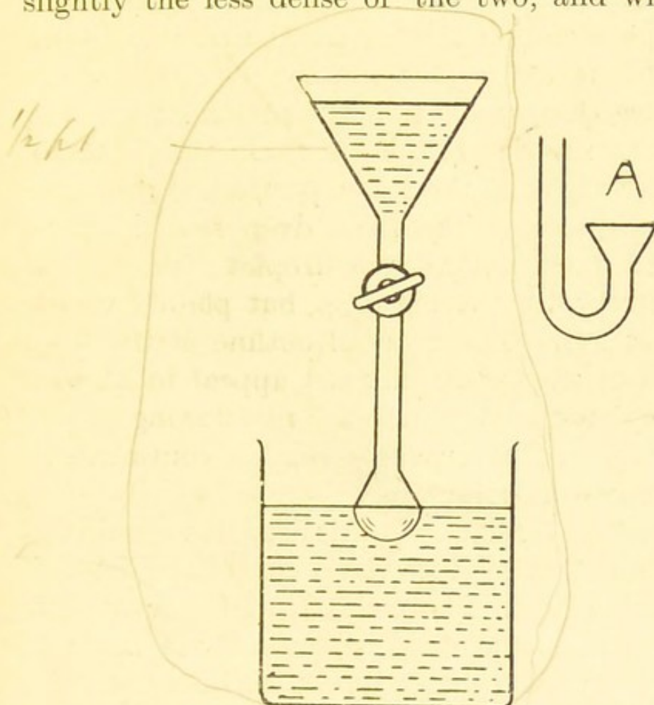
FIG. 13.—Apparatus for forming ascending or descending drops of liquids.
