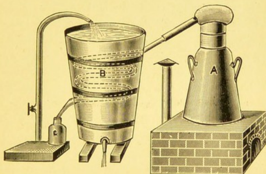
FIG. 21.—A, copper alembic; B, condenser; C, receiver.
