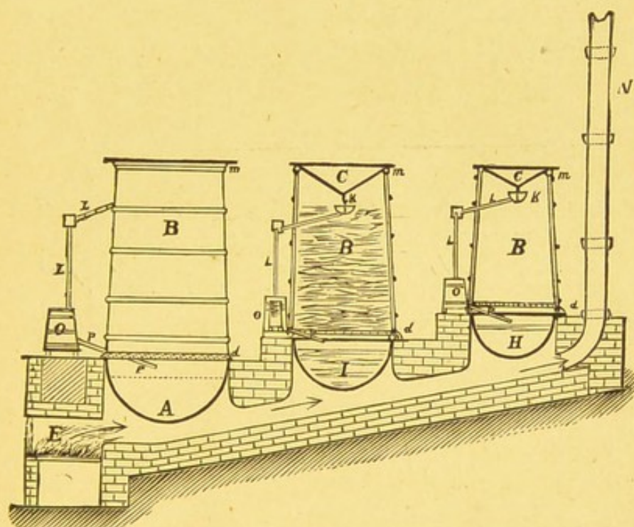
FIG. 18.—Peppermint Stills (section).
