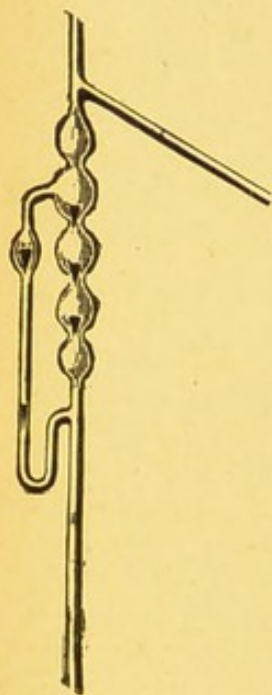
FIG. 11. Fractionating Columns.
