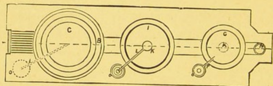
FIG. 19.—Peppermint Stills (ground plan).
