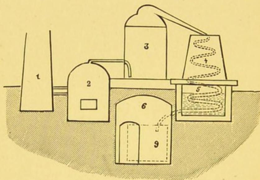
FIG. 14.—Citronella Oil Still.
