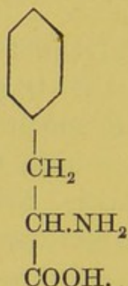
Phenyl alanin.
