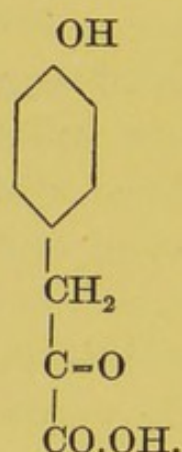
Paroxy-phenyl-pyruvic acid.
