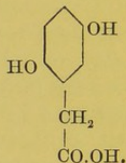
Homogentisic acid
