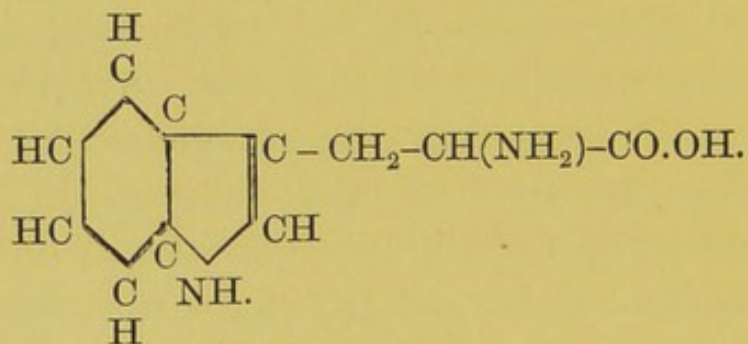
Tryptophane.
