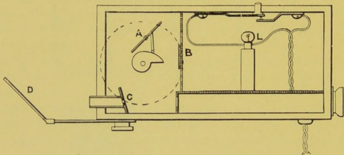
FIG. 169.—EVERETT-EDGCUMBE LUXOMETER.
