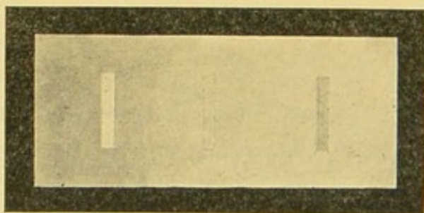
FIG. 79.—SLOT PHOTOMETER, WITH CENTRAL SLOT IN BALANCE.
