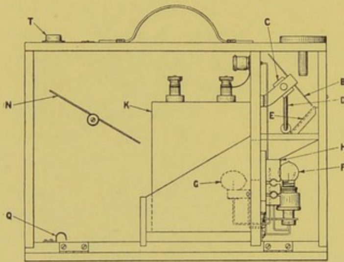
FIG. 159.—THE HARRISON PHOTOMETER, SIDE VIEW OF INTERIOR.
