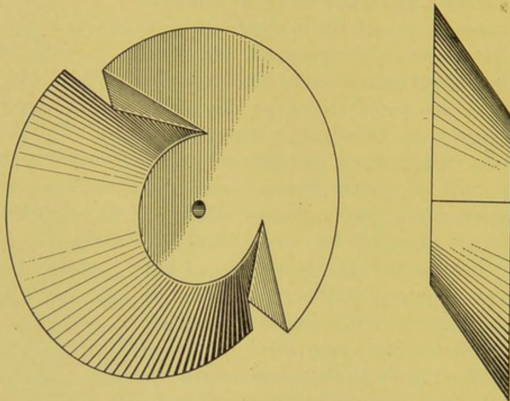
FIG. 126.—WHITMAN'S DISC FOR FLICKER PHOTOMETER.
