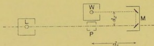
FIG. 91.—THE MOVING-MIRROR METHOD.
