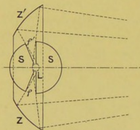
FIG. 114.—BLONDEL'S ANNULAR ELLIPSOIDAL LUMENMETER.
