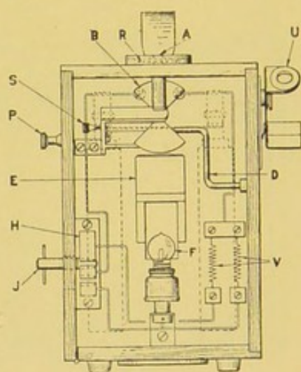
FIG. 158.—THE HARRISON PHOTOMETER, END VIEW OF INTERIOR.
