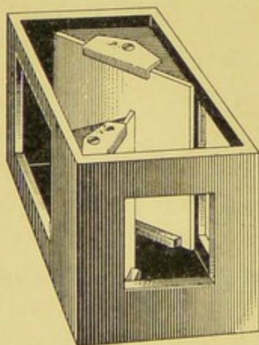
FIG. 71.—THE CONROY PHOTOMETER, PERSPECTIVE VIEW.
