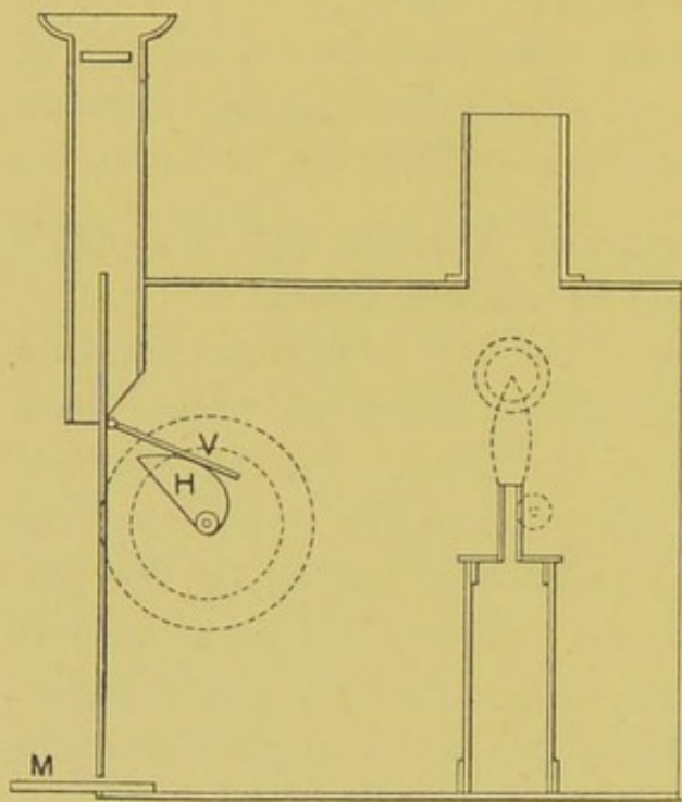
FIG. 166.—THE WINGEN-KRÜSS PHOTOMETER.
