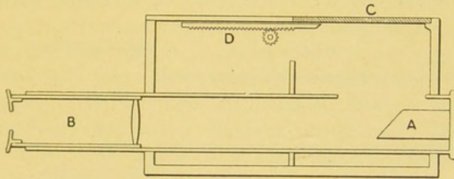
FIG. 53.—HOUSTON AND KENNELLY'S PHOTOMETER.
