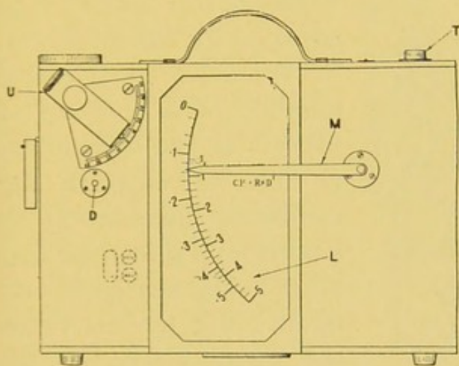
FIG. 157.—THE HARRISON PHOTOMETER, OUTSIDE VIEW.
