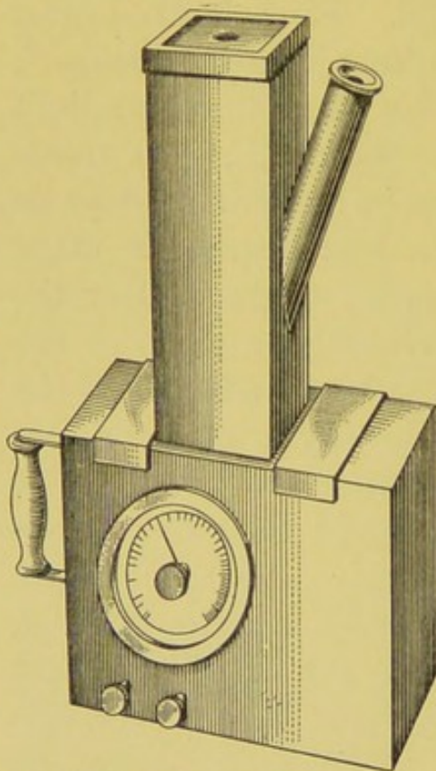
FIG. 170.—TROTTER PHOTOMETER WITH DAYLIGHT ATTACHMENT.
