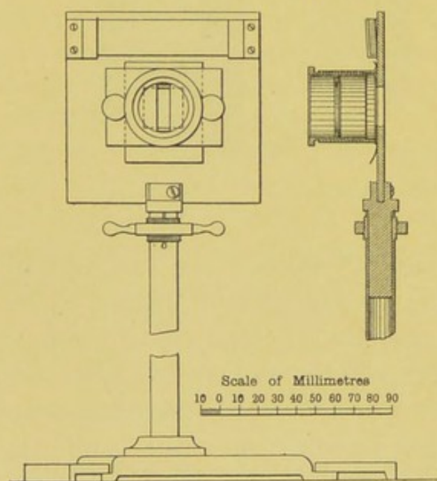
FIG. 58.—THE VERNON HARCOURT GAS REFEREES' PHOTOMETER.
