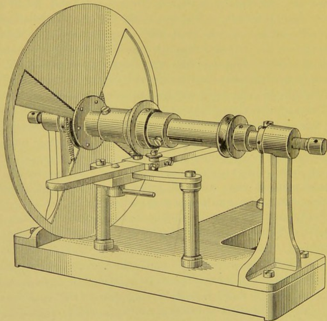
FIG. 93.—THE ABNEY SECTORS.
