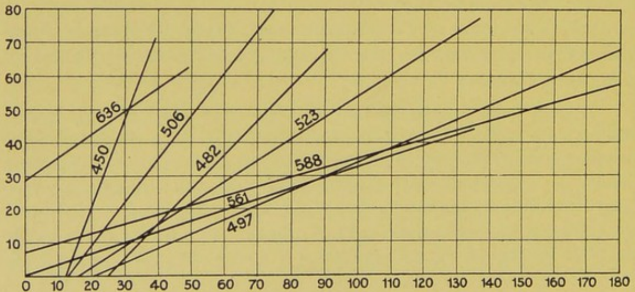
FIG. 123.—WAVE LENGTHS IN HUNDRED MILLIONTHS.
