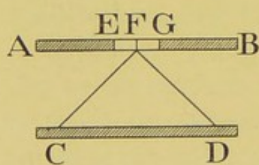
FIG. 61.—RITCHIE'S PHOTOMETER.
