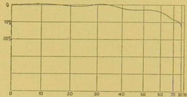
FIG. 164.—SHARP AND MILLAR TEST-PLATE ANGLE ERRORS.
