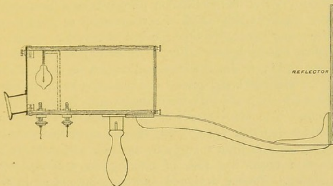
FIG. 134.—THE PREECE ILLUMINATION PHOTOMETER.
