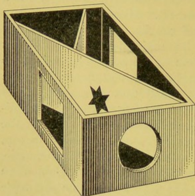
FIG. 75.—THE PERFORATED SCREEN PHOTOMETER.
