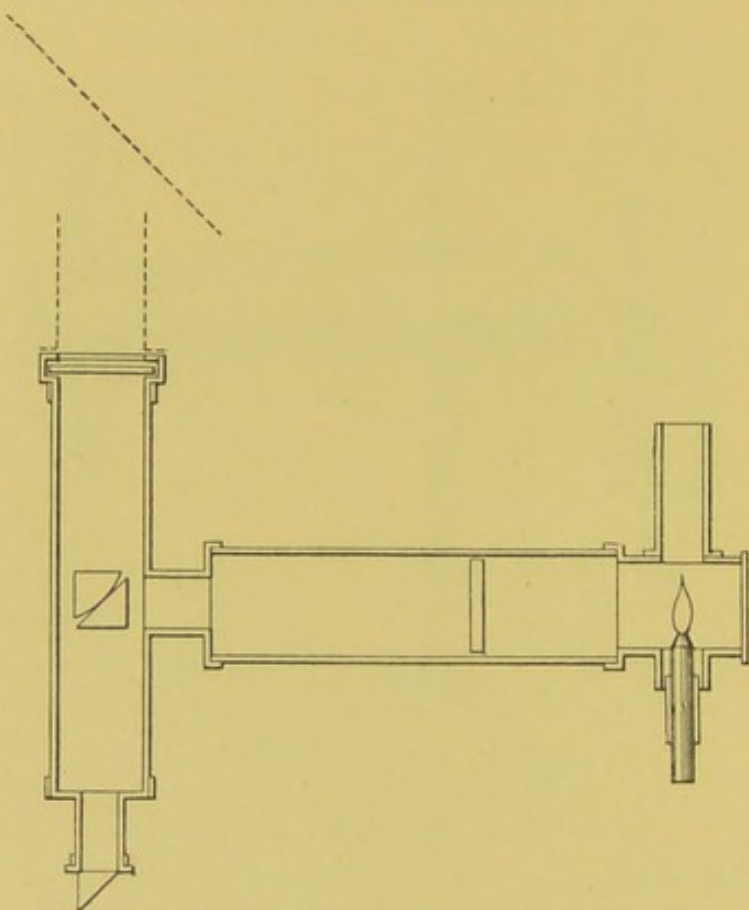
FIG. 161.—THE WEBER PHOTOMETER SECTION.
