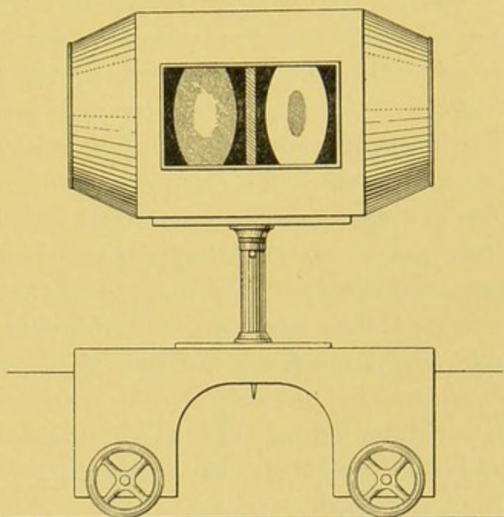
FIG. 59.—BUNSEN PHOTOMETER, FRONT VIEW, SHOWING THE SPOT OUT OF BALANCE, OWING TO THE ILLUMINATION OF THE DISC BEING GREATER ON THE RIGHT THAN ON THE LEFT.
