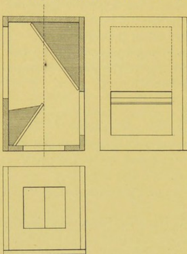
FIG. 70.—THE CONROY PHOTOMETER, PLAN AND ELEVATIONS, HALF SCALE.
