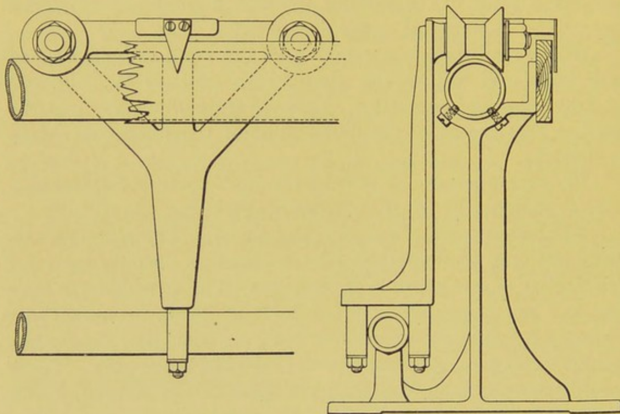
FIG. 92.—EVERETT-EDGUMBE PHOTOMETER BAR AND CARRIAGE.
