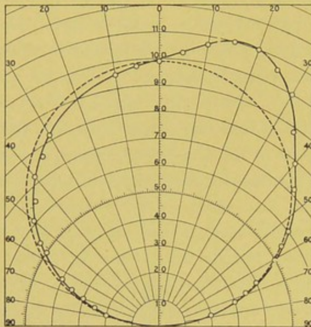
FIG. 147.—BADLY GLAZED SCREEN IN WORST POSITION.
