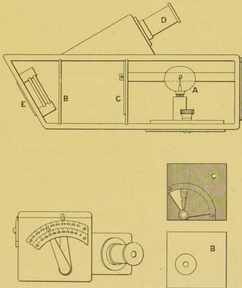
FIG. 168.—DOW AND MACKINNEY'S LUMETER.
