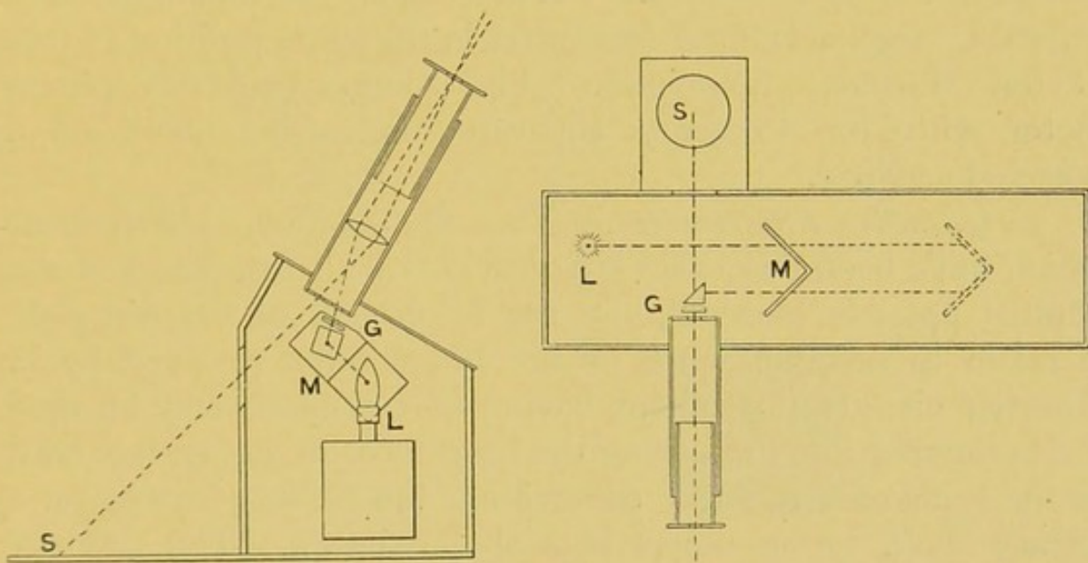
FIG. 167.—THE MARTENS PHOTOMETER. DIAGRAMMATIC PLAN, END VIEW.
