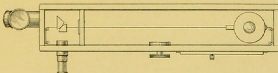
FIG. 163.—THE SHARP AND MILLAR PHOTOMETER.
