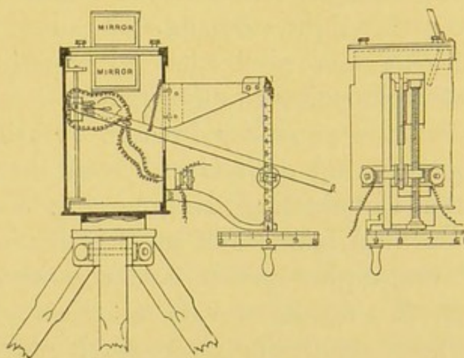
FIG. 135.—PREECE AND TROTTER ILLUMINATION PHOTOMETER.
