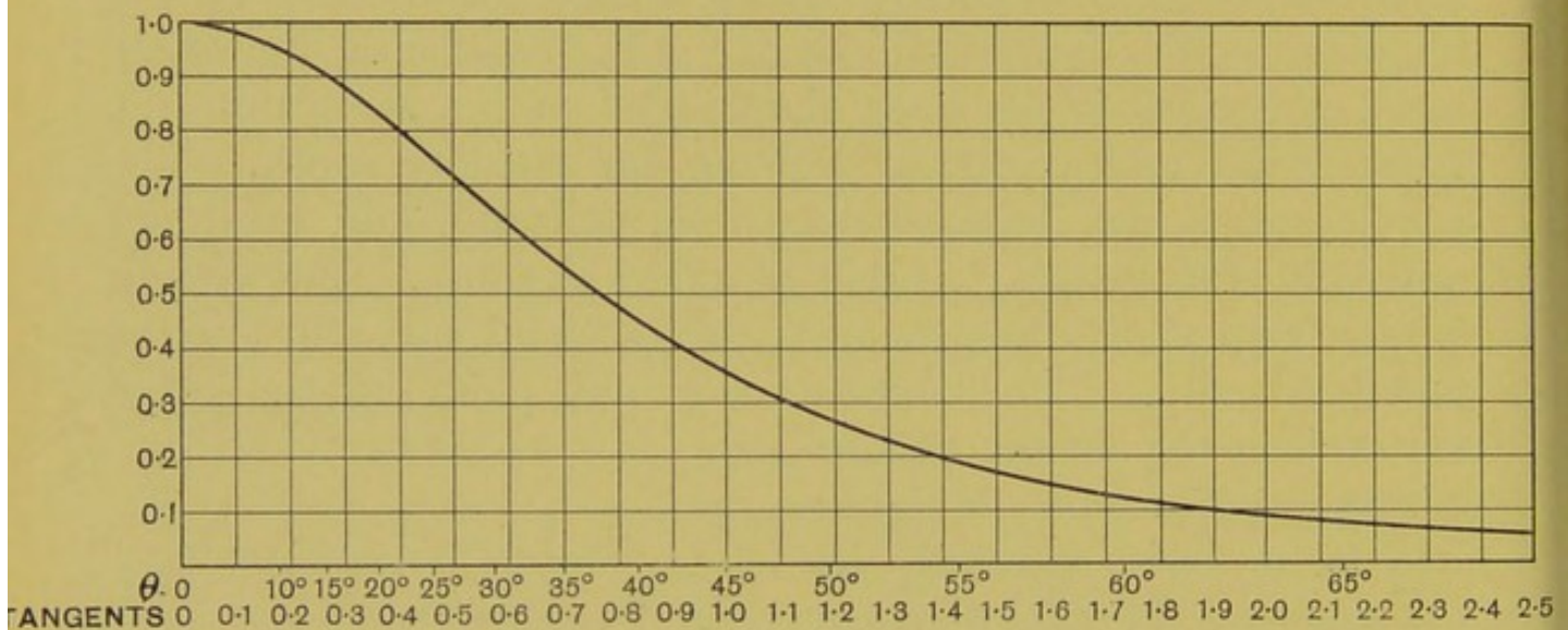
FIG. 9.—CURVE OF COSINES CUBED.
