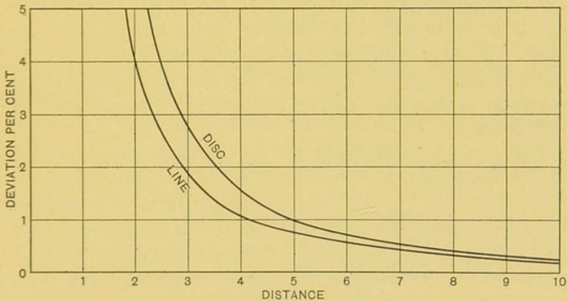
FIG. 90.—DEVIATION FROM THE LAW OF INVERSE SQUARES.
