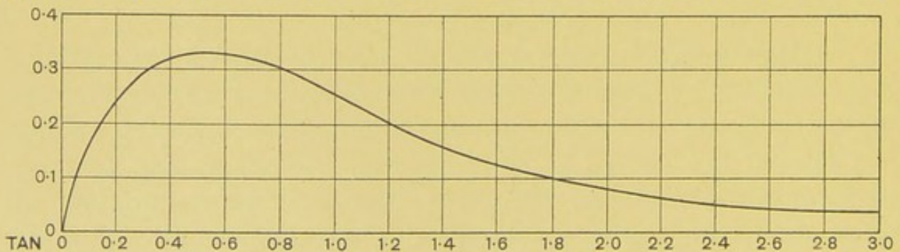
FIG. 16.—DISTRIBUTION OF ILLUMINATION FROM A VERTICAL FILAMENT.
