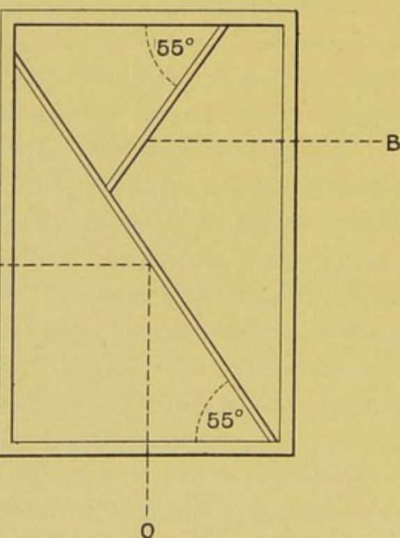
FIG. 76.—THE PERFORATED SCREEN PHOTOMETER.
