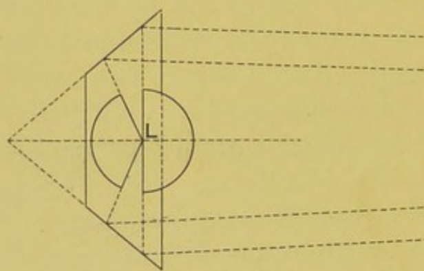
FIG. 115.—BLONDEL'S DIFFUSING CONE LUMENMETER.
