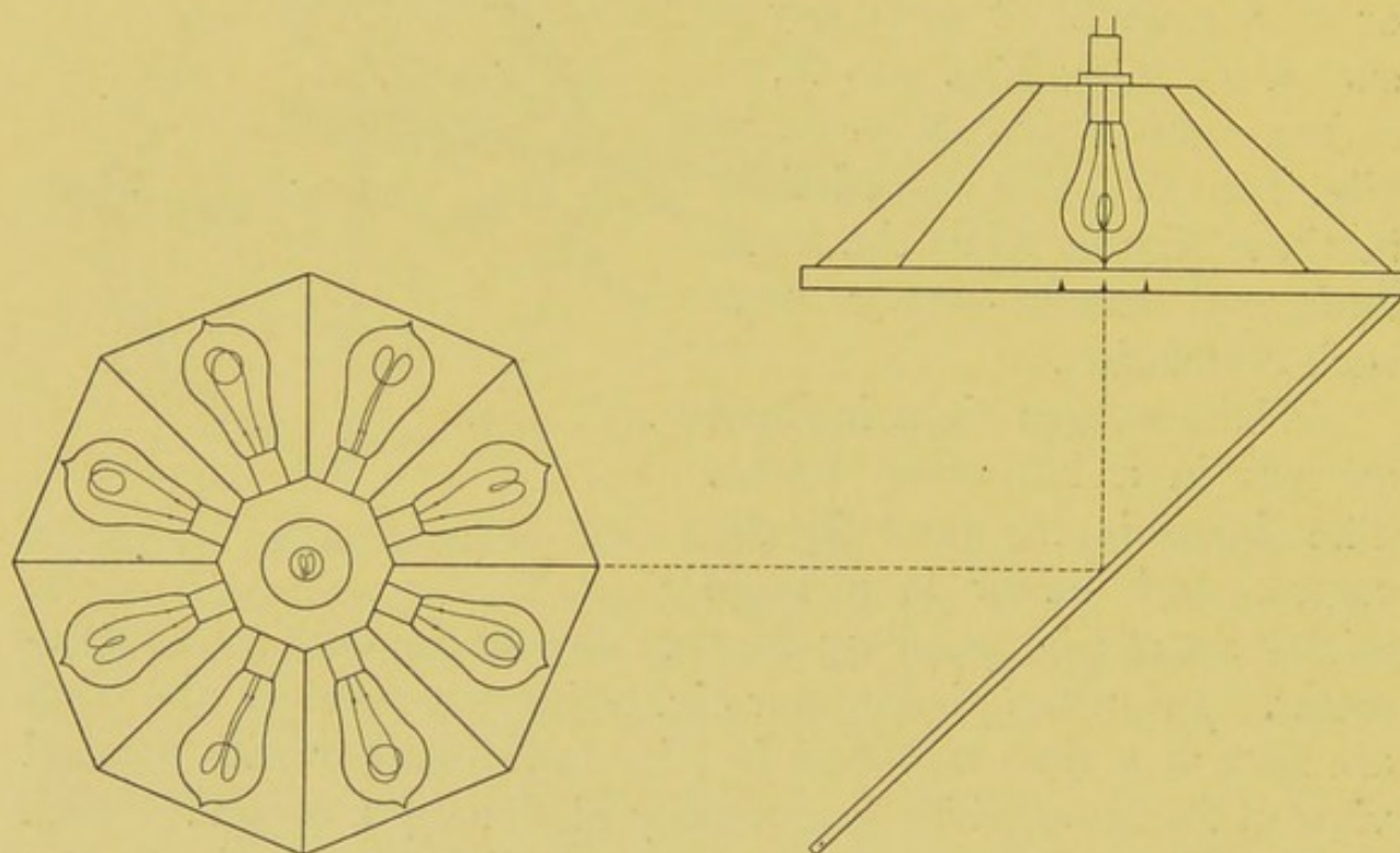
FIG. 101.—WILD'S MIRRORS FOR MEAN HORIZONTAL CANDLE-POWER.
