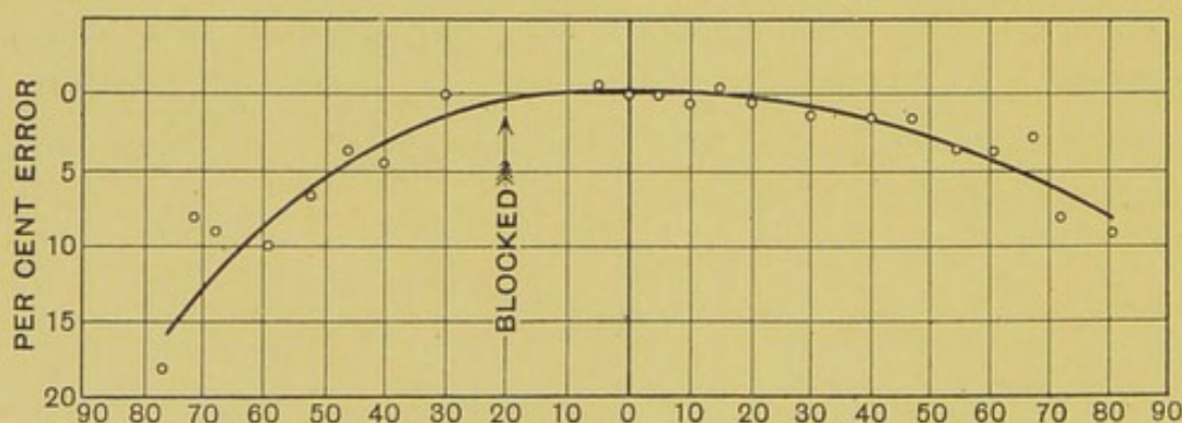
FIG. 150.—GOOD SCREEN IN WORST POSITION.
