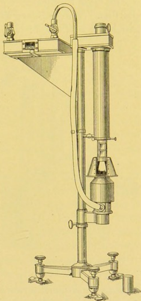
FIG. 1.—THE VERNON HARCOURT PENTANE 10-CANDLE LAMP.
