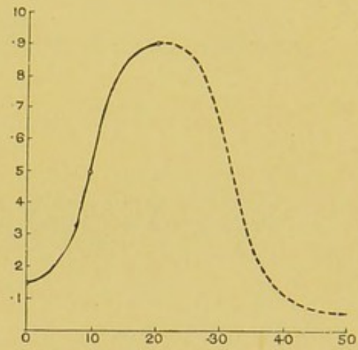
FIG. 175.—MAXIMUM 0.9 FOOT-CANDLE.
