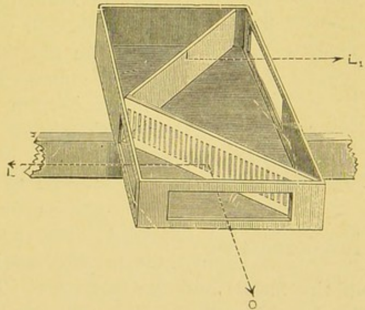
FIG. 81.—GRID PHOTOMETER.
