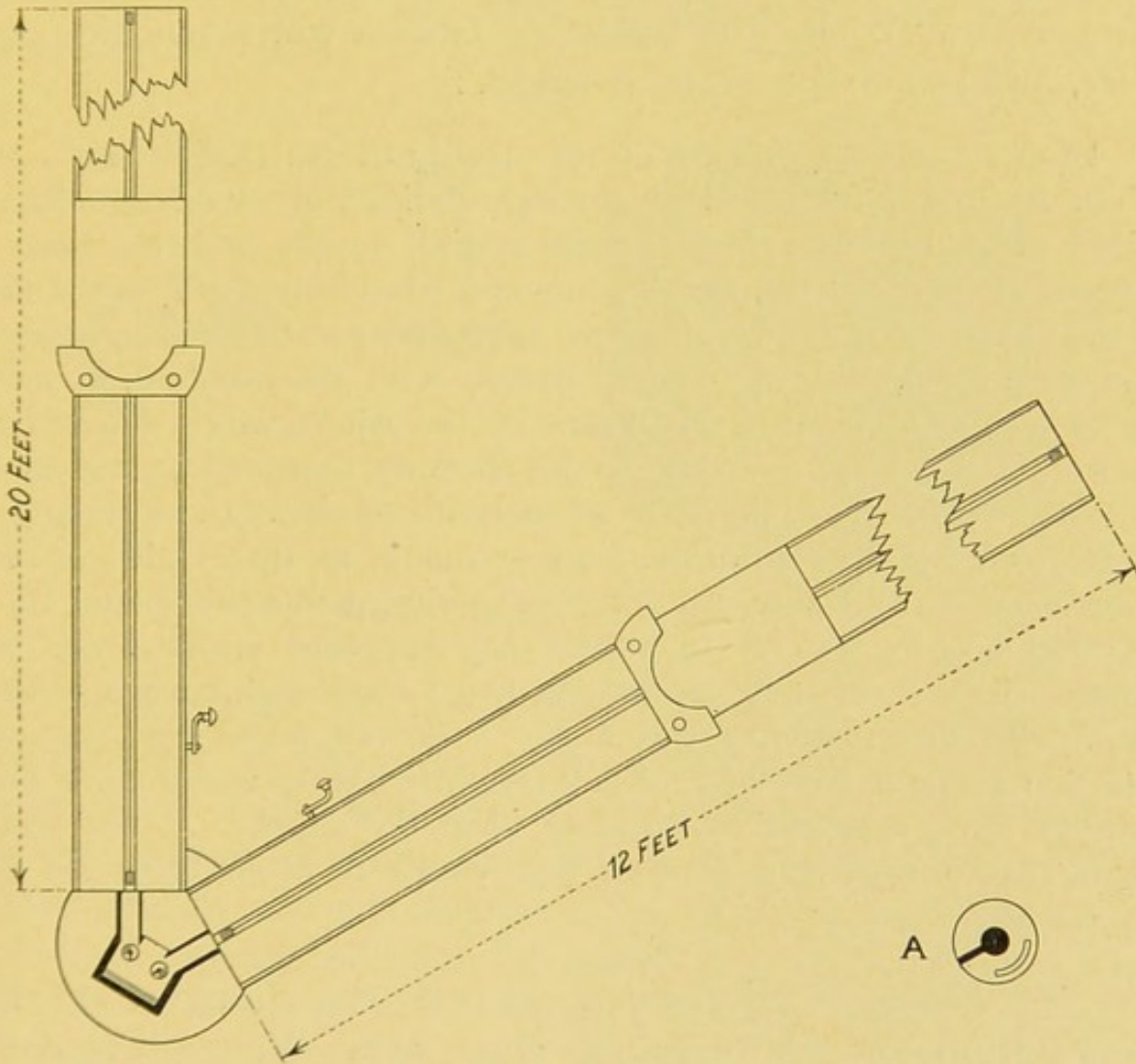
FIG. 56.—RUMFORD'S PHOTOMETER.
