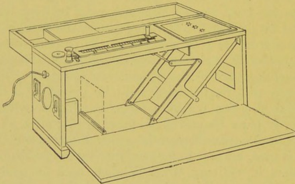
FIG. 137.—SECOND PATTERN TROTTER ILLUMINATION PHOTOMETER, 1895.
