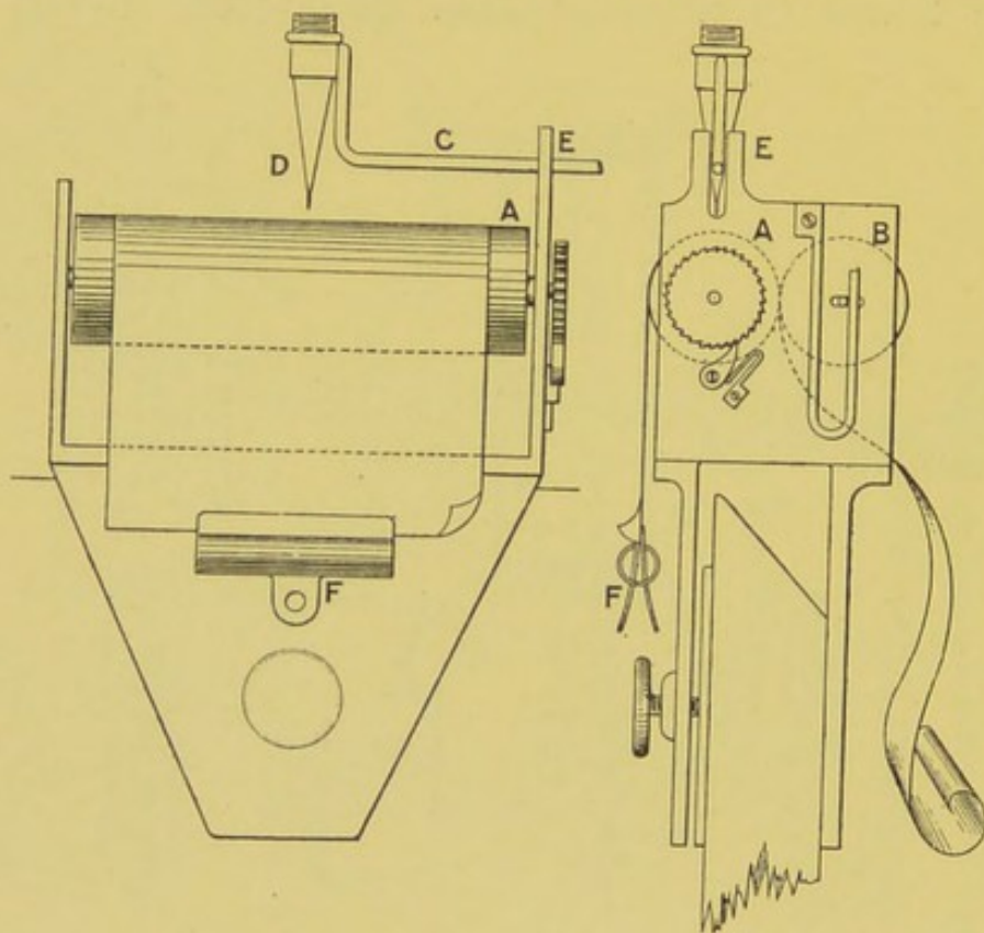
FIG. 95.—OBSERVATION RECORDER.
