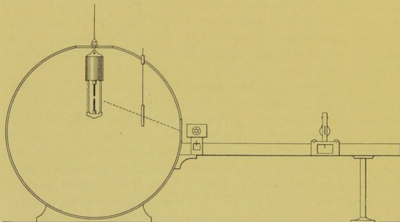
FIG. 120.—THE ULBRICHT GLOBE.
