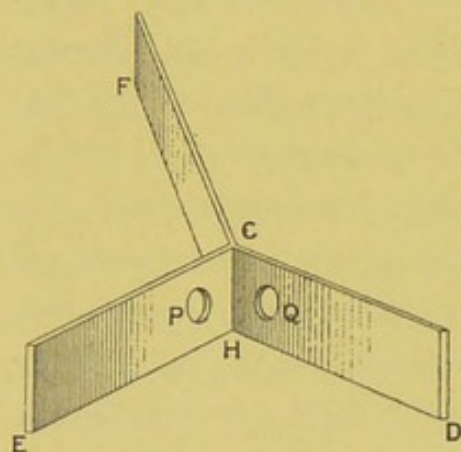
FIG. 55.—BOUGUER'S PHOTOMETER.
