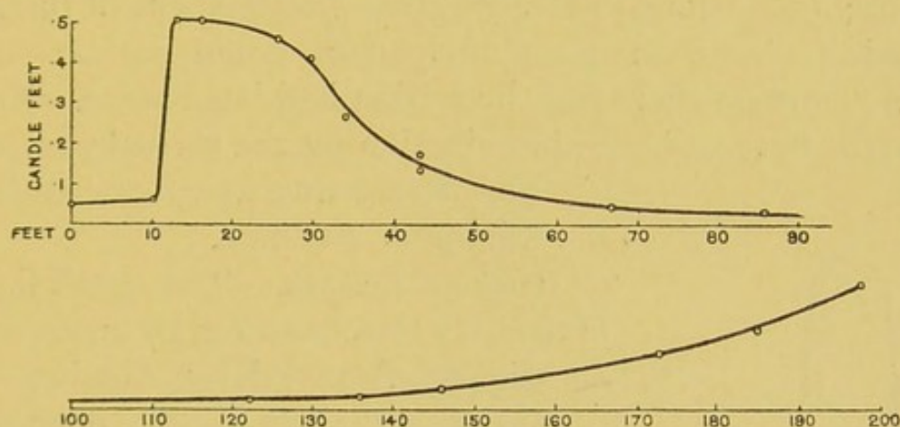
FIG. 172.—DISTRIBUTION OF ILLUMINATION AT CANNON STREET STATION (1872).
