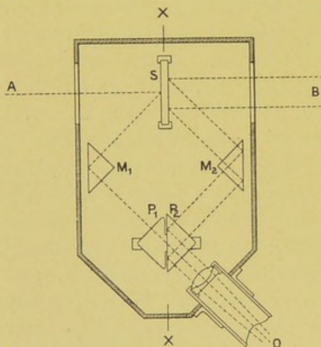
FIG. 73.—LUMMER-BRODHUN PHOTOMETER.
