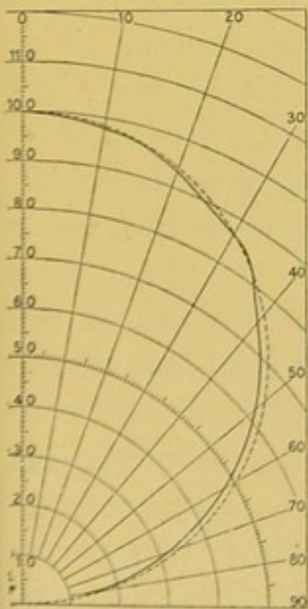
FIG. 165.—SHARP AND MILLAR TEST-PLATE ANGLE ERRORS.
