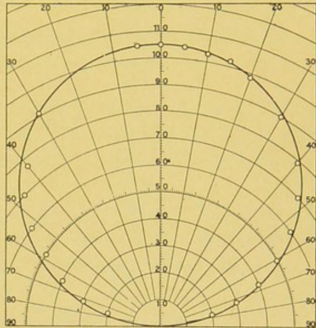
FIG. 149.—GOOD SCREEN IN WORST POSITION.
