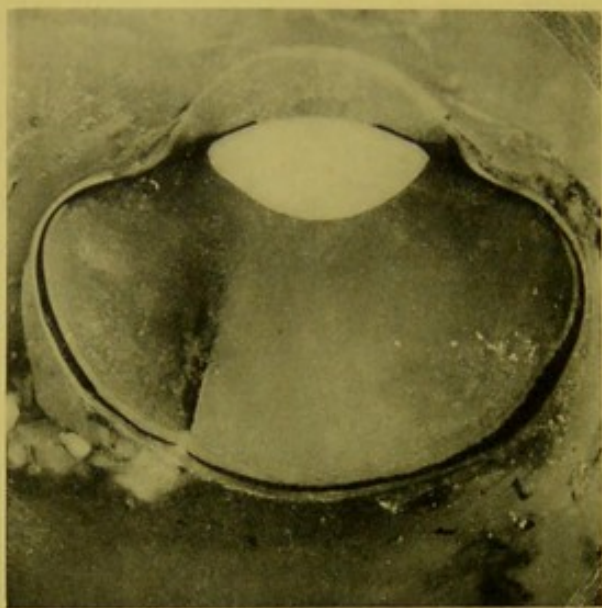
Muskel- ruhe (Curare)
