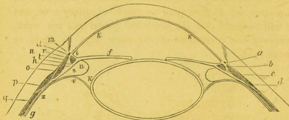
Fig. 30. Magnified section of the human eye, from Hueck. a , Canal of Schlemm. b , Anterior canal of Fontana. c , Middle canal of Fontana. d , Posterior canal of Fontana. f , Iris. g , Posterior portion of ciliary body. h , Anterior portion of ciliary body. i , External margin of iris. k , Coat of Descemet. m , Ligamentum pectinatum iridis. n , o , Anterior junction of ciliary body with the sclerotica. p , q , Posterior junction. r , Orbiculus ciliaris. s , Ciliary process connected at t with the uvea. u , Fimbriated portion of ciliary process. v , Posterior wall of the canal of Petit. z , Junction of the hyaloid membrane with the ciliary zone.
