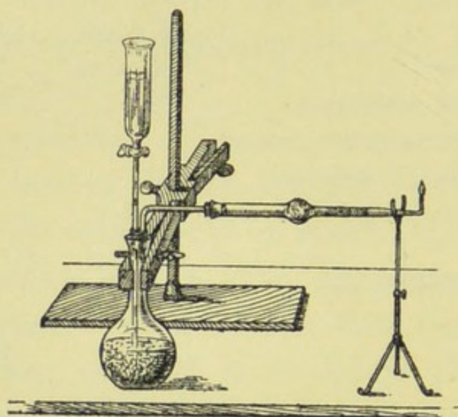
ANALYTICAL APPARATUS.
