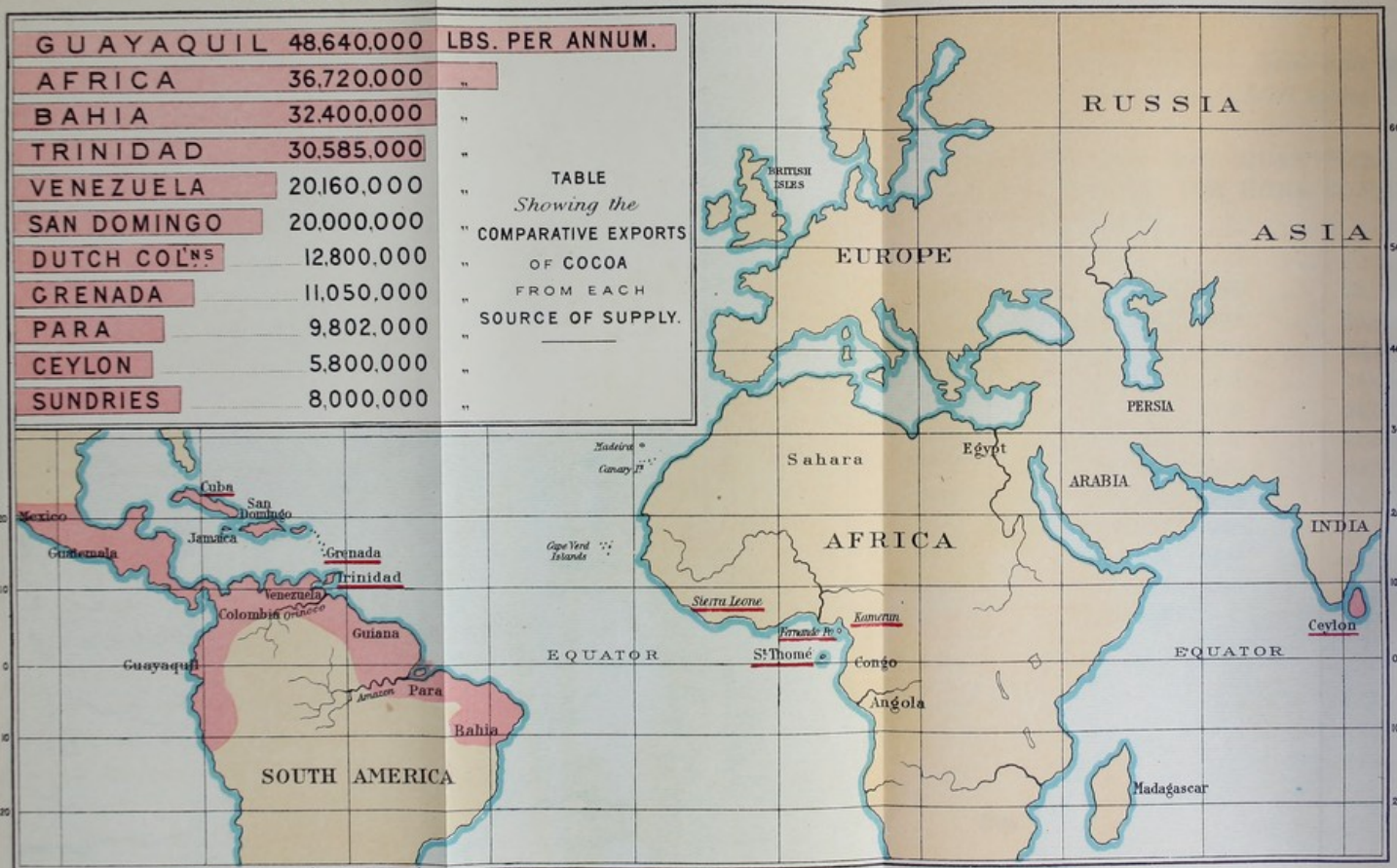
CHART SHOWING THE POSITIONS OF THE PRINCIPAL COCOA PLANTATIONS OF THE WORLD.
